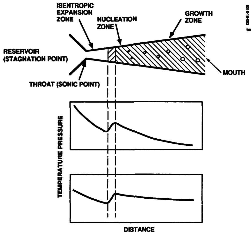
Figure 2. Pressure and temperature distributions in gas flow through a supersonic nozzle with condensation. According to Oswatitsch 3 nucleation takes place only within a narrow zone, while cluster growth continues along much of the nozzle.
