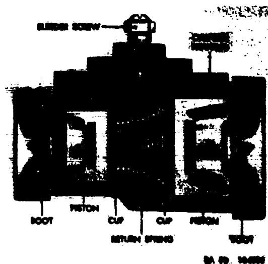
Figure 520. Stepped wheel cylinder—cross sectional view.
