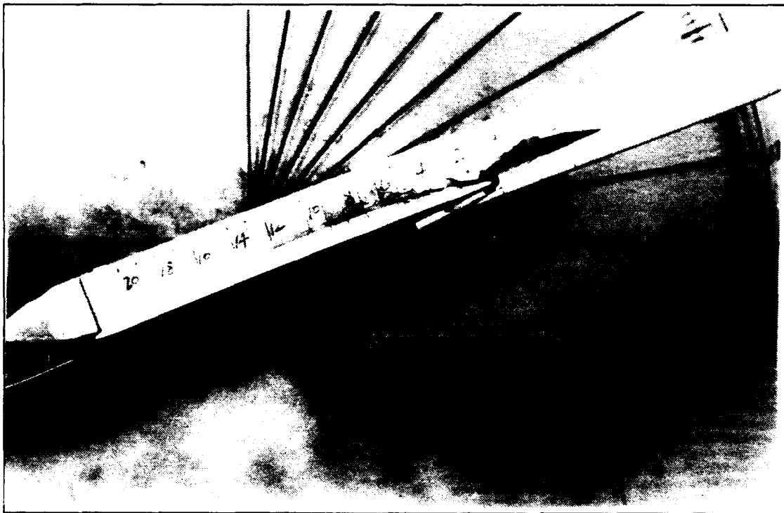
Figure 78. Wing Root Vortex Flow, \alpha=20^\circ , K=-0.16 , \delta_a=\pm 5^\circ , K_c=10.4
