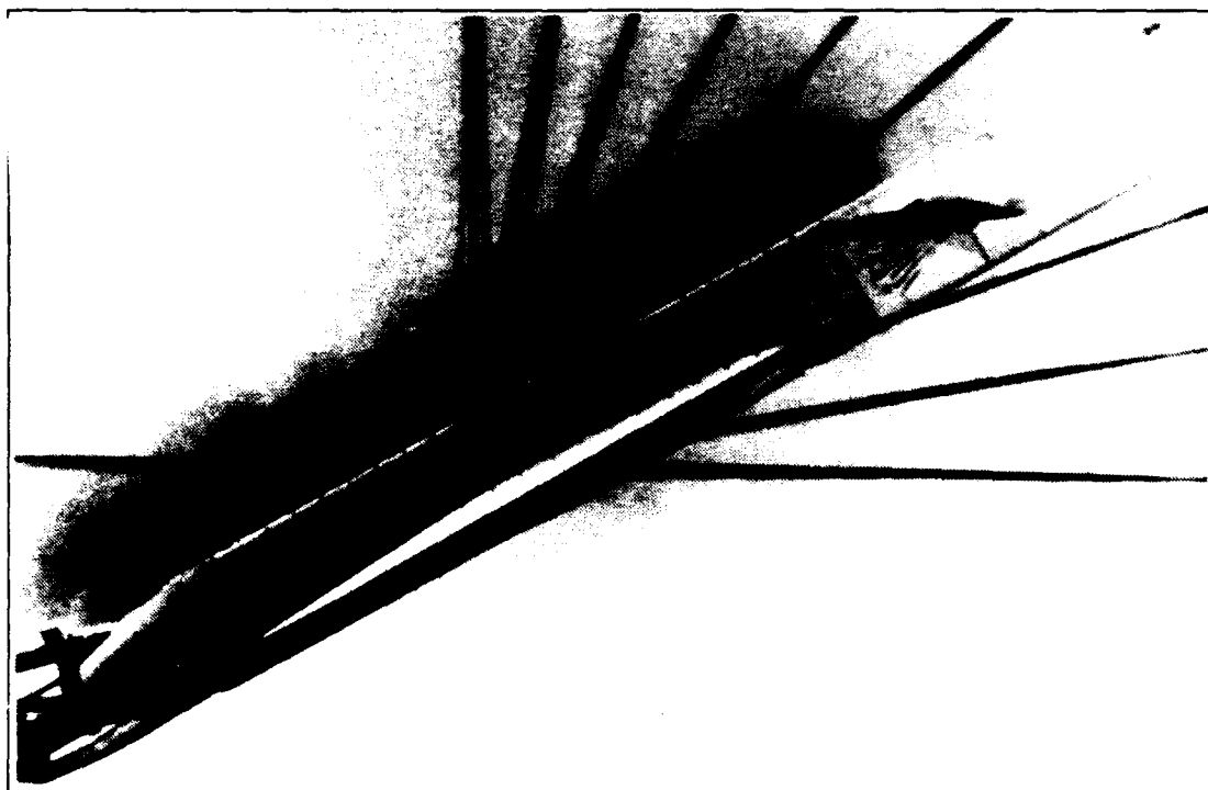
Figure 40. Wing Root Vortex Flow, Static Case, \alpha=30^\circ , \delta=-20^\circ
