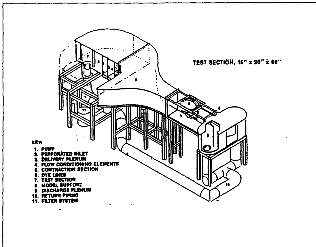
Figure 3. Water Tunnel Facility at NPS
