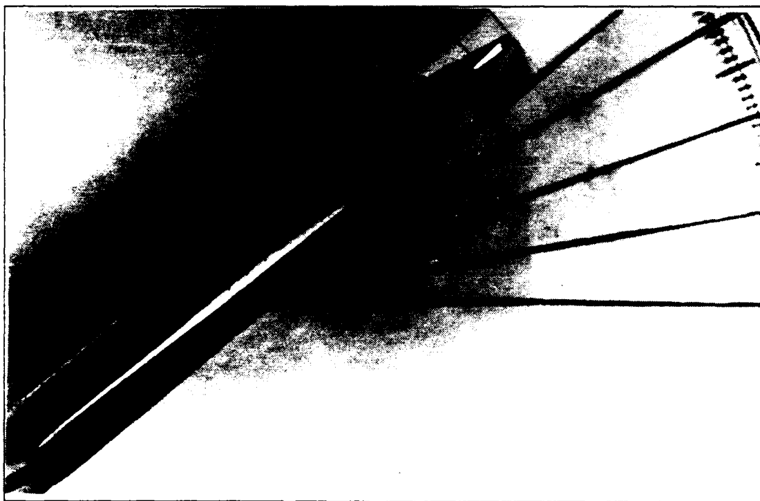
Figure 48. Wing Root Vortex Flow, \alpha=40^\circ , K=0 , \delta_a=+/-5^\circ , K_c=10.4
