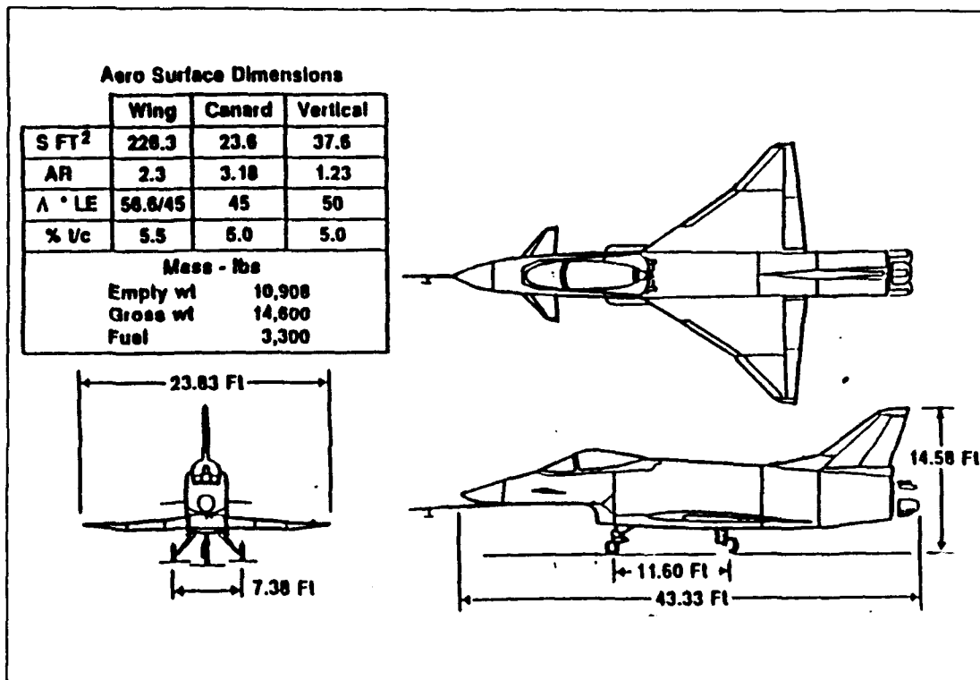
Figure 2. X-31A Aircraft Configuration
