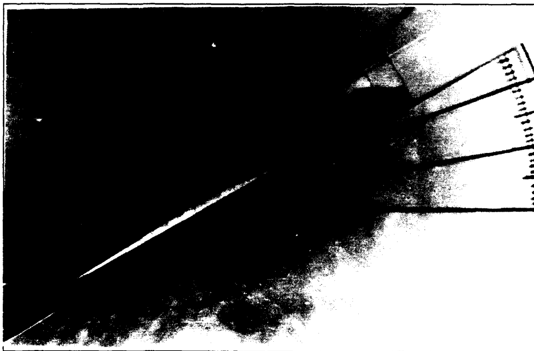
Figure 52. Wing Root Vortex Flow, \alpha=30^\circ , K=0 , \delta_s=+/-25^\circ , K_c=10.4
