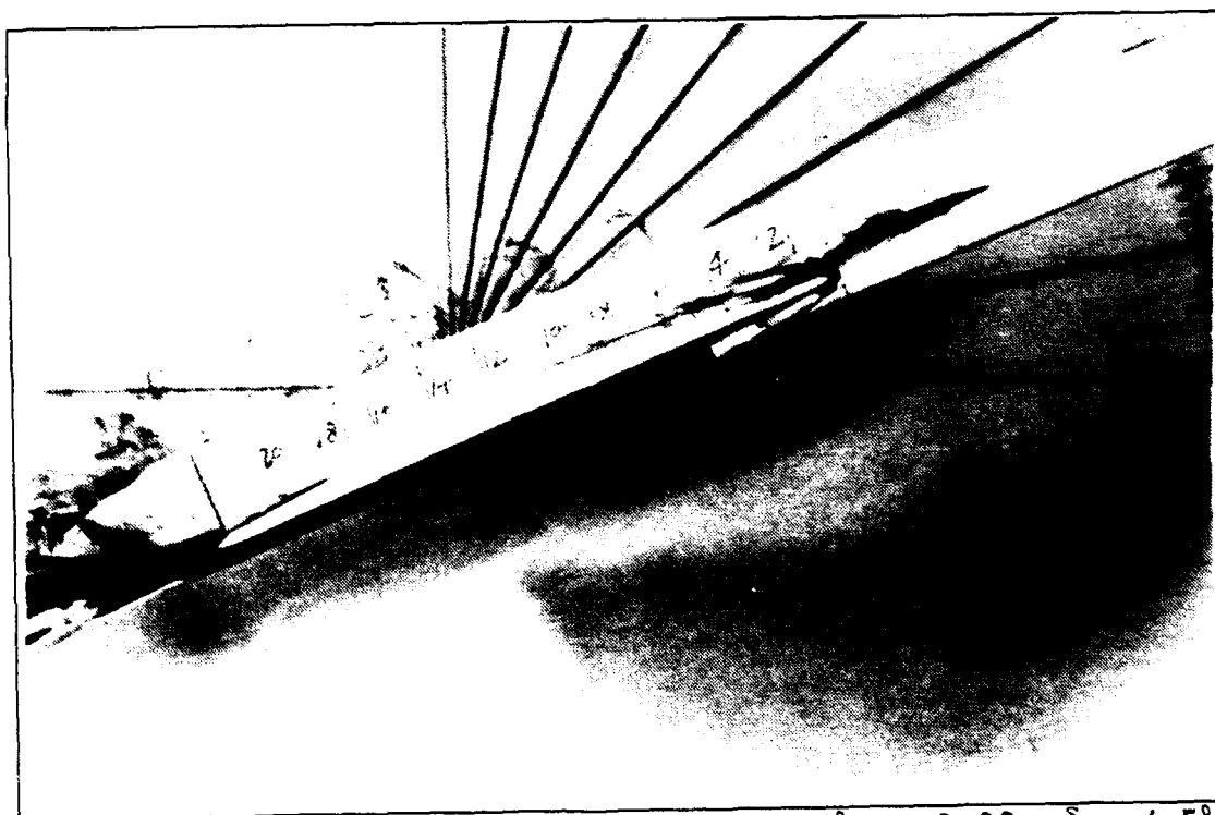
Figure 64. Wing Root Vortex Flow, \alpha=20^\circ , K=0.08 , \delta_a=+/-5^\circ , K_c=1.7
