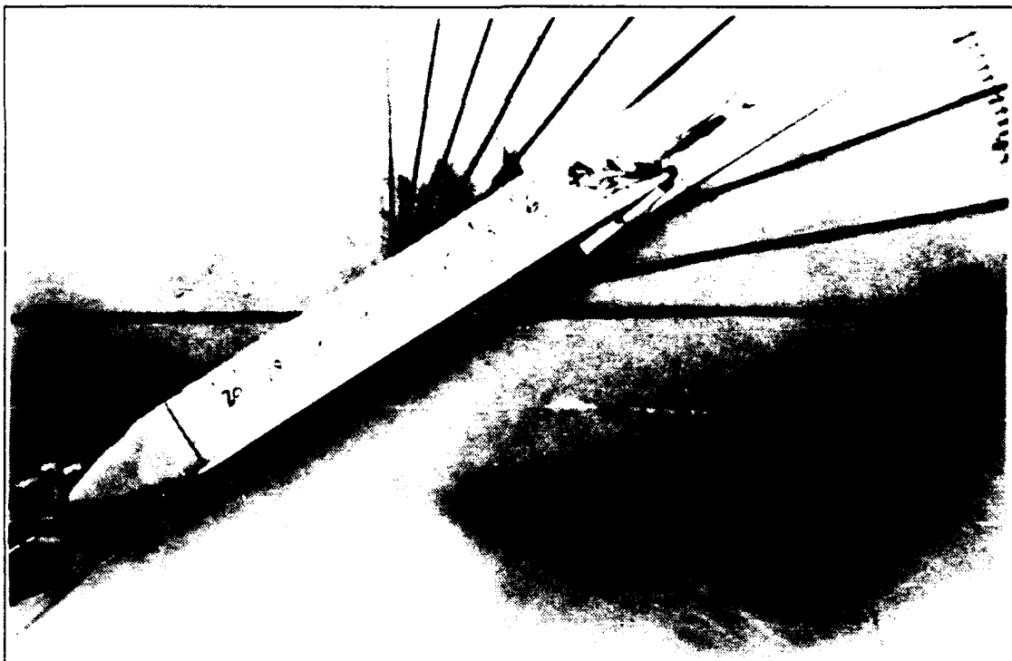
Figure 69. Wing Root Vortex Flow, \alpha=30^\circ , K=-0.08 , \delta_a=+/-5^\circ , K_c=1.7
