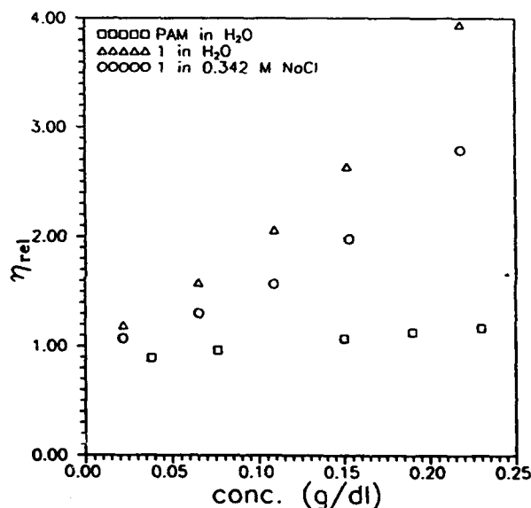
Figure 4. Relative viscosity vs concentration for copolymer 1 in H 2 O ( \Delta ) and in NaCl (O) and for homopolyacrylamide in H 2 O ( \square ).
