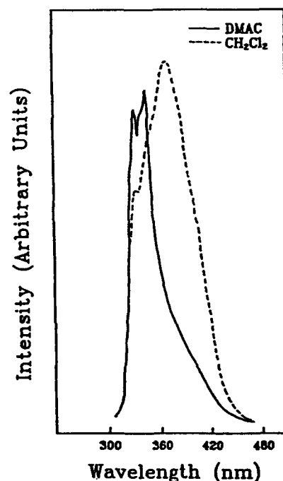
Fig. 2. Steady state fluorescence spectra of NAEA(59-6)-VP in dimethylacetamide (DMAC) and methylene chloride (CH 2 Cl 2 ).
