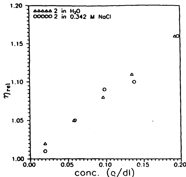
Figure 2. Relative viscosity vs concentration for copolymer 2 in H 2 O ( \Delta ) and in NaCl (O).
