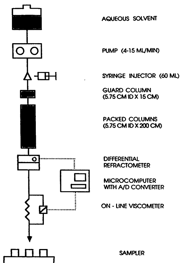
Figure 1 Preparative GPC system.
