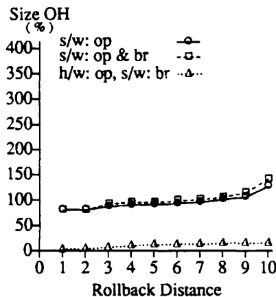
Figure 15: PUZZLE, Program Size Overhead.
