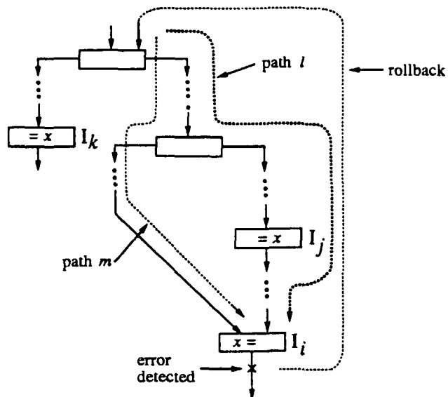
Figure 5: read Buffer Resolution of Branch Hazards
