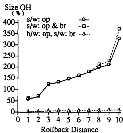
Figure 7: QUEEN, Program Size Overhead.
