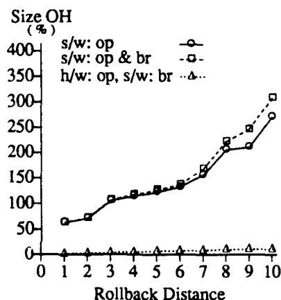
Figure 11: QSORT, Program Size Overhead.
