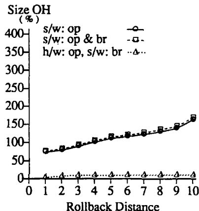
Figure 13: CMP, Program Size Overhead.
