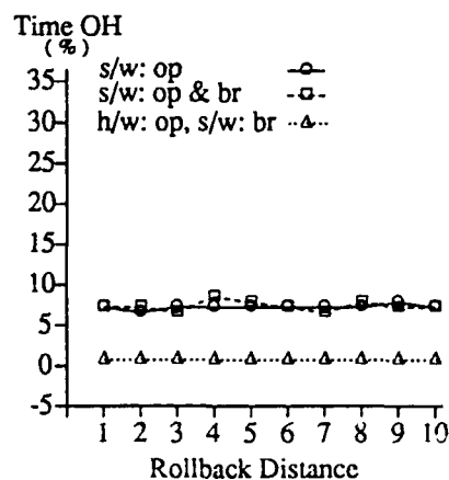
Figure 8: WC, Runtime Overhead.
