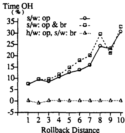
Figure 10: QSORT, Runtime Overhead.
