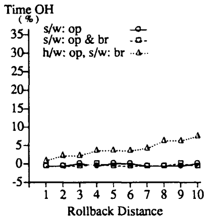
Figure 14: PUZZLE, Runtime Overhead.
