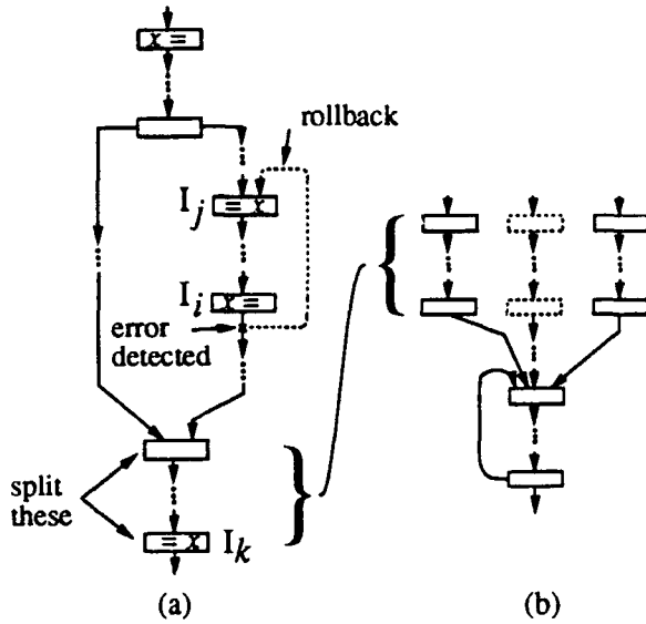
Figure 2: Node Splitting.
