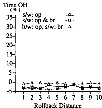
Figure 12: CMP, Runtime Overhead.
