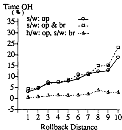
Figure 6: QUEEN, Runtime Overhead.
