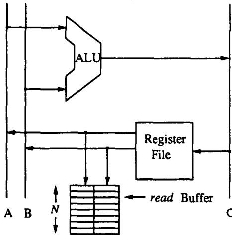
Figure 4: read Buffer.
