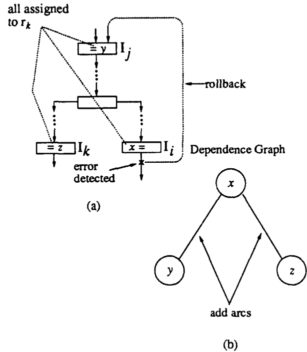
Figure 3: Machine Register Hazards.
