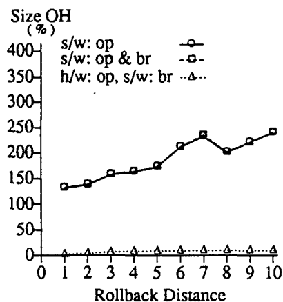
Figure 9: WC, Program Size Overhead.
