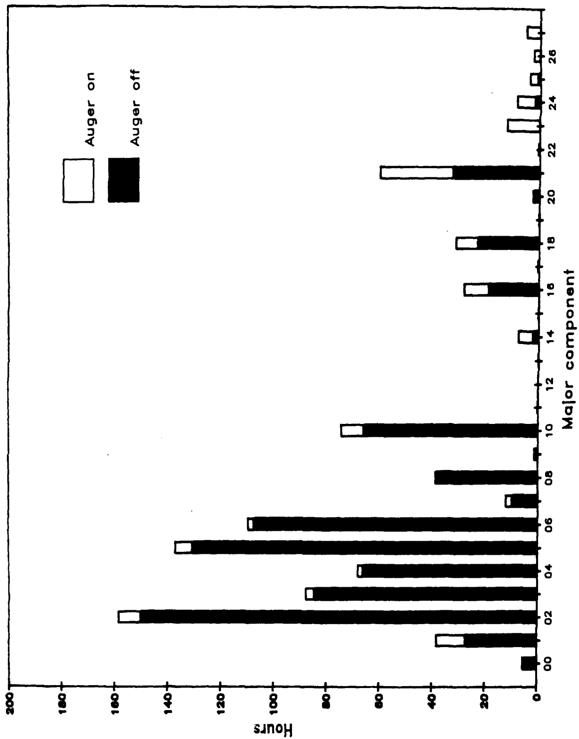
Figure 16. Component Unscheduled Maintenance Times.
