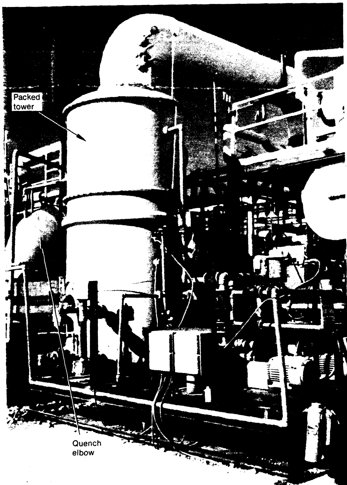
Figure 10. View of Skid Mounted Packed Tower.
