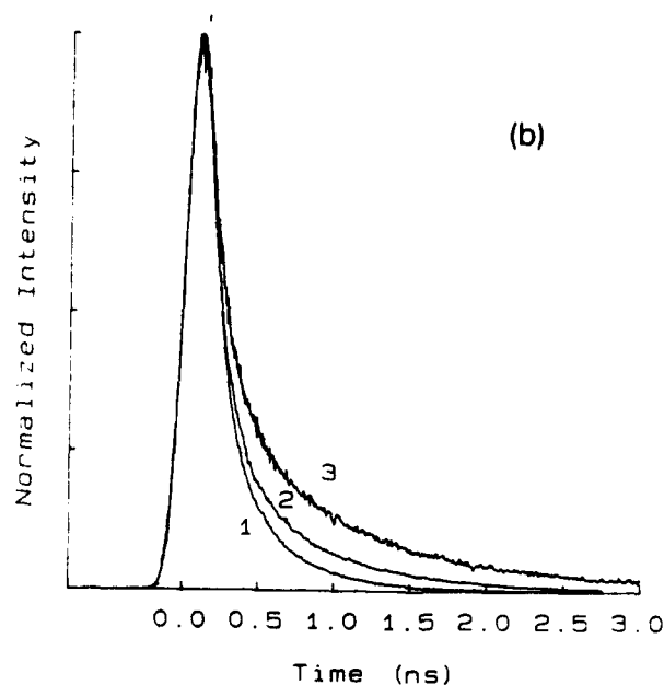
Fig. 4. (a) Fringe spacing dependence of the TG signal probing excited-state energy transport in disodium fluorescein in ethanol, for \theta/2 = 8^\circ and 22^\circ (excitation wavelength 266 nm) [8]. For the smaller angle, the signal is dominated by acoustic effects (note: time scale is different for \theta/2 = 8^\circ ). At \theta/2 = 22^\circ , the acoustic-signal contribution damps out due to acoustic attenuation. (b) Fringe spacing dependence of the TG signal probing carrier density diffusion in GaAs. N_{eh} = 2 \times 10^{19} photocarriers/cm 3 . The measured ambipolar diffusion constant is in good agreement with the known value for high purity GaAs ( D_{ex} \approx 8 cm 2 /sec). Curve 1: \theta = 4.9^\circ , curve 2: \theta = 3^\circ , curve 3: \theta = 1.1^\circ (see ref. [117]).
