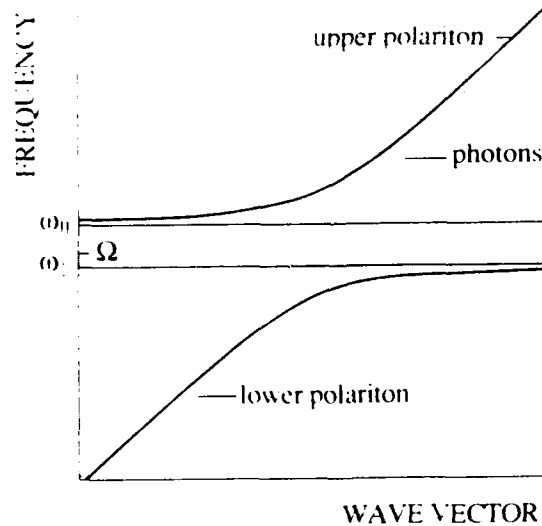
Fig. 6 Typical polariton dispersion curves in the optical region for an atomic crystal (thick solid curves). The diagonal line represents the pure photon dispersion curve ( \omega_k = kc ). The shaded region between the transverse ( \omega_- ) and longitudinal ( \omega_+ ) crystal exciton frequencies is the stopgap, where no polariton modes exist. \Omega indicates the atomic transition frequency. For a crystal of two-level molecules, the stopgap position depends on the direction of propagation (see text).
