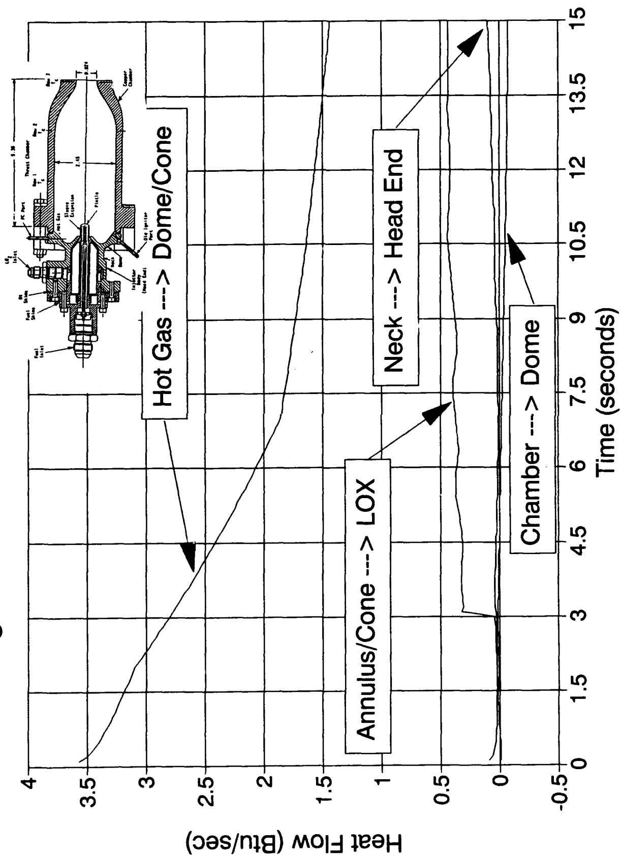
Figure 4-11. Heat Flows - Run HA2A-3999
