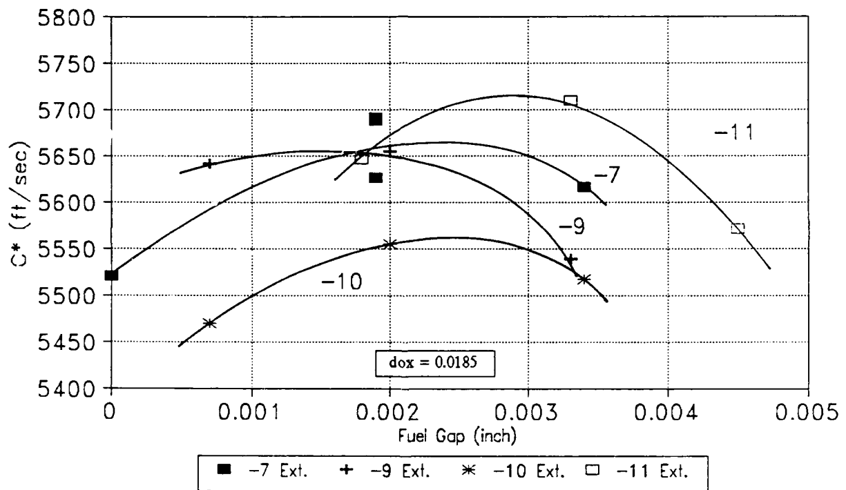
Figure 5-9. C^* verses fuel gap for 200 lbf elements
