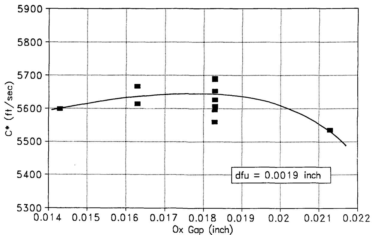
Figure 5-7. -7 C^* verses oxidizer gap
