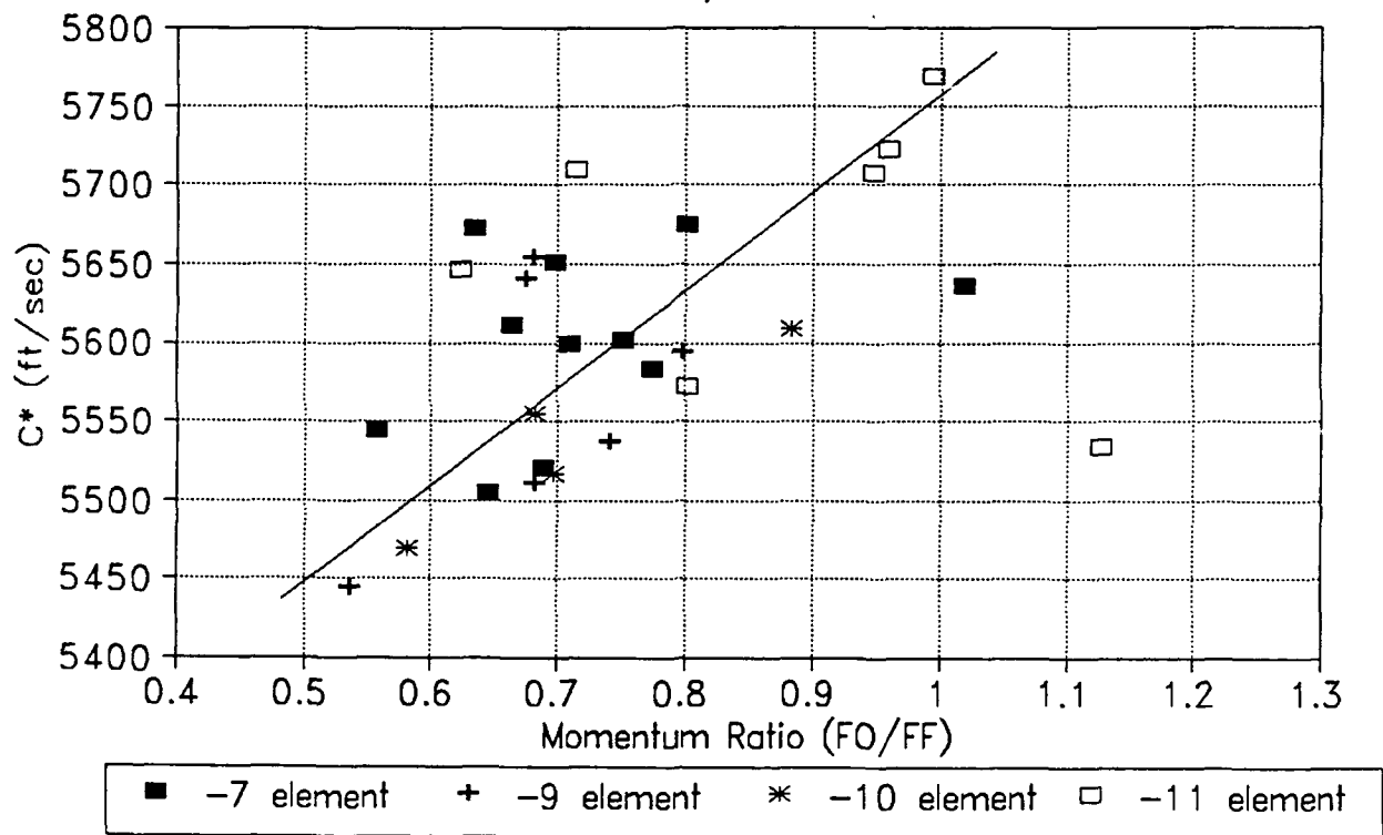
Figure 5-12. C^* performance verses Momentum Ratio
