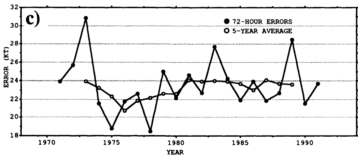
Figure 5-4. Annual mean intensity forecast errors (kt) and 5-year running mean for a) 24-hours, b) 48-hours and c) 72-hours in the Northwest Pacific Ocean.
