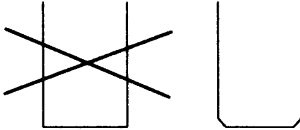
Figure 3a. Avoid sharp corners to avoid areas of stagnation, to facilitate cleaning, and to facilitate application of coatings.
