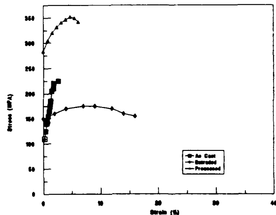
Figure 11. Comparison of the stress vs strain behavior of as-cast, extruded and as-processed composite (550°C).
