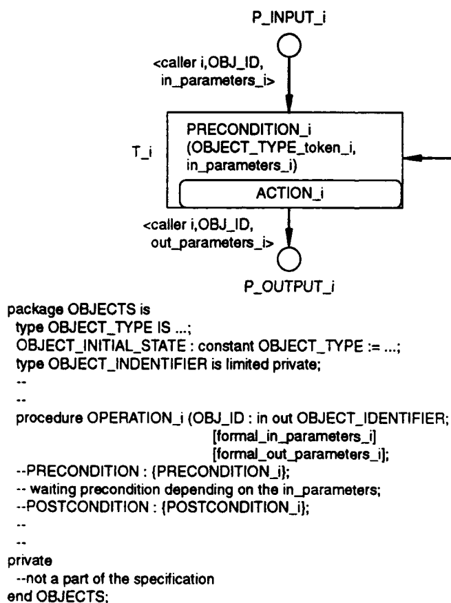
Figure 25. Input Scheme of the Transformation Applicable to TR.2
