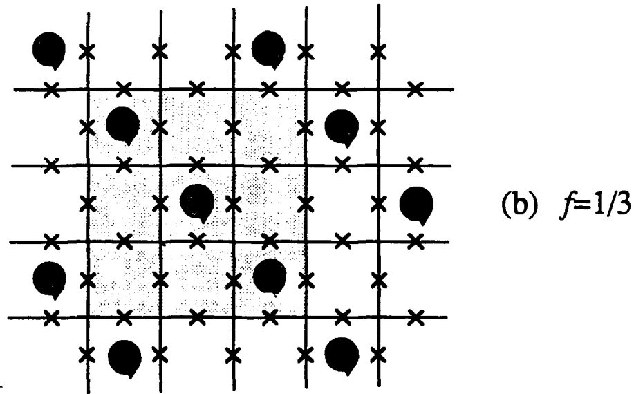
Fig. 1.6. Schematic diagram of a square-lattice array of Josephson junctions in the presence of a commensurate magnetic field, where the average number of flux quanta per unit array cell, f , is (a) 1/2 and (b) 1/3 . The "x"s represent the positions of the junctions and the direction of the applied field is out of the page. The darkened circles with arrows represent the field-induced vortices, and they are arranged in a superlattice which is commensurate with the underlying array lattice. A unit cell of the superlattice is shown shaded in each of the diagrams.
