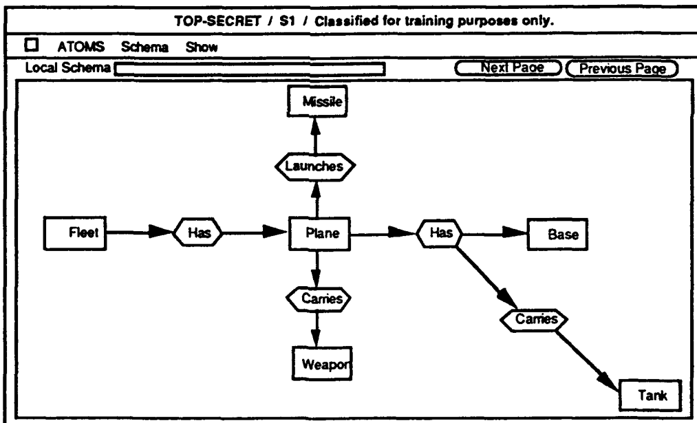
Figure 17. Suggested Improvements for Schema Display
