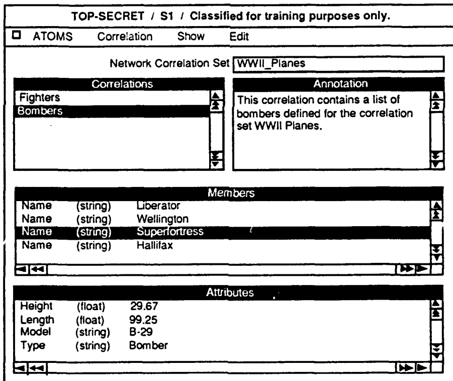
Figure 15. An Example Correlation Set Browser Window in which a user correlates entity and relationship instances.
