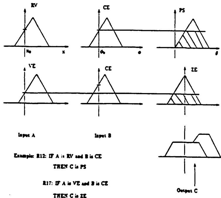
Figure 3. An example of MIN-Centroid procedure.
