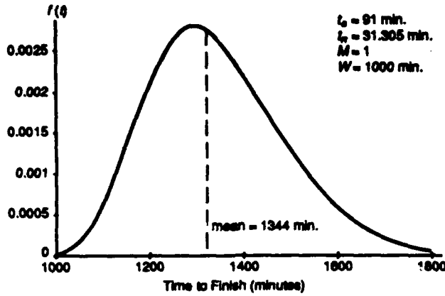
Figure 2: First Passage Time Density for Direct Analysis.
