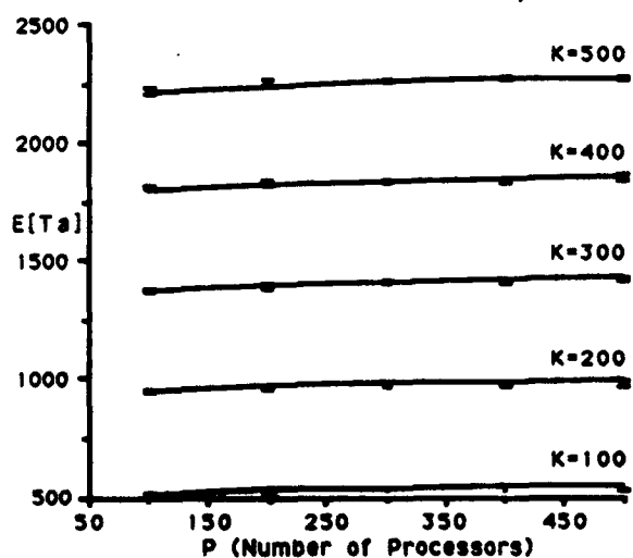
Comparison of E[T_a] Approximation with Simulation (Confidence 98%) ( \mu = 1/4 )
