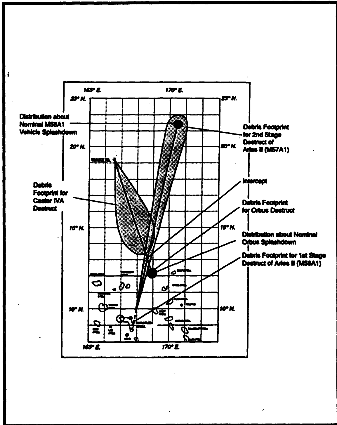
Exhibit 1.13: LEAP-5 Dispersion Area
