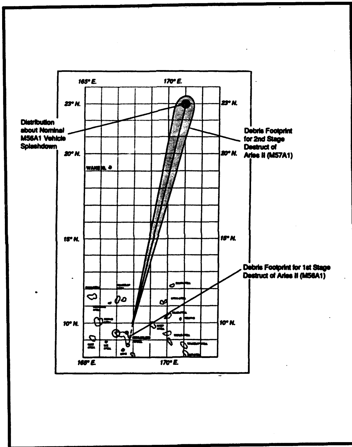
Exhibit 1.11: LEAP-X Dispersion Area
