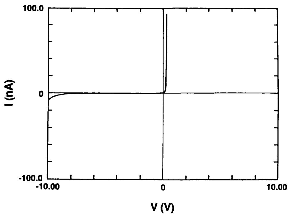
Figure 5. Current-voltage characteristics of Pt/6H-SiC after annealing at 650^{\circ}\text{C} for 20 min. ( 2.0 \times 10^{-3} \text{ cm}^2 contact area).
