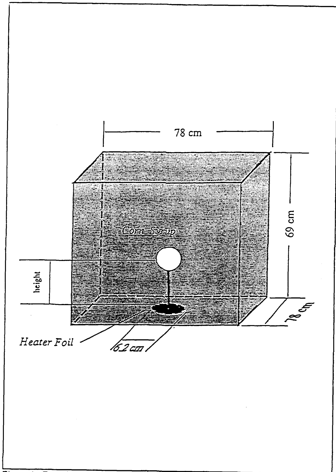
Figure 1. Experimental apparatus.
