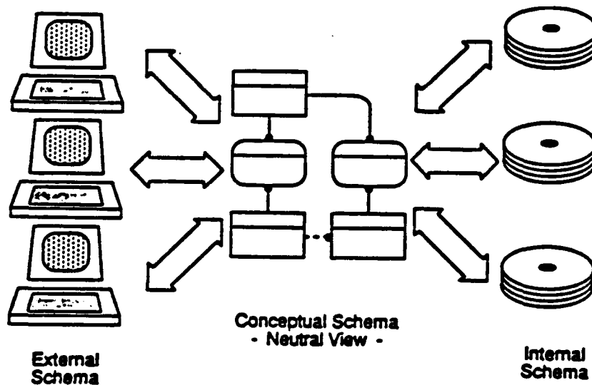
Figure 2-3. Three-Schema Approach
