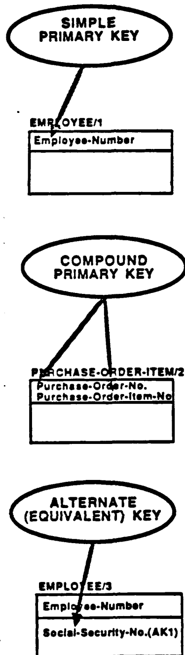
Figure 4-12. Key Forms
