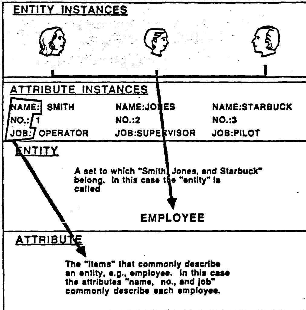
Figure 4-11. Attribute Examples
