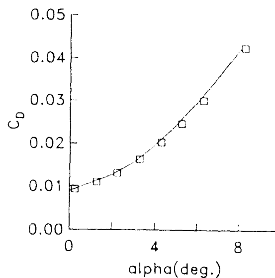
Figure 4-7. High-Speed Civil Transport Navier-Stokes Configuration
