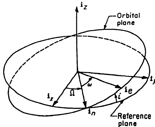
Figure 2.9 Orbital Elements 25
