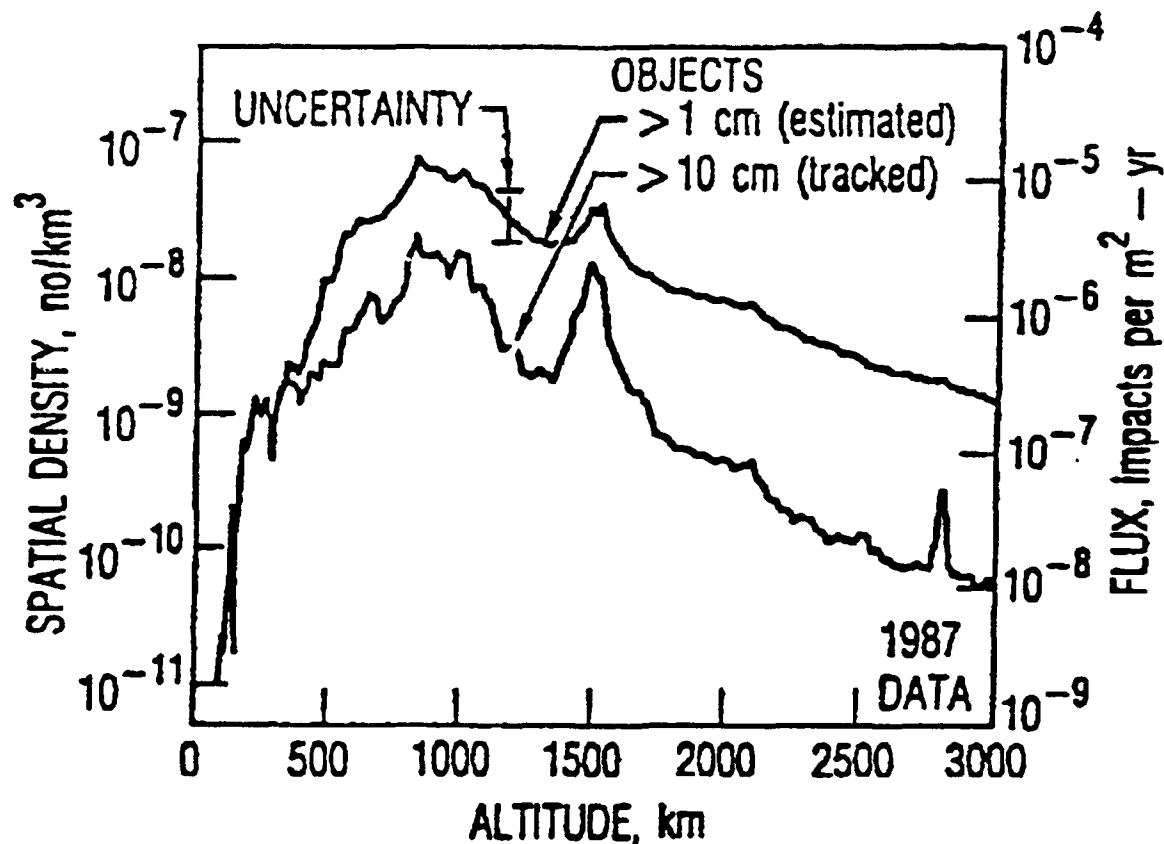
Figure 3.13 Orbital Debris Density vs. Altitude 20
