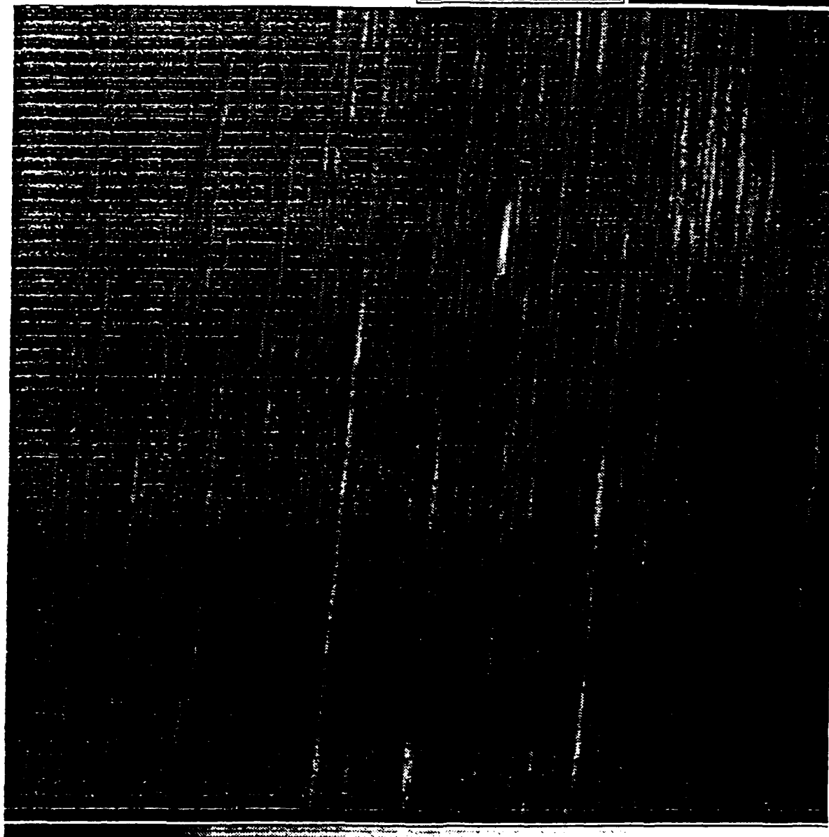
Figure B.6 50 Shifted and Added Video Frames After Background Subtraction of the Same Object as in Figure B.5
