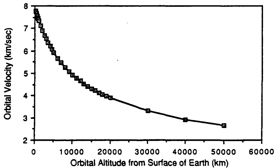
Figure 4.2 Orbital Velocities for Circular Orbits at Various Altitudes
