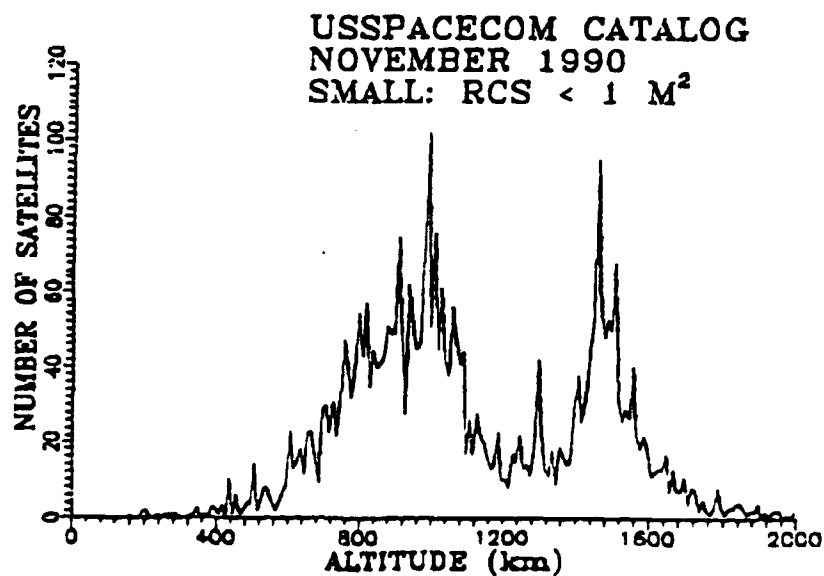
Figure 3.5 Number of Objects Cataloged Less Than 1 Square Meter vs Altitude Size Approximated by Radar Cross Section (RCS)
