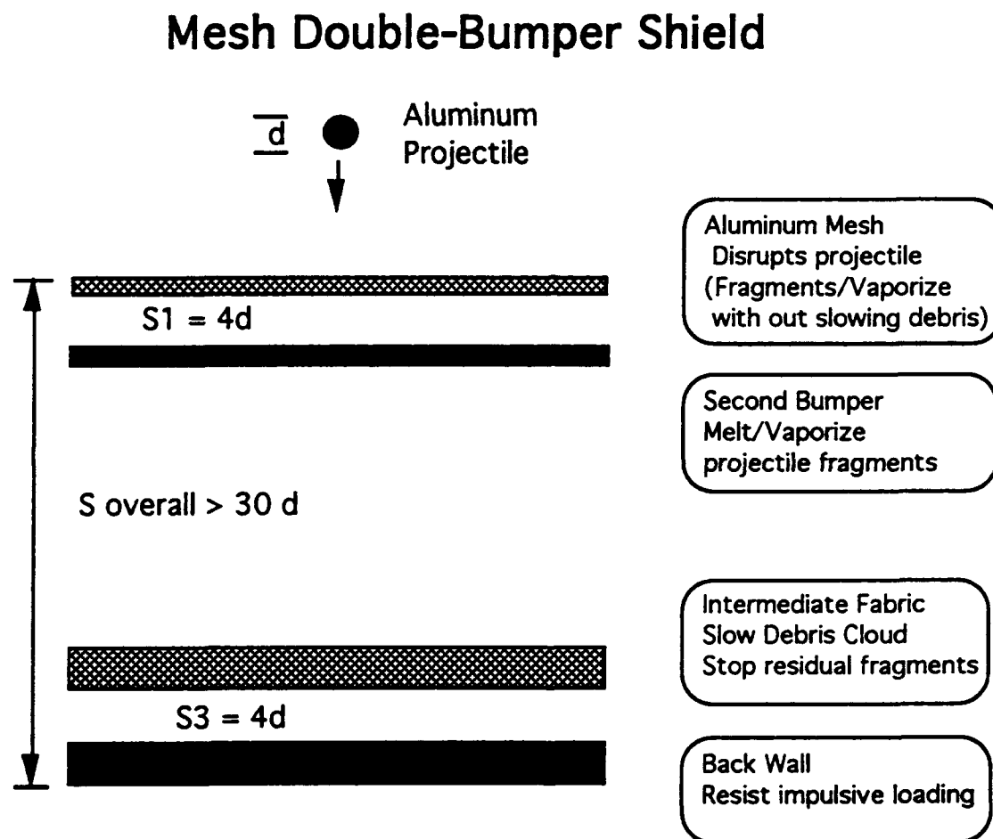
Figure 7.2 Mesh Double Bumper 6
