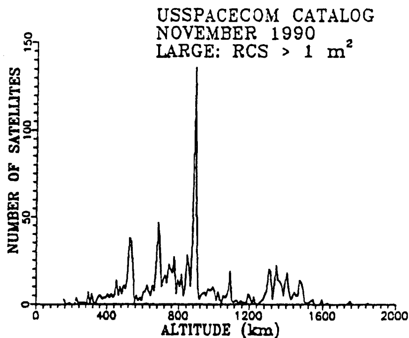
Figure 3.4 Number of Objects Cataloged Greater Than 1 Square Meter vs Altitude Size Approximated by Radar Cross Section (RCS)
