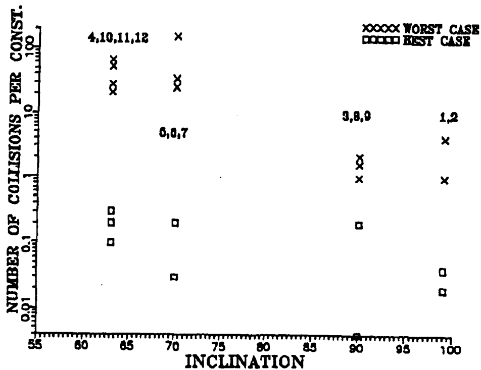
Figures 3.18 and 3.19 Department of Defense Satellite Hazard Analysis for Altitude and Inclination Dependence
