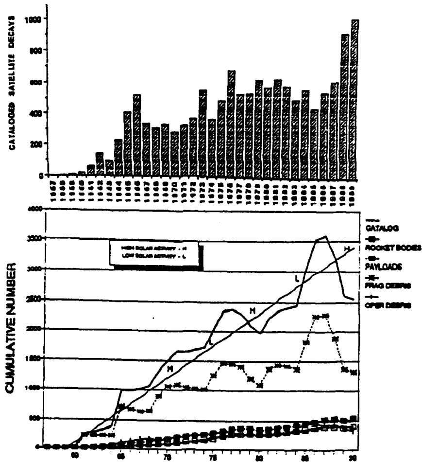
Figure 2.13 a,b,c a) Solar Activity Measured by the Sunspot Number (Bottom line) and F10 Index (Top line), b) The Number of Decaying Cataloged Objects by Year, and c) the Total Number of Low Earth Orbiting Objects below 1000 km Contained in the Satellite Catalog by Year
