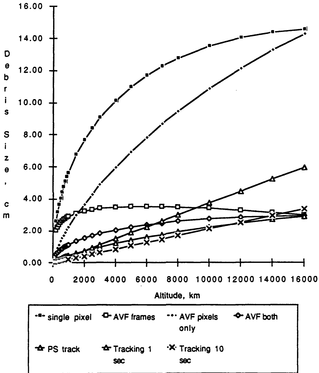
Figure B.17 Minimum Detectable Size for Wright Patterson at Various Altitudes and Various Methods (Signal to Noise Ratio of 5).
