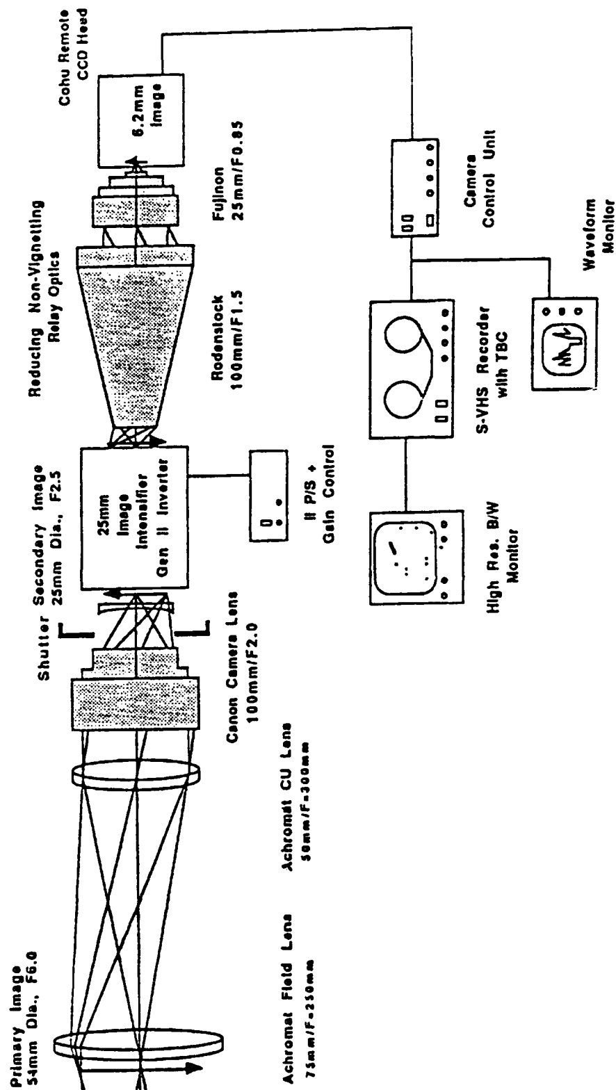
Figure B.2 Receiver Schematic for the Wright Patterson 100-inch Collimator for Debris Detection Efforts
