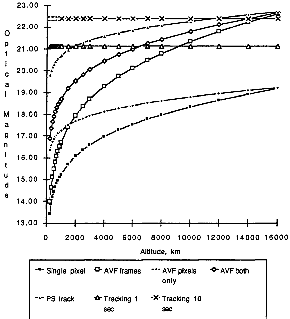
Figure B.15 Faintest Detectable Object Brightness for the Wright Patterson Debris Detection System at Various Altitudes and a Signal to Noise Ratio of 5.
