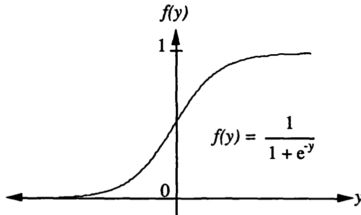
Figure 2.4 Sigmoidal Function
