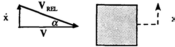
Figure 4.2 Effective Angle-of-Attack
