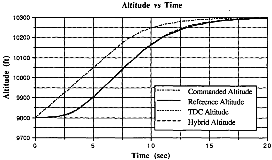
Figure 4.22(a) Altitude trajectories for the reference model, TDC controlled aircraft, and hybrid controlled aircraft after 500 trials.
