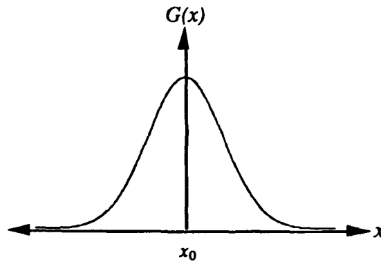
Figure 3.2 Gaussian Function
