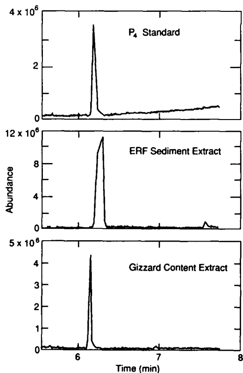
Figure 19. Chromatogram from a GCMS comparing peaks for a white phosphorus standard and extracts of an ERF salt marsh sediment and of the gizzard contents of a pintail duck that died in ERF on 11 September 1990.
