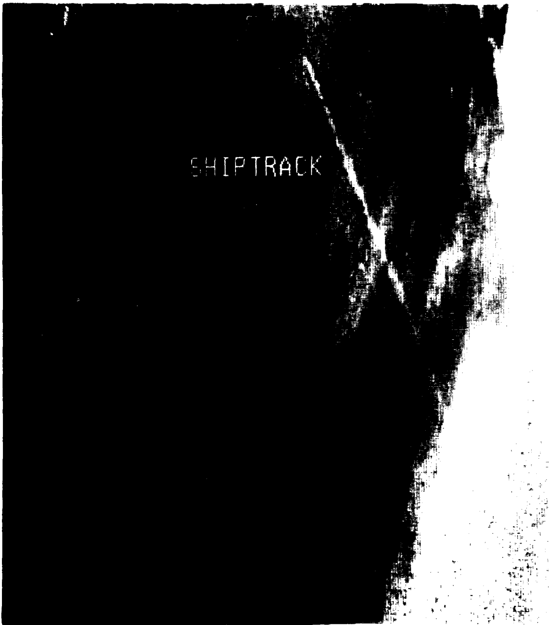
Fig. 18. Subtropic Shiptrack Case 10: 03 July 1987 1626 UTC
