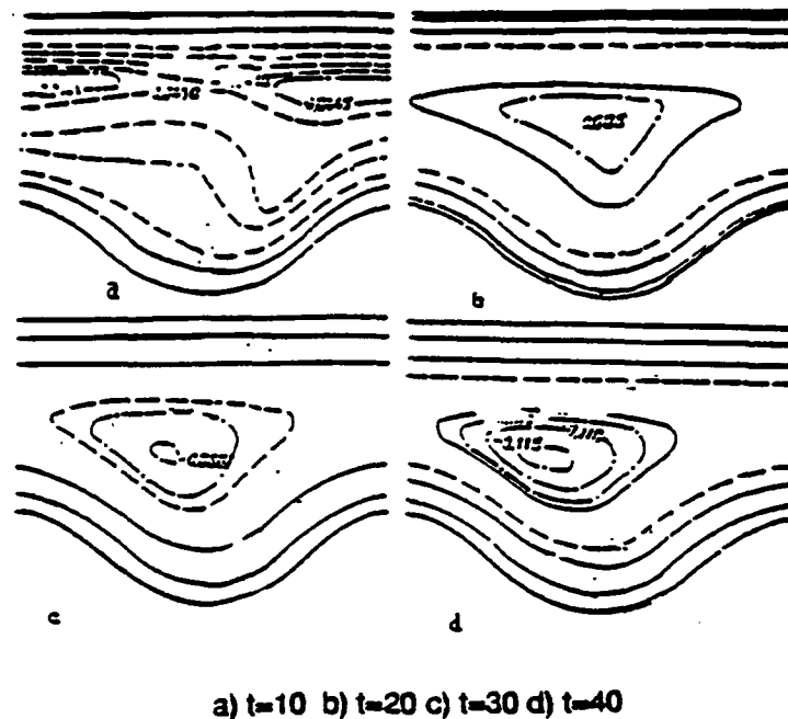
Figure 5. Results of Numerical Computations for Various Times (Kalugin & Panchuk, 1970)
