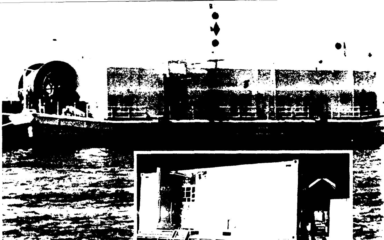
(Above) A barge-mounted, 300,000 gallon-per-day reverse osmosis water purification unit (ROWPU) for assignment to echelons above corps and (inset) a 3,000 gallon-per-hour system for corps-level water units
