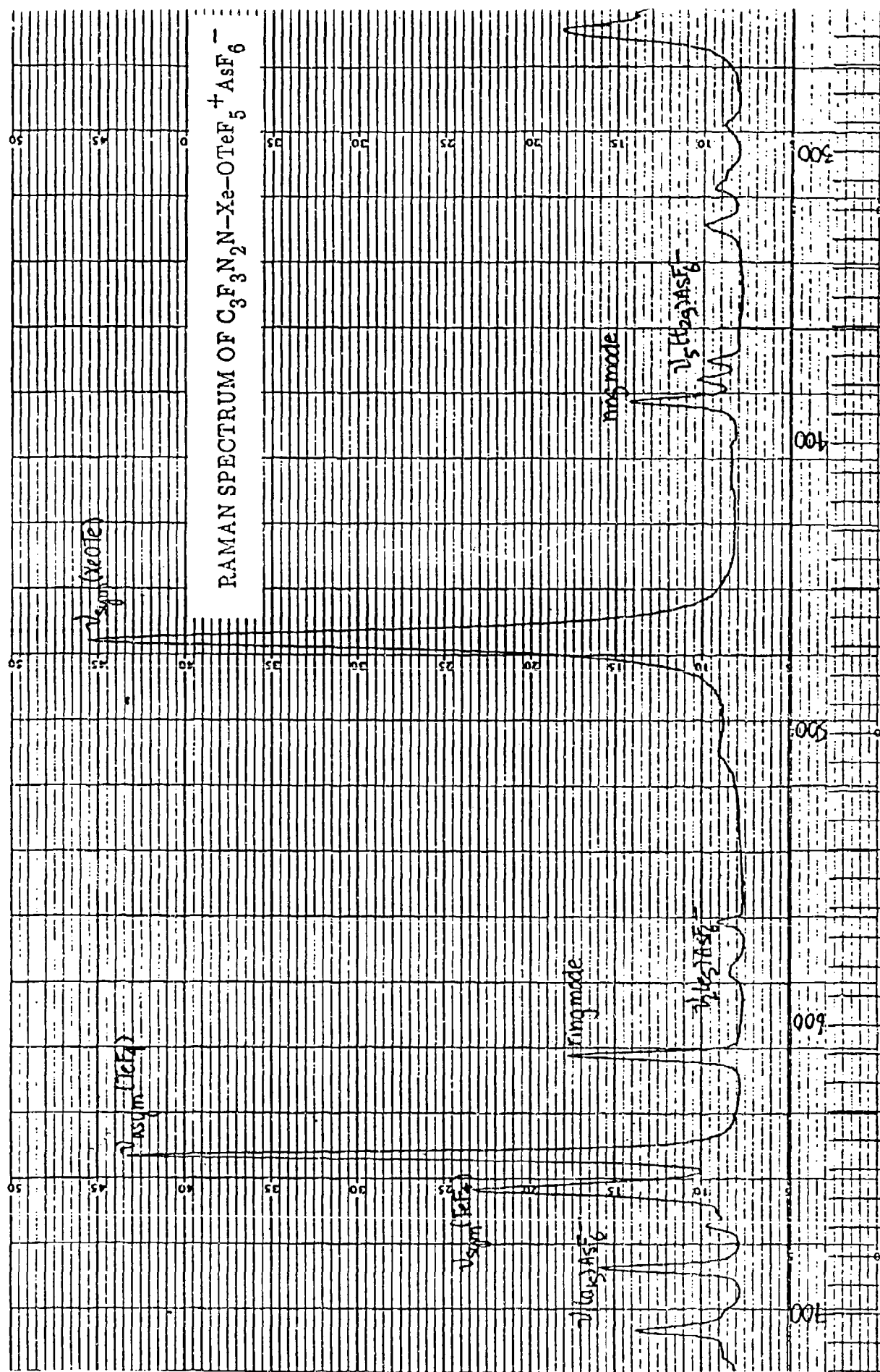
Figure 22. Raman Spectrum of C_3F_3N_2N-Xe-O\text{TeF}_5^+AsF_6^-
