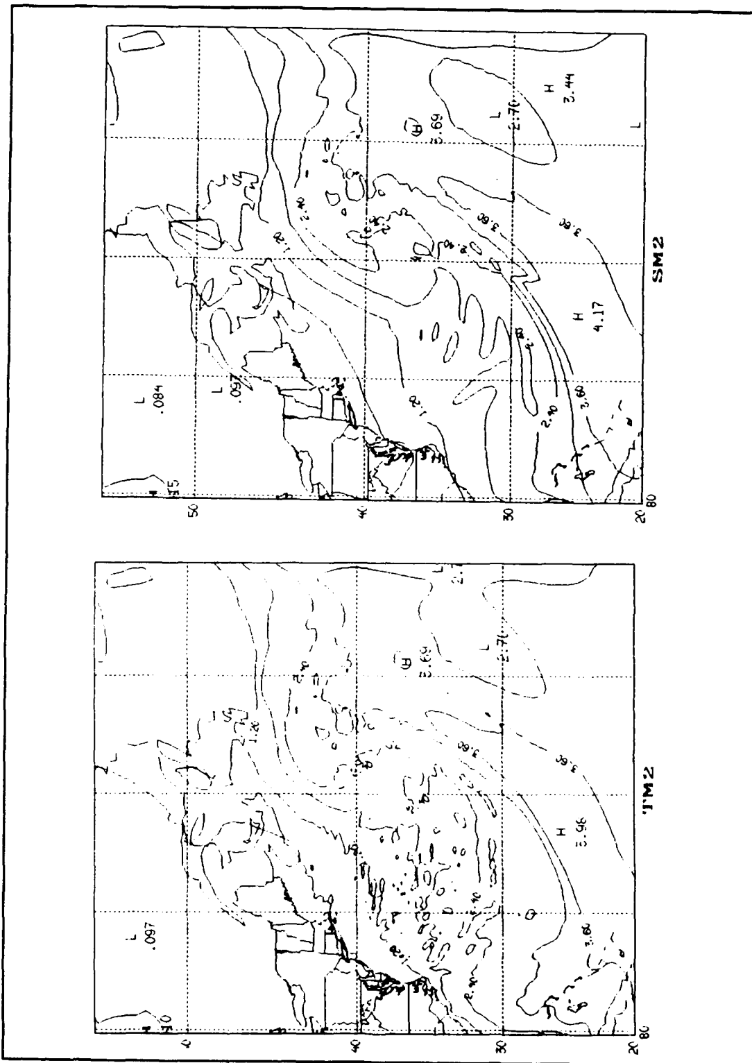
Figure 32. Precipitable water content ( \times 10 \text{ kg/m}^2 ) for TM2 and SM2 at 2400 UTC.
