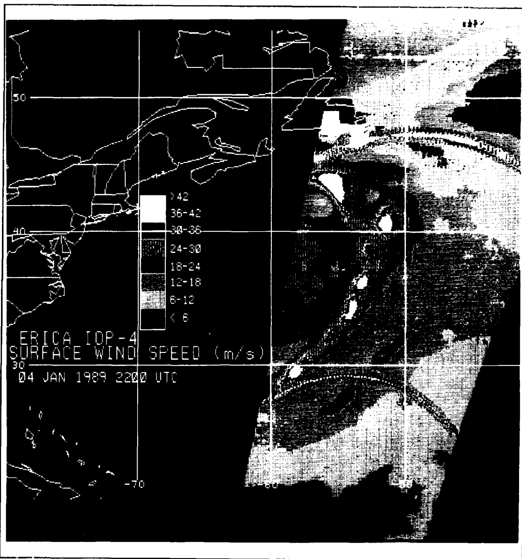
Figure 10. SSM/I wind speed (m/s) at 2200 UTC.
