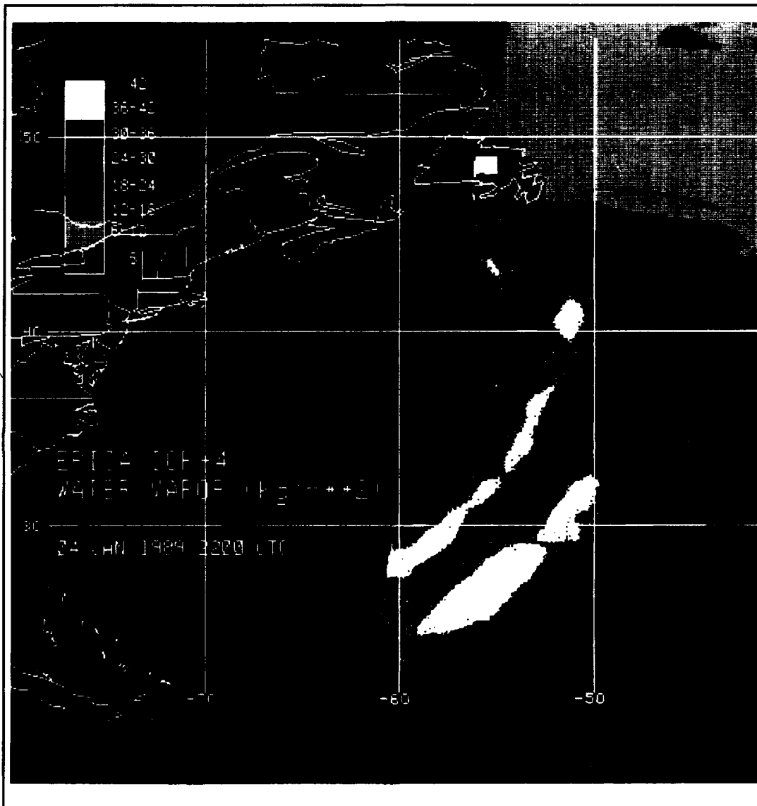
Figure 17. As in Figure 15, but at 2200 UTC.
