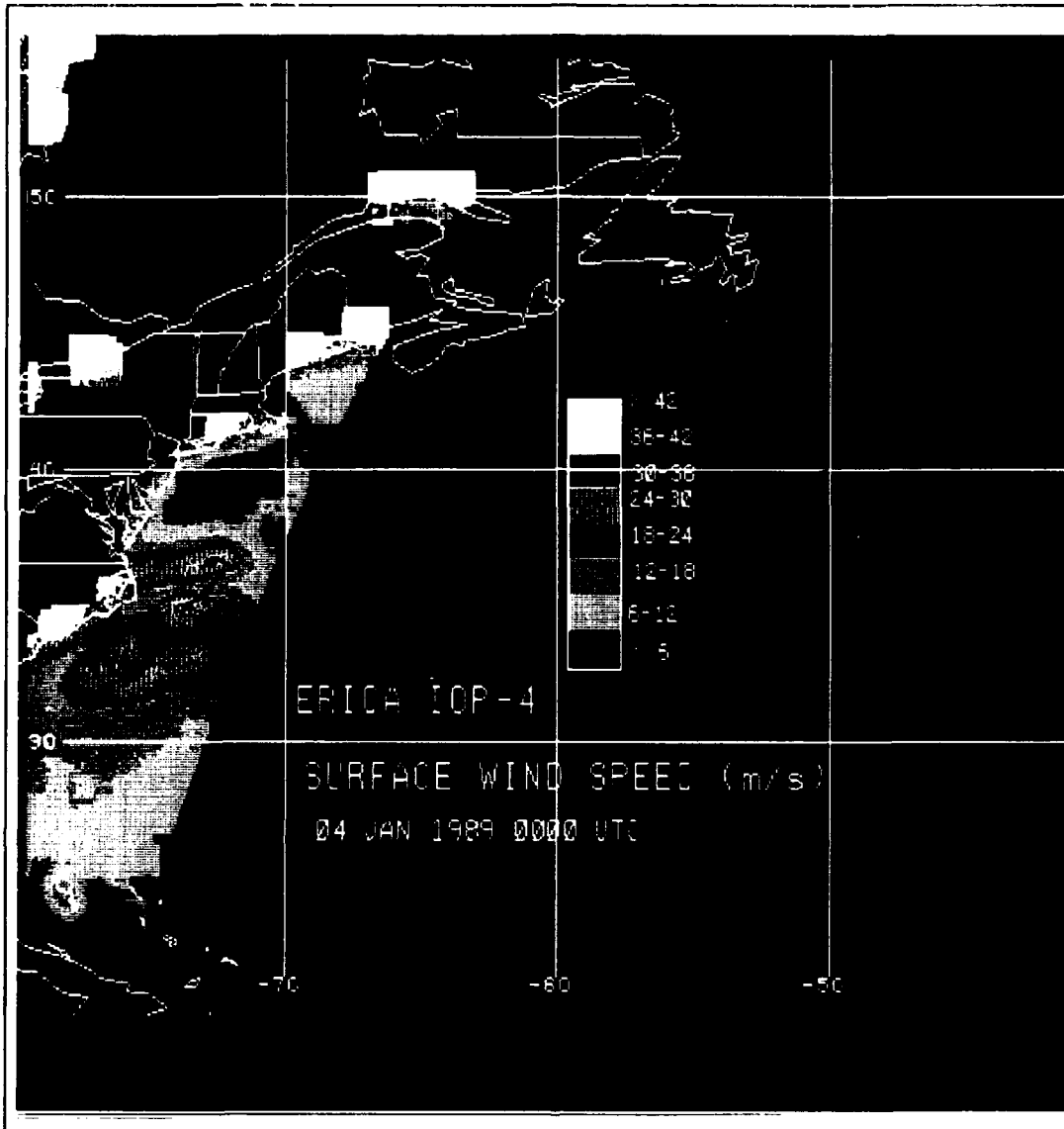
Figure 8. SSM/I wind speed (m/s) at 0000 UTC.
