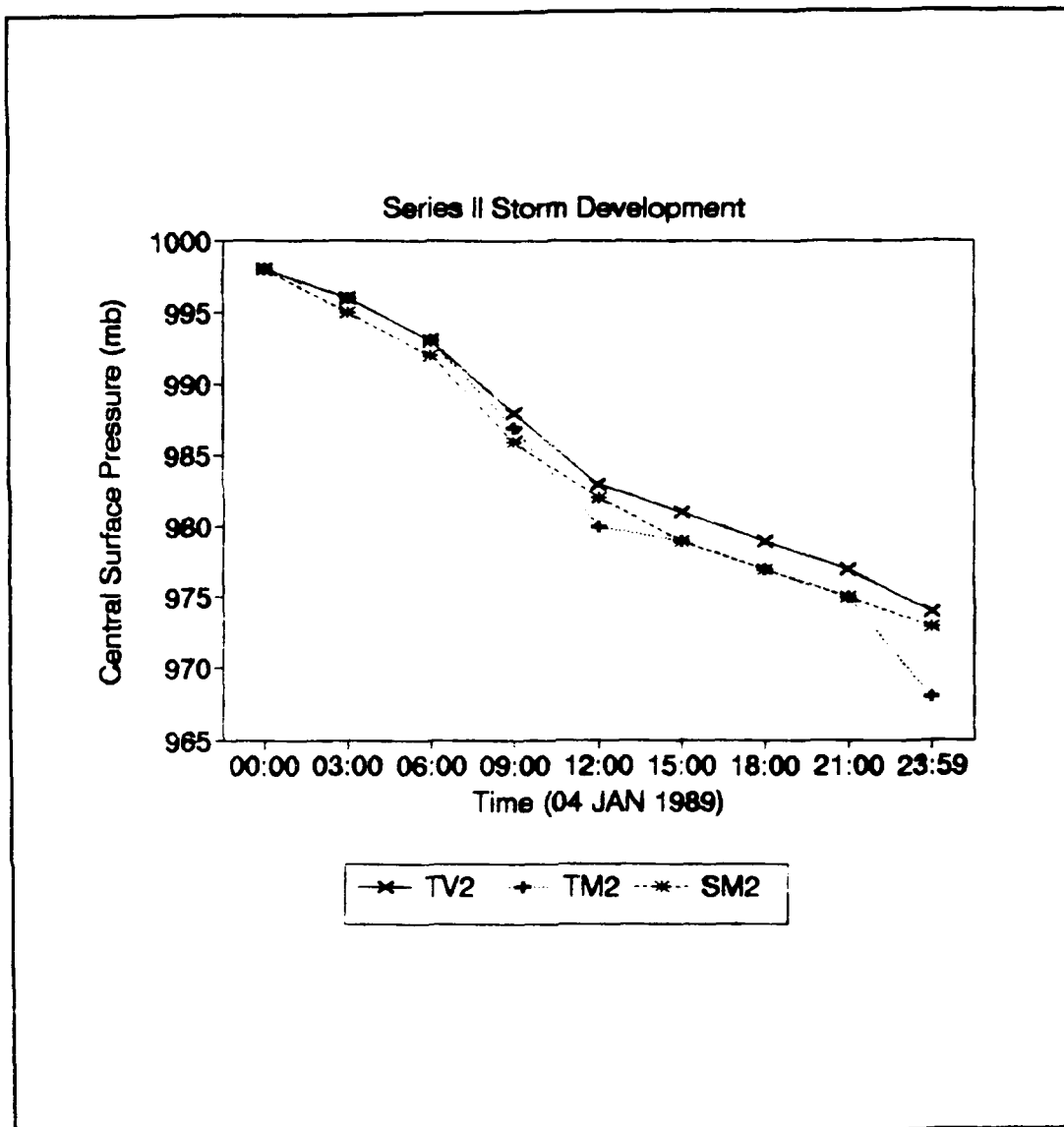
Figure 33. Series II storm development.
