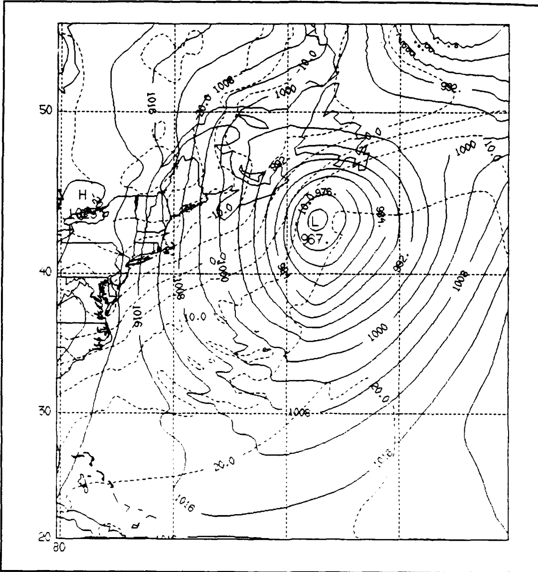
Figure 43. Surface pressure (solid, mb) and temperature (dashed, °C), TW4 at 2400 UTC.
