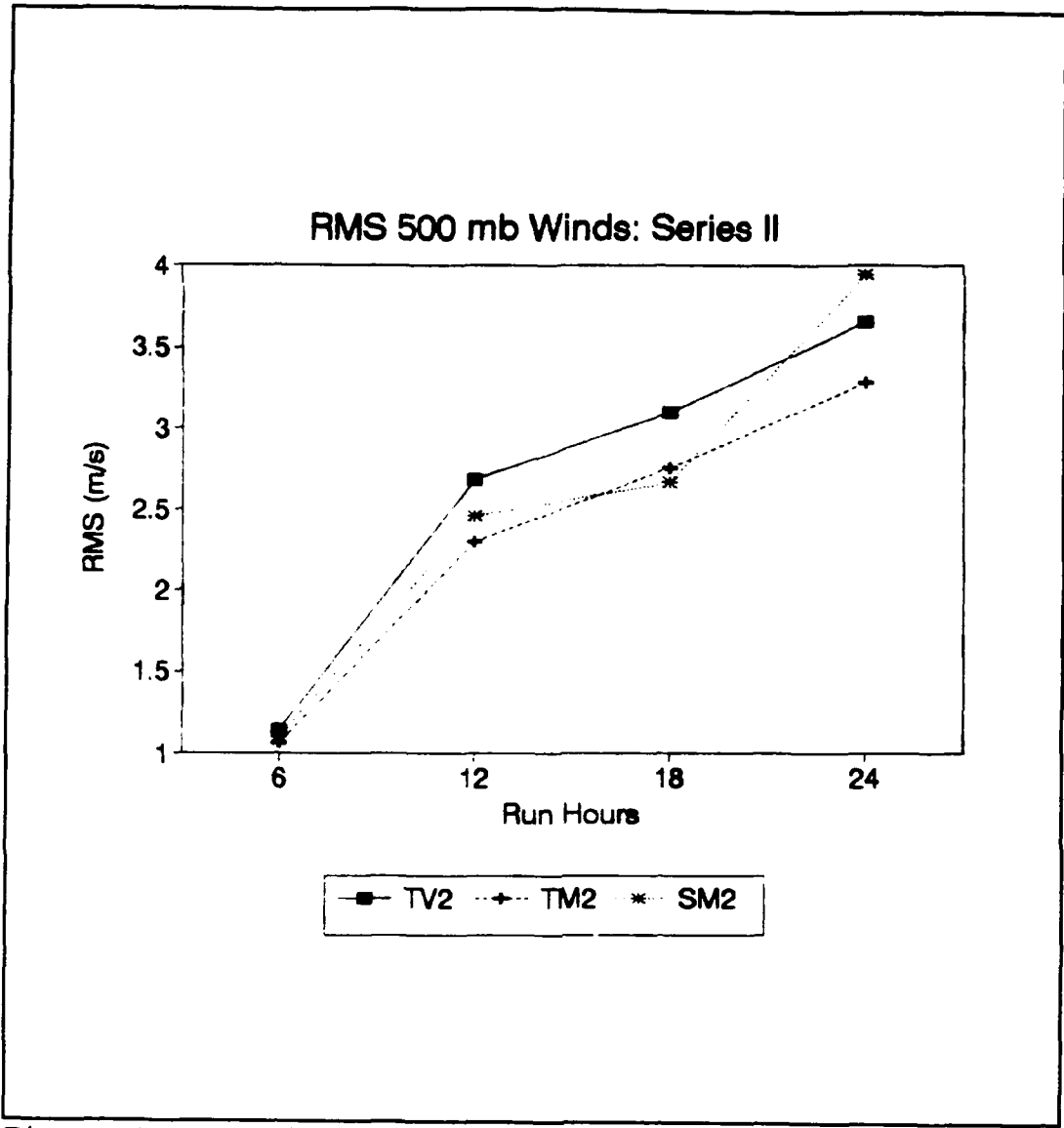
Figure 36. Series II 500 mb wind speed error.
