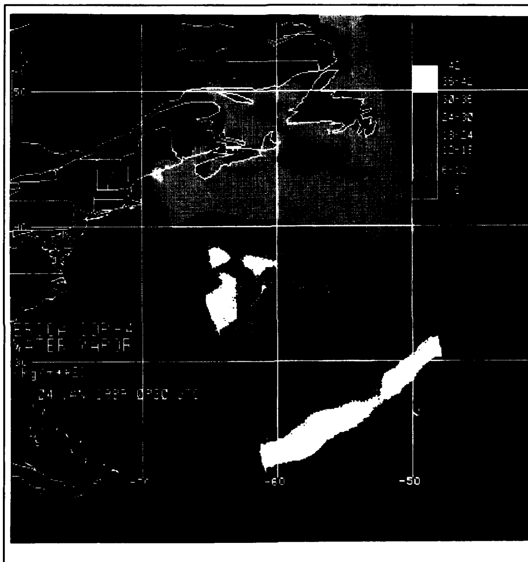
Figure 16. As in Figure 15, but at 0930 UTC.
