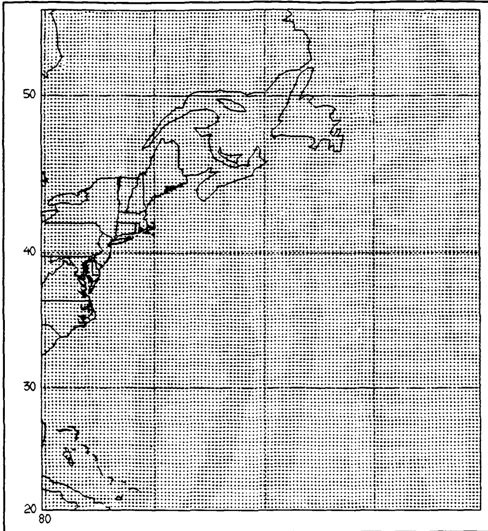
Figure 7. NRL Mesoscale Model domain.
