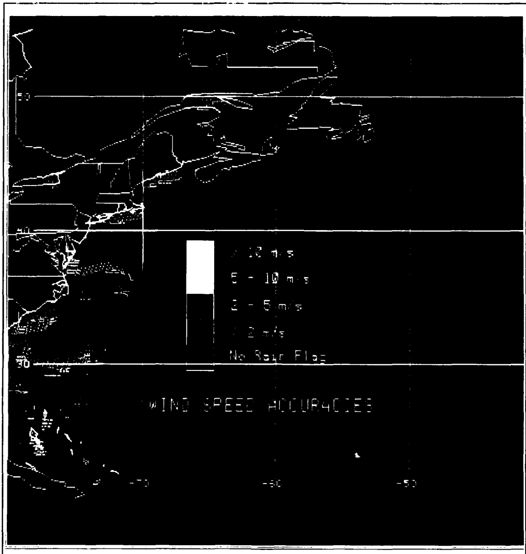
Figure 4. Wind speed accuracies based on SSM/I rain flags for the 0000 UTC swath.
