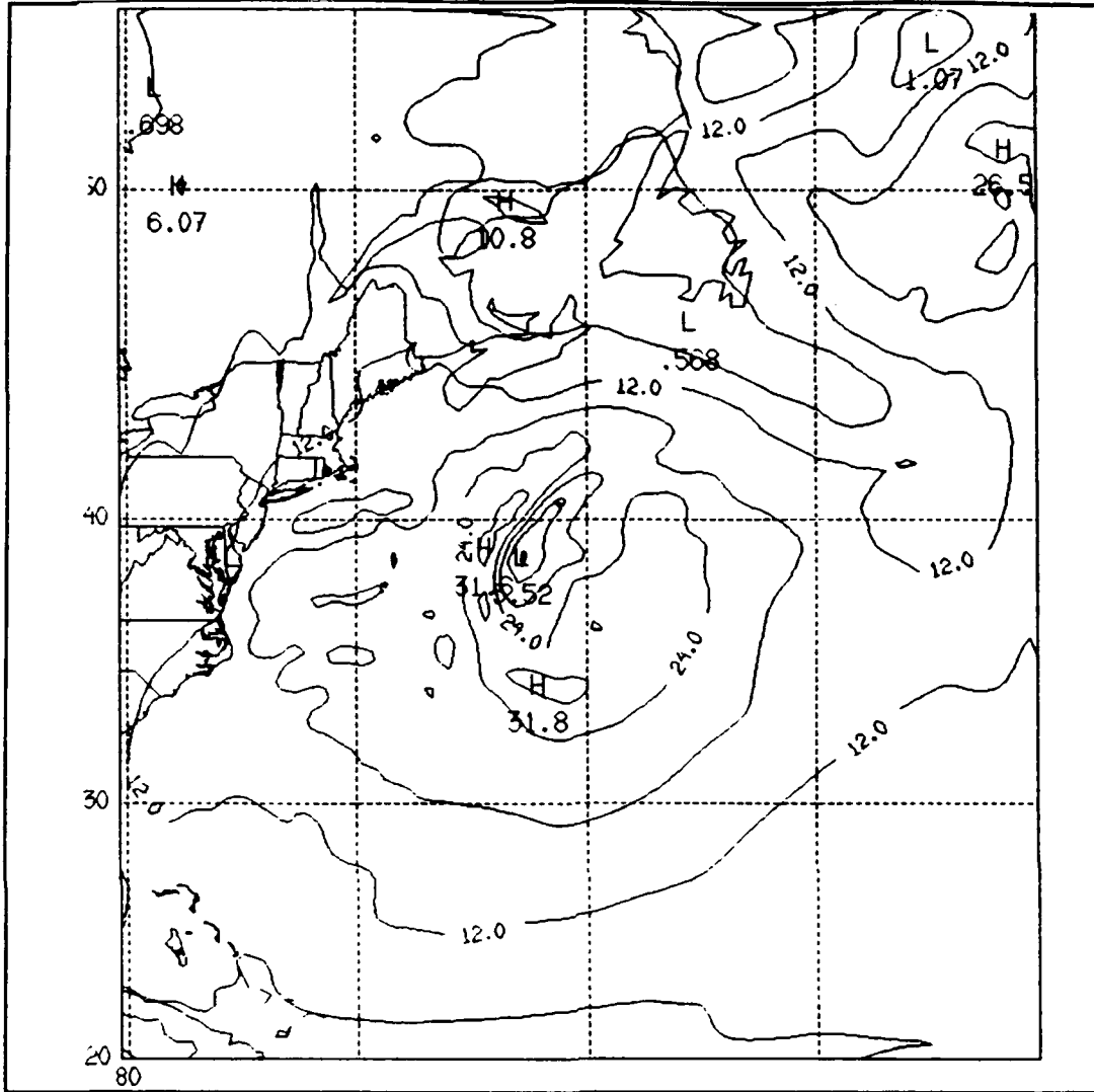
Figure 13. EE16 generated surface wind field (m/s) at 1800 UTC.
