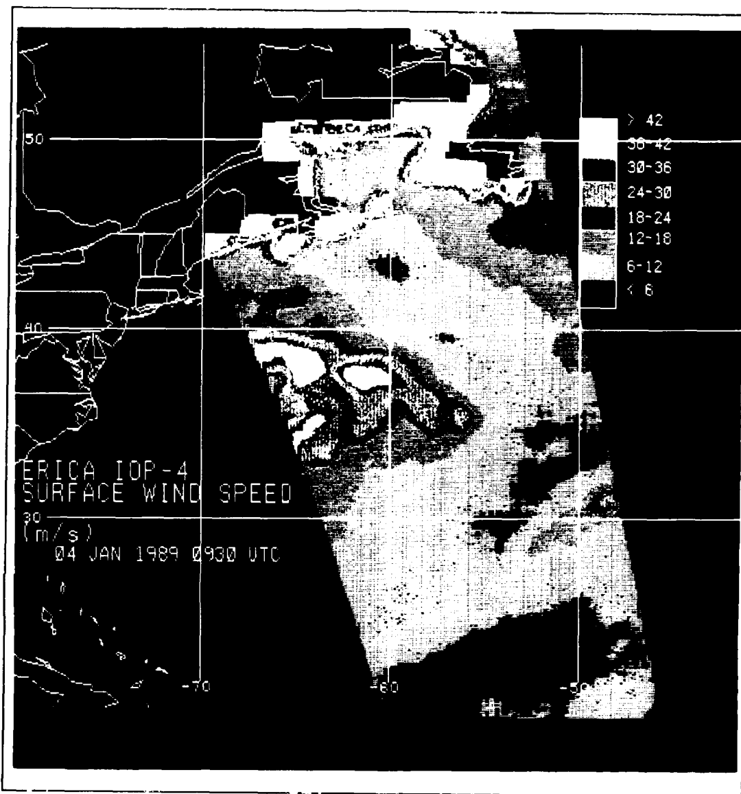
Figure 9. SSM/I wind speed (m/s) at 0930 UTC.
