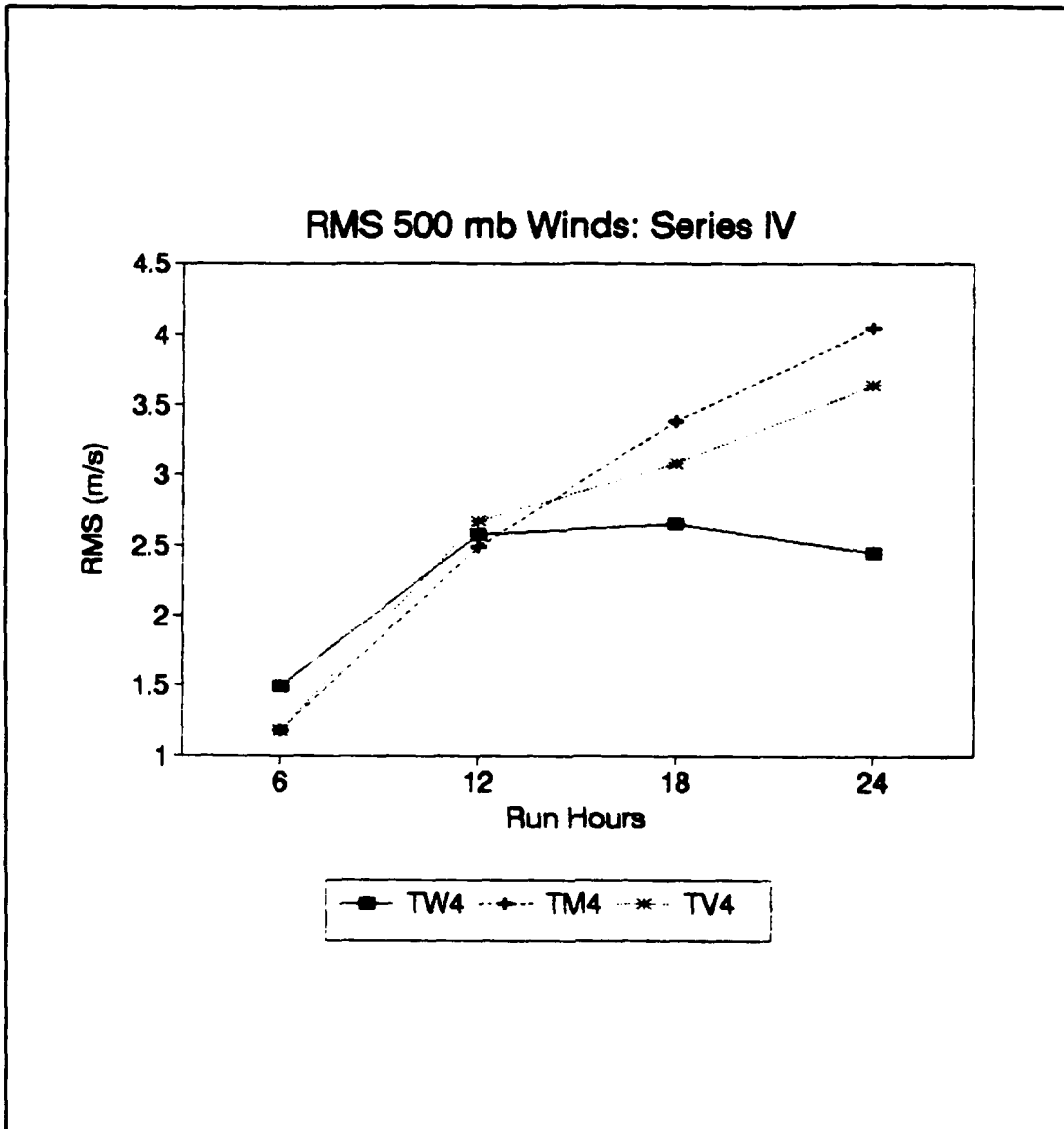
Figure 49. Series IV 500 mb wind RMS errors.
