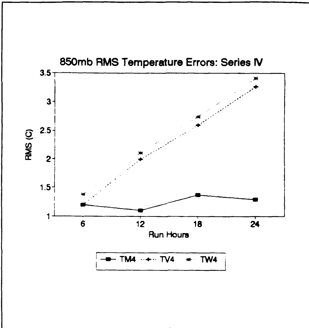
Figure 46. Series IV 850 mb temperature RMS errors.
