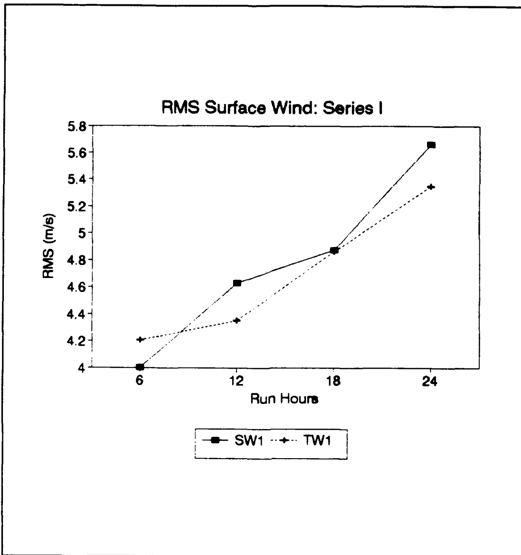
Figure 30. Series I surface wind RMS errors.
