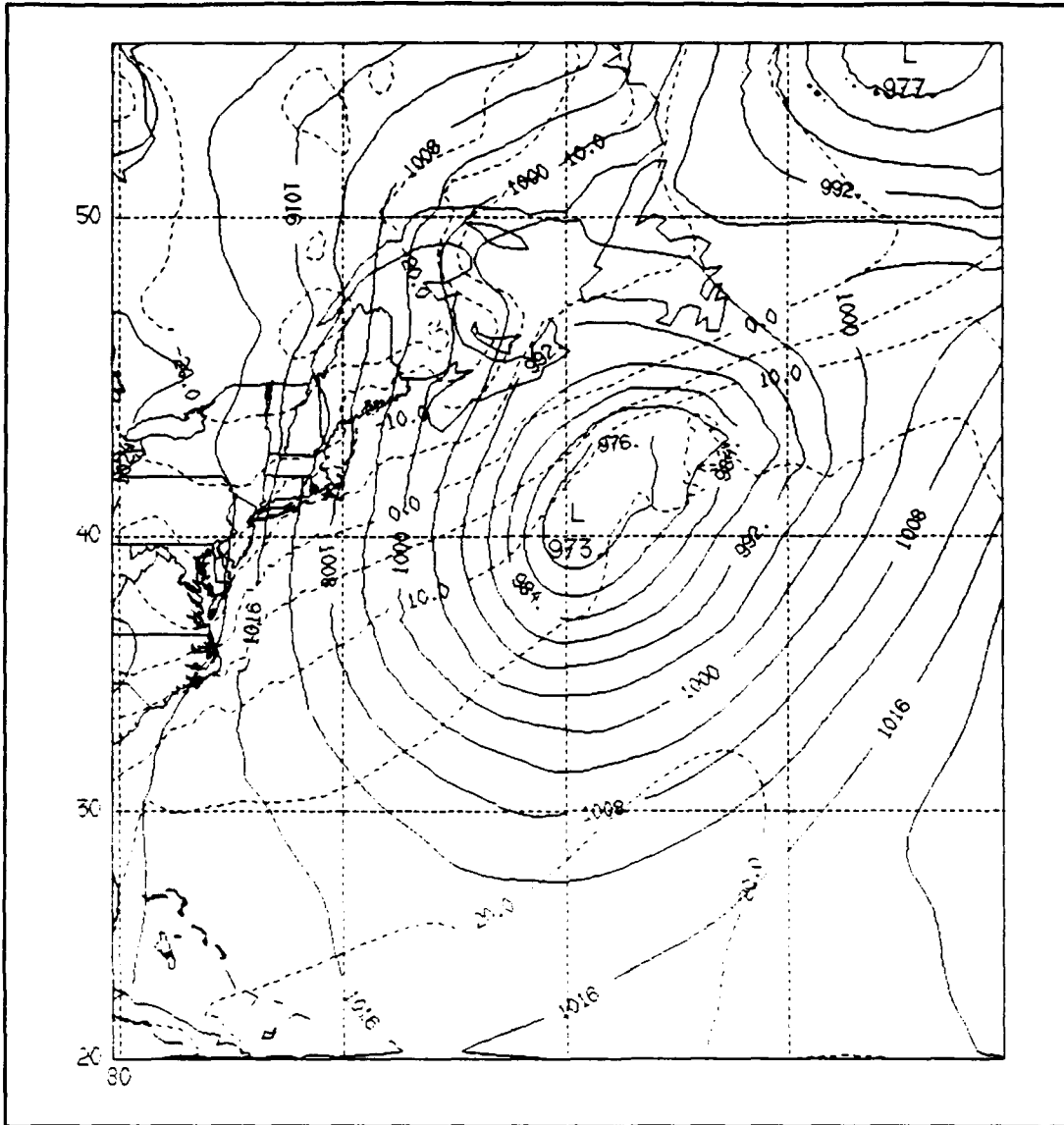
Figure 44. TM4 surface pressure (solid) and temperature (dashed), 2400 UTC.
