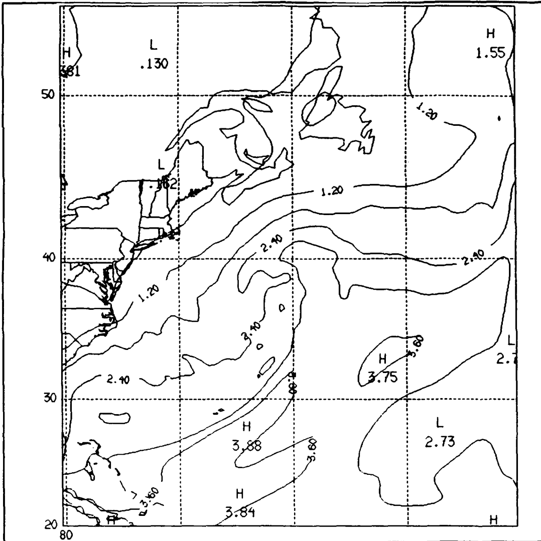
Figure 20. As in Figure 18, but at 1800 UTC.
