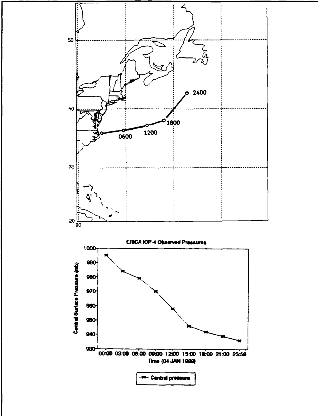
Figure 1. Storm track and central pressure of ERICA IOP-4 storm, 4 January 1989
