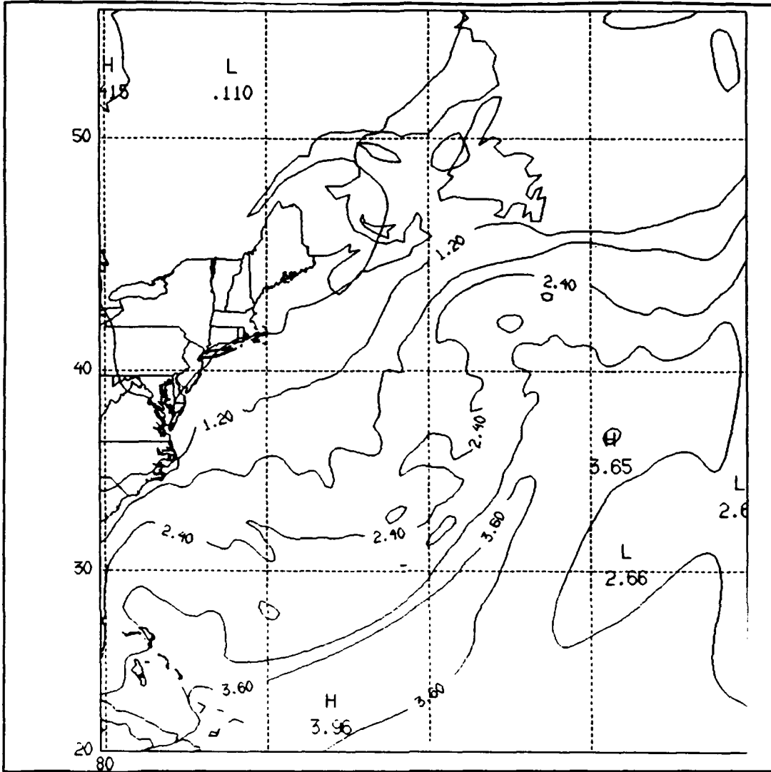
Figure 21. As in Figure 18, but at 2400 UTC.
