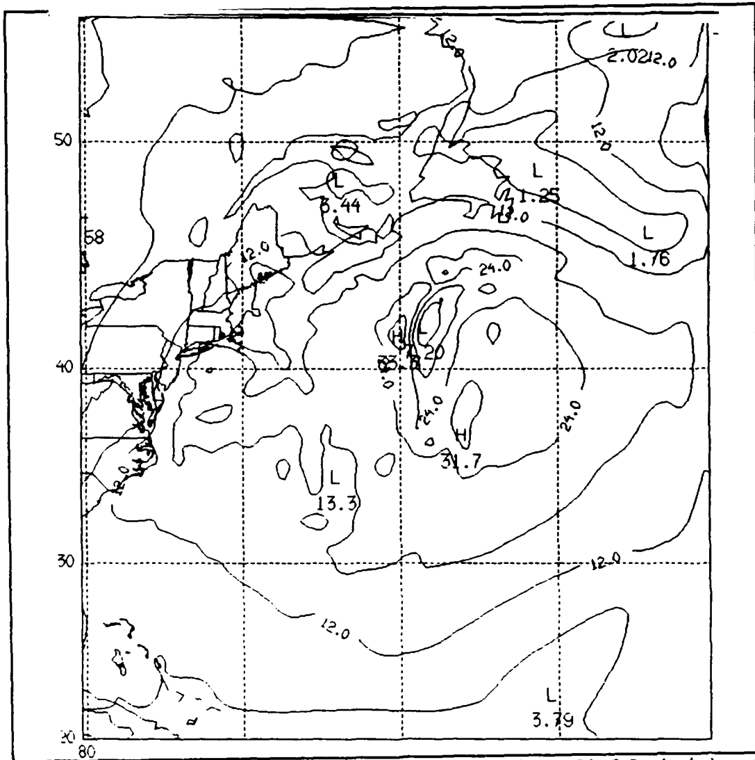
Figure 14. EE16 generated surface wind field (m/s) at 2400 UTC.
