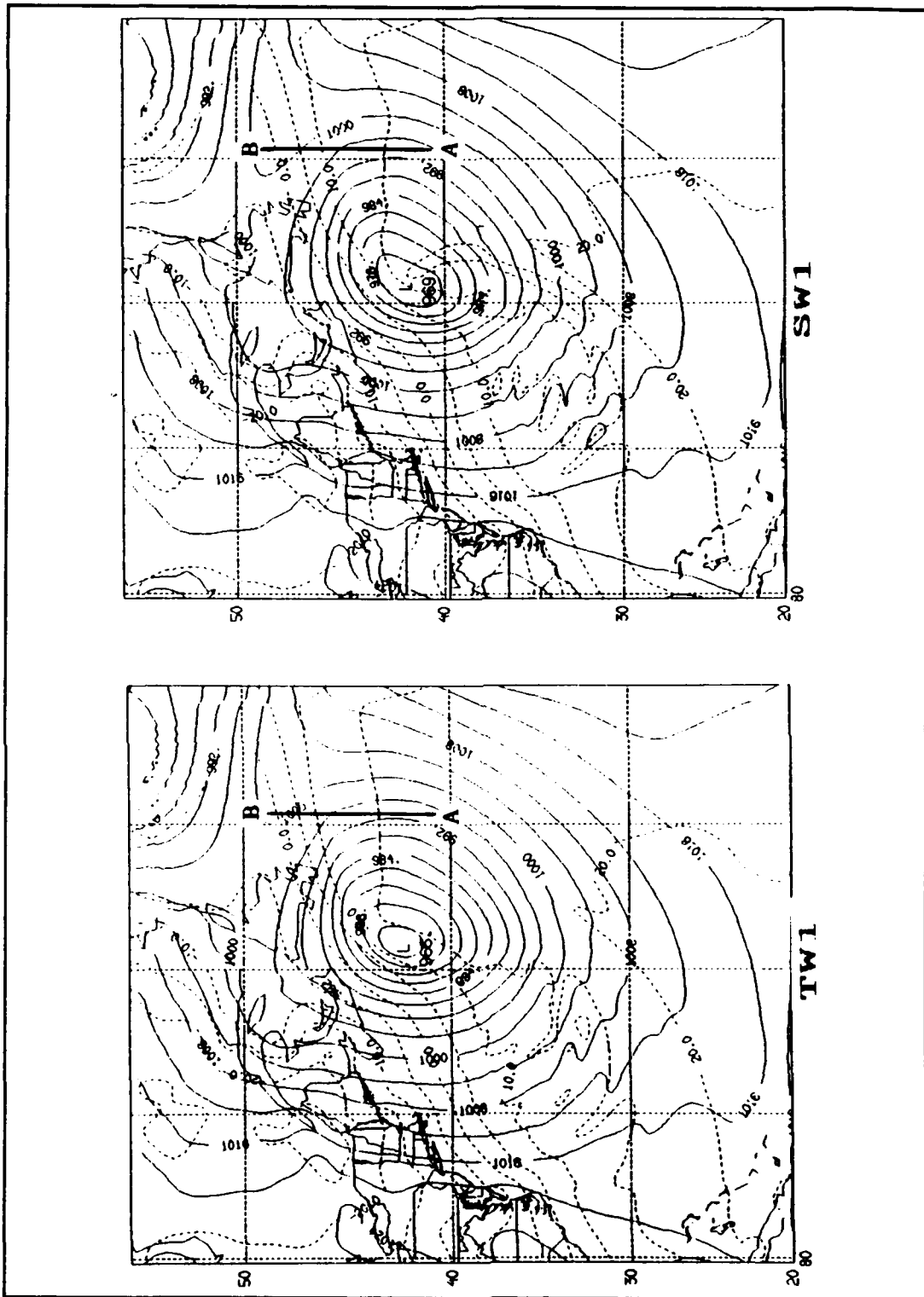
Figure 26. TW1/SW1 surface pressure (solid lines, mb) and temperature (dashed, °C) at 2400 UTC.
