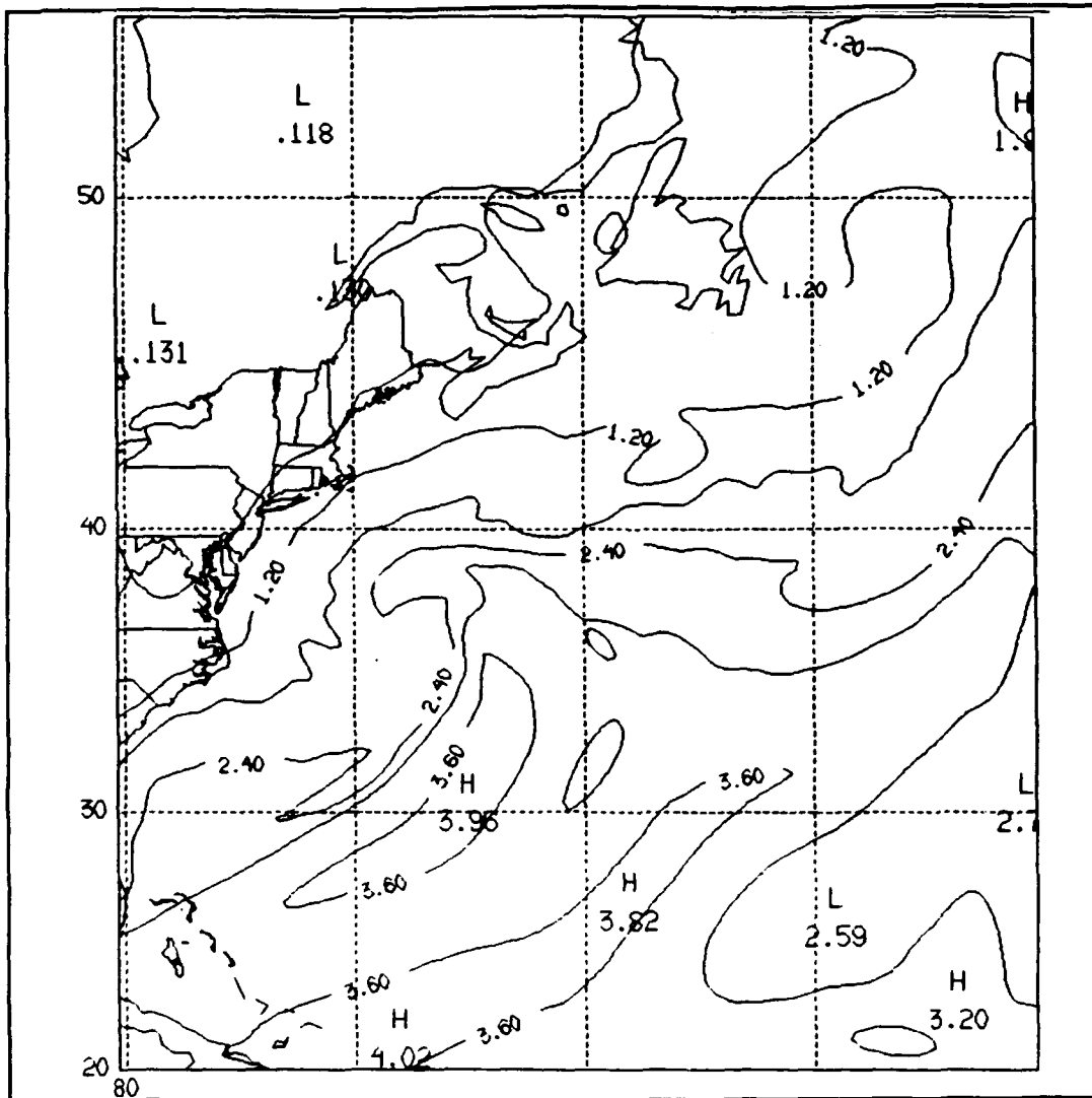
Figure 19. As in Figure 18, but for 1200 UTC.
