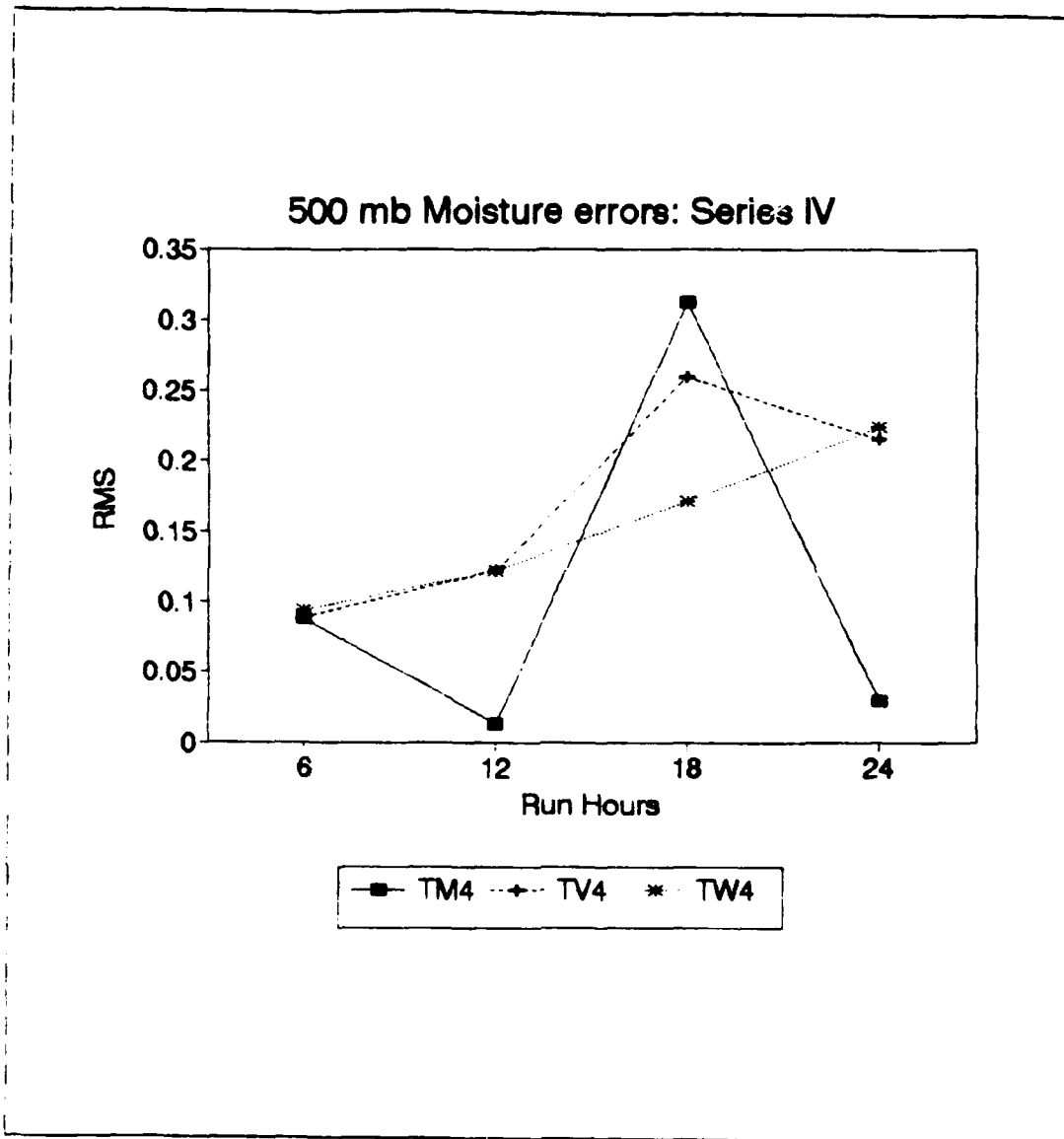
Figure 47. Series IV 500 mb moisture RMS errors.
