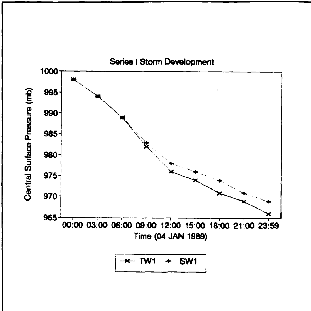
Figure 24. Series I storm development.
