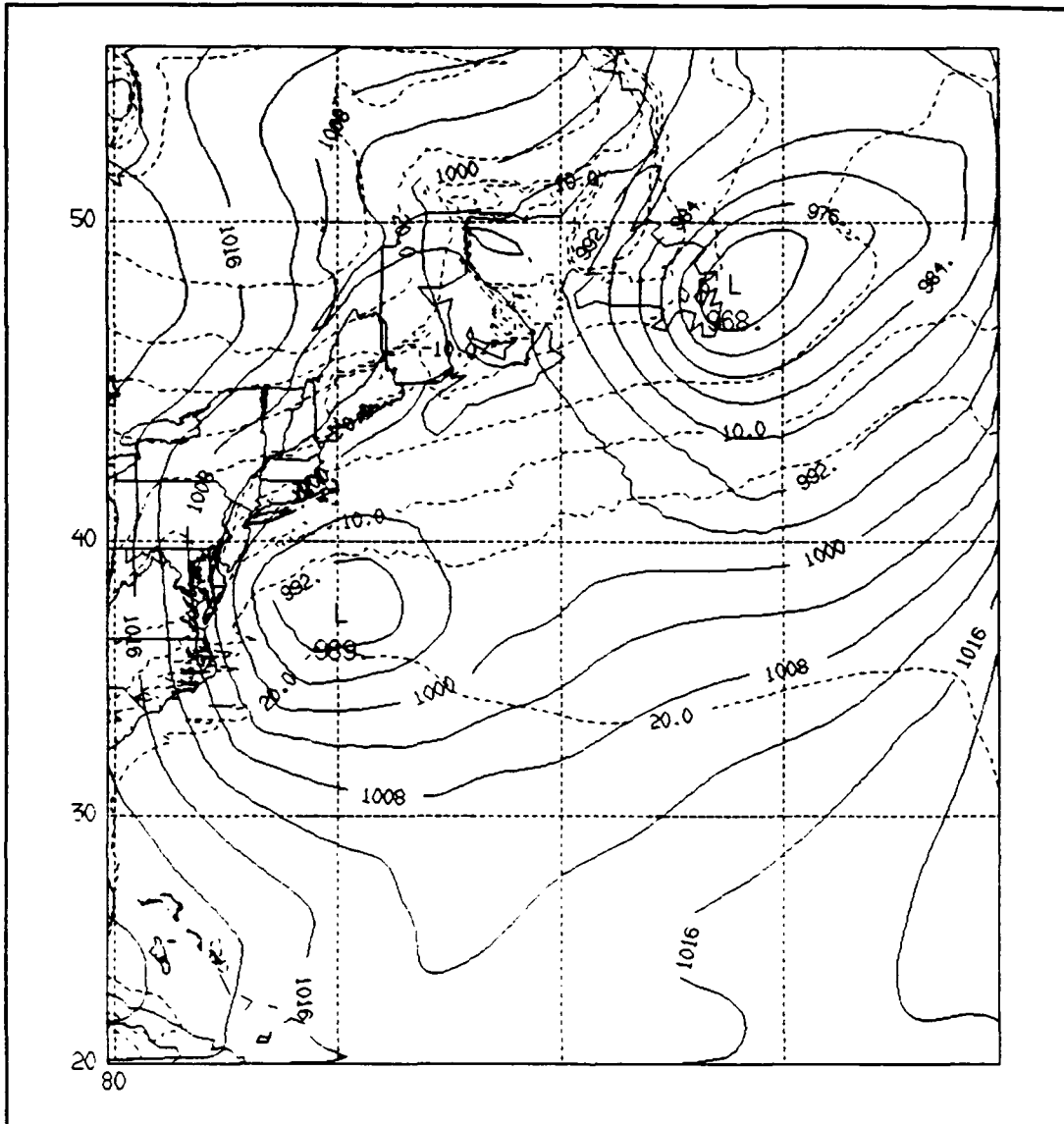
Figure 42. TW4 surface pressure (solid, mb) and temperature (dashed, °C) at 0600 UTC.
