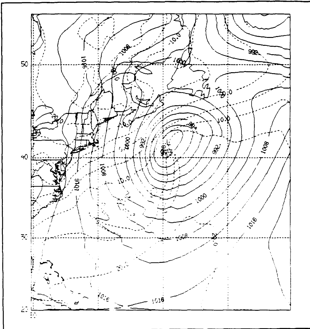
Figure 45. TV4 surface pressure (solid) and temperature (dashed), 2400 UTC.
