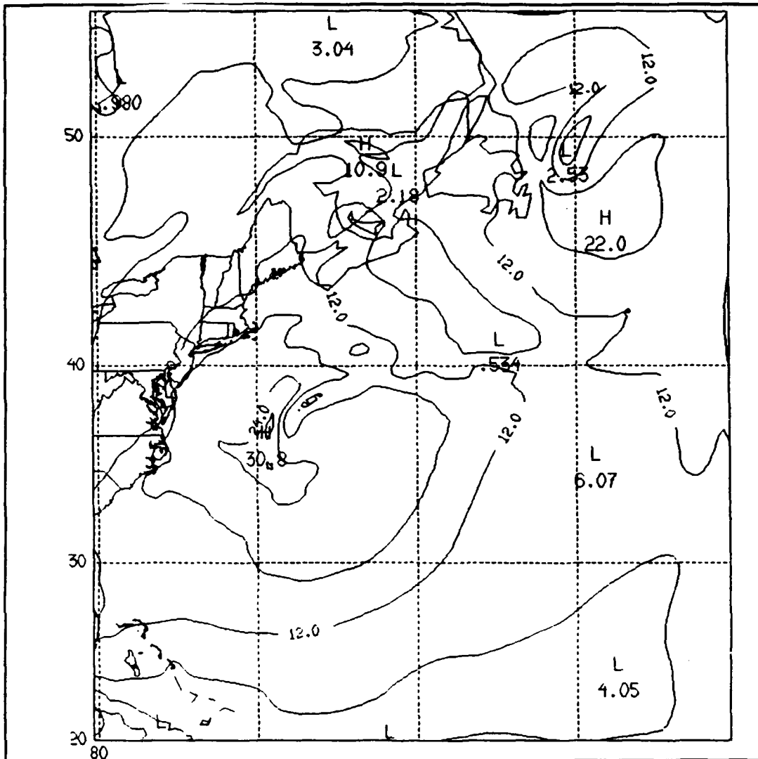
Figure 12. EE16 generated surface wind field (m/s) at 1200 UTC.
