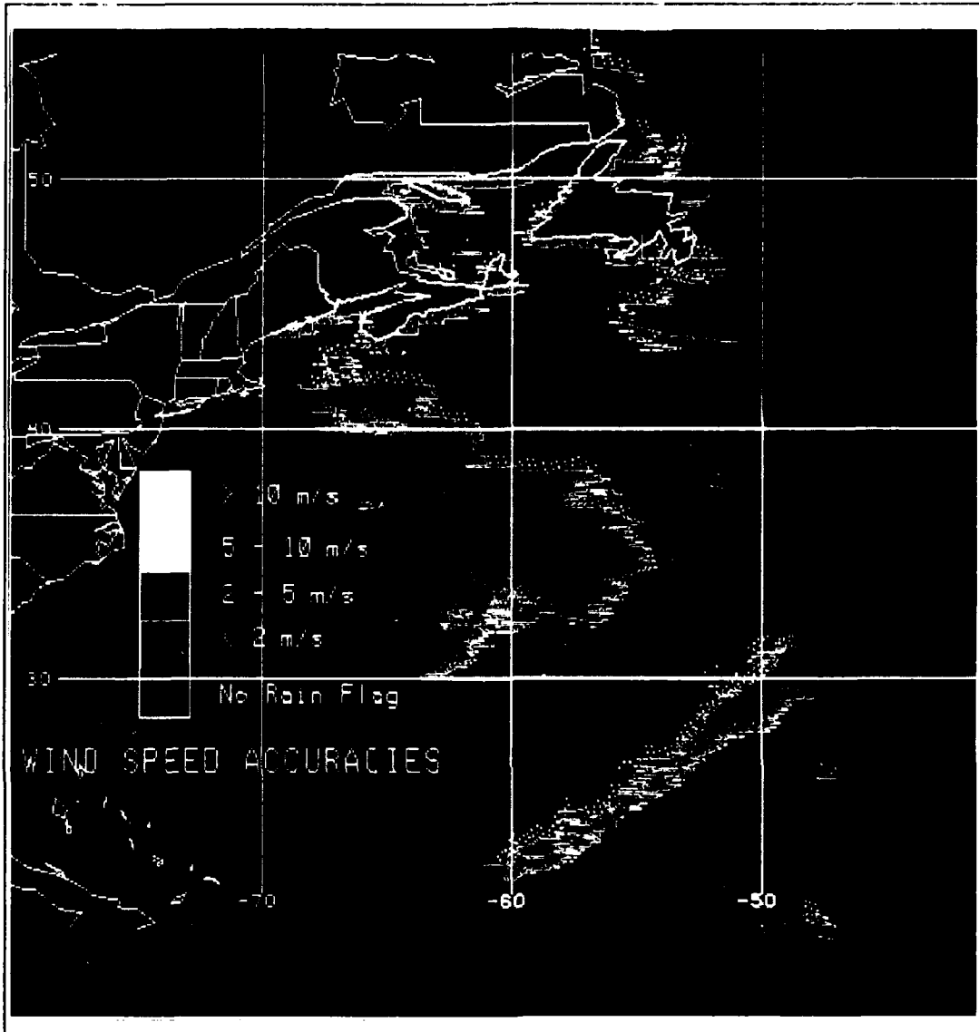
Figure 5. Wind speed accuracies as in Figure 4, but for the 0930 UTC swath.
