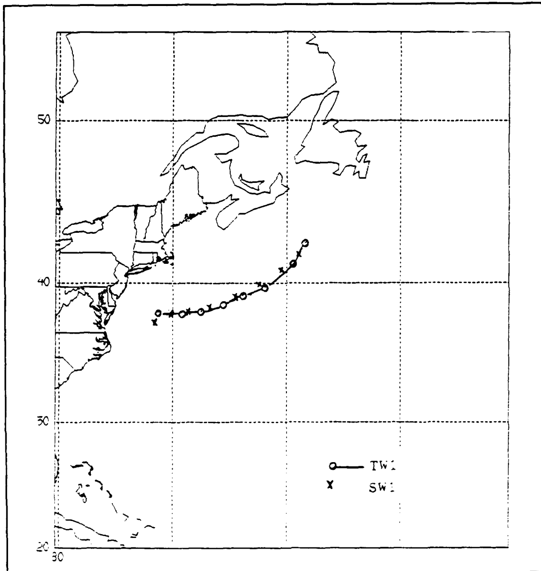
Figure 31. SW1 vs. TW1 storm tracks.
