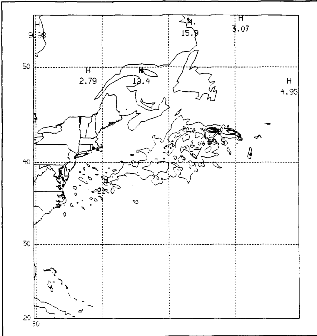
Figure 35. 24 hour accumulation of precipitation (cm) for TM2. Contour interval is 10 cm.
