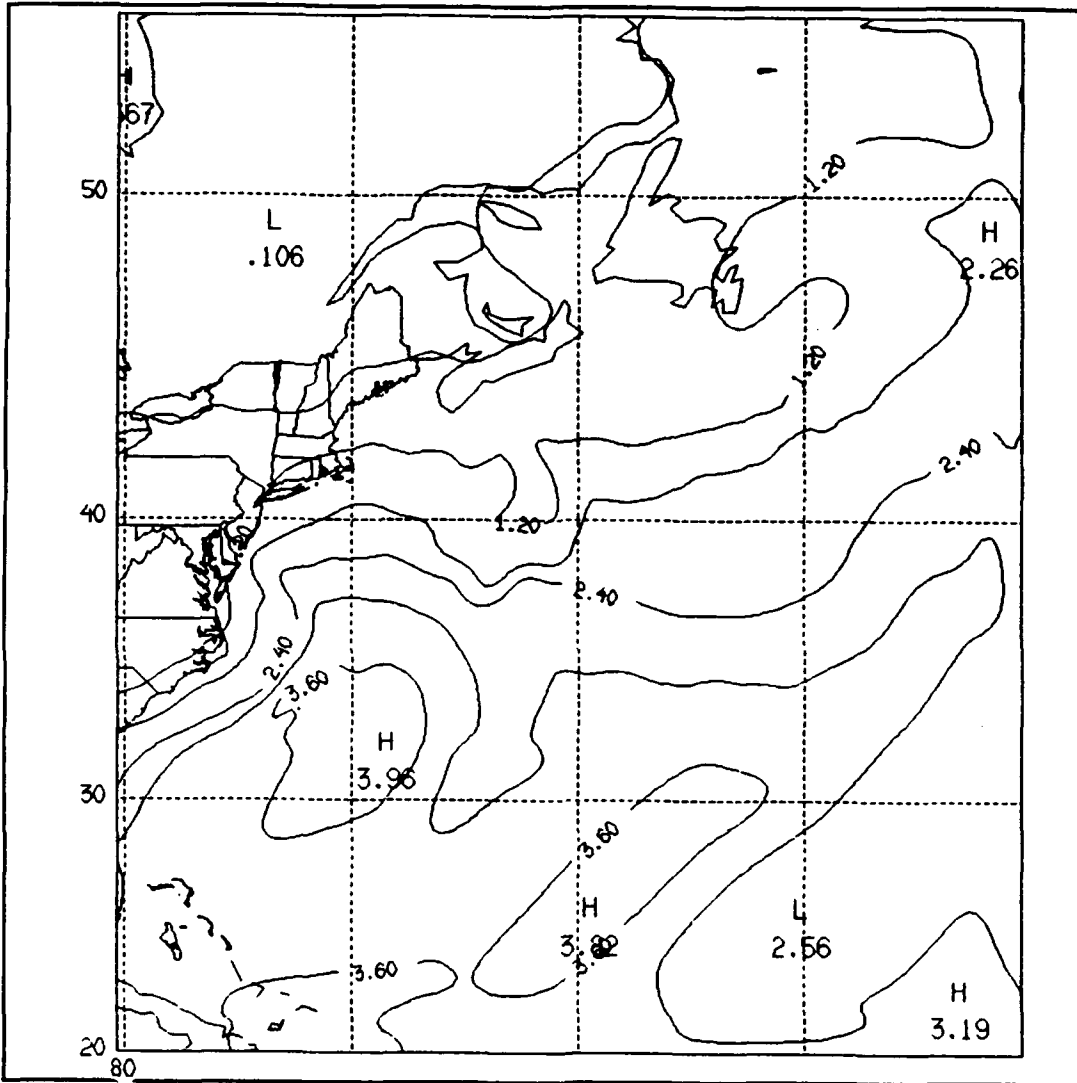
Figure 18. EE16-generated precipitable water ( x 10 kg/m 2 ) at 0600 UTC.
