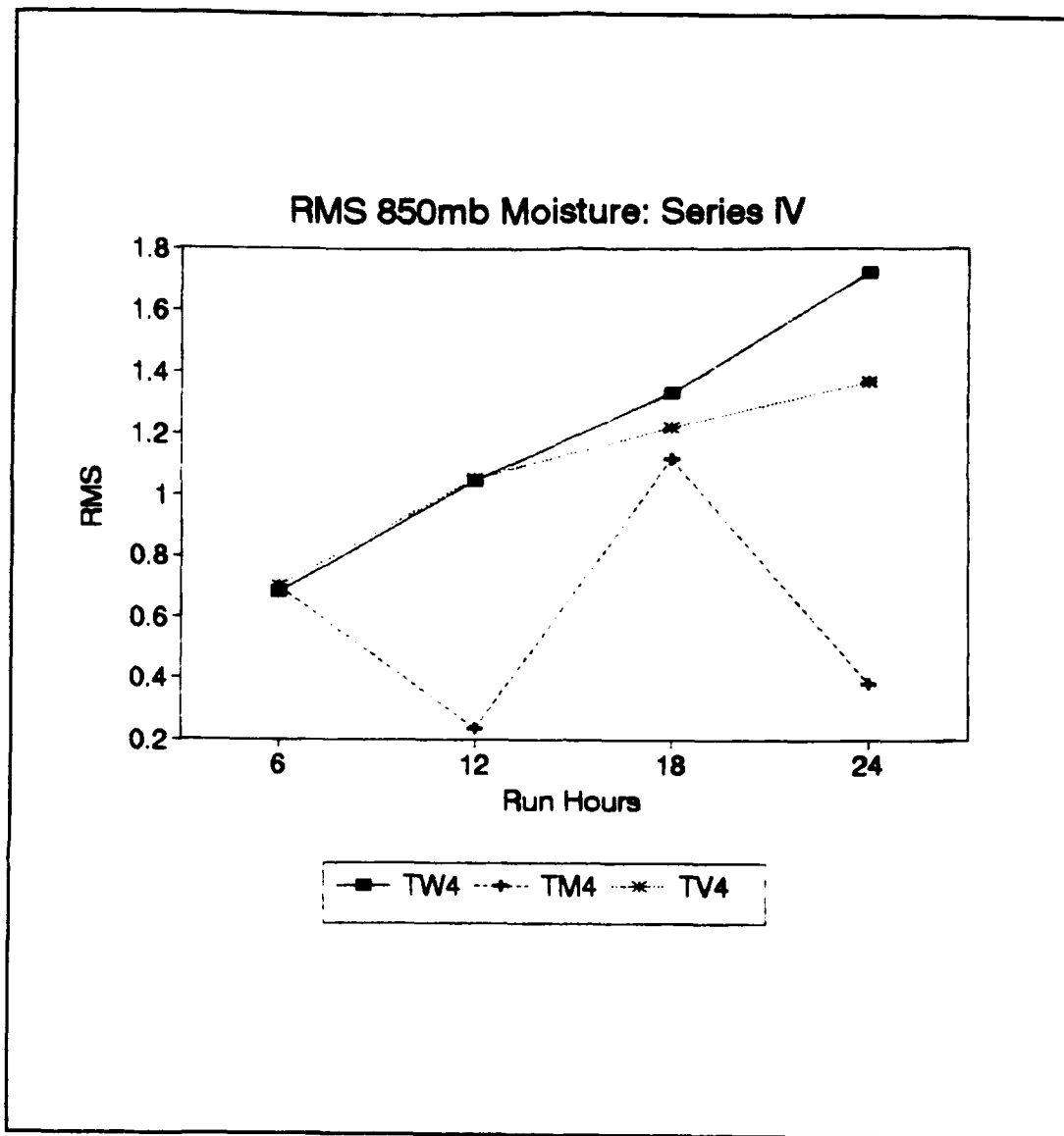
Figure 48. Series IV 850 mb moisture RMS errors.
