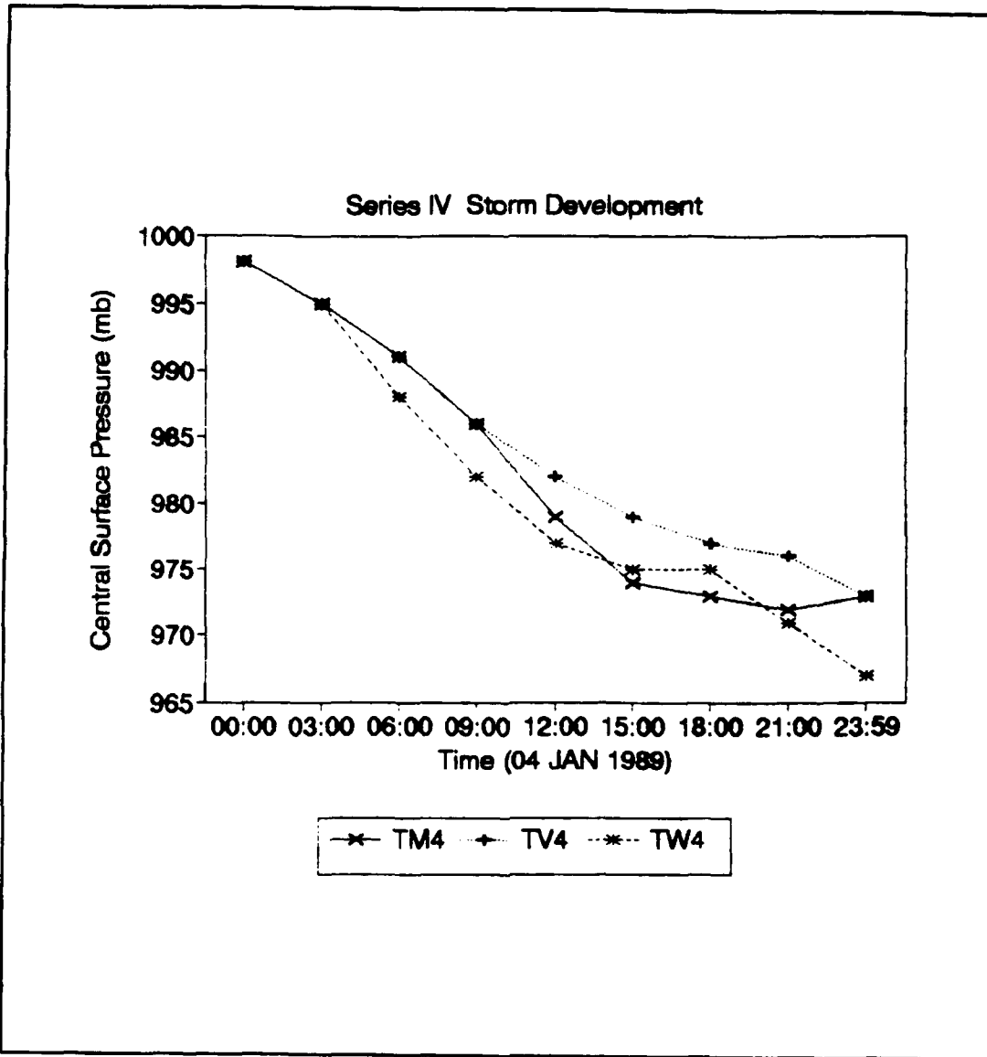
Figure 41. Series IV storm development.
