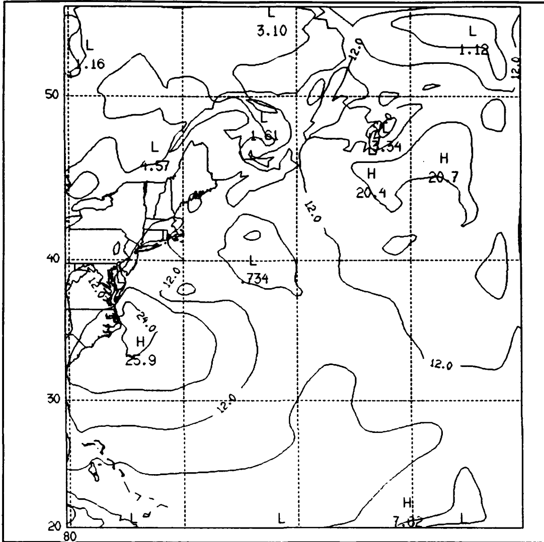
Figure 11. EE16 generated surface wind field (m/s) at 0600 UTC.
