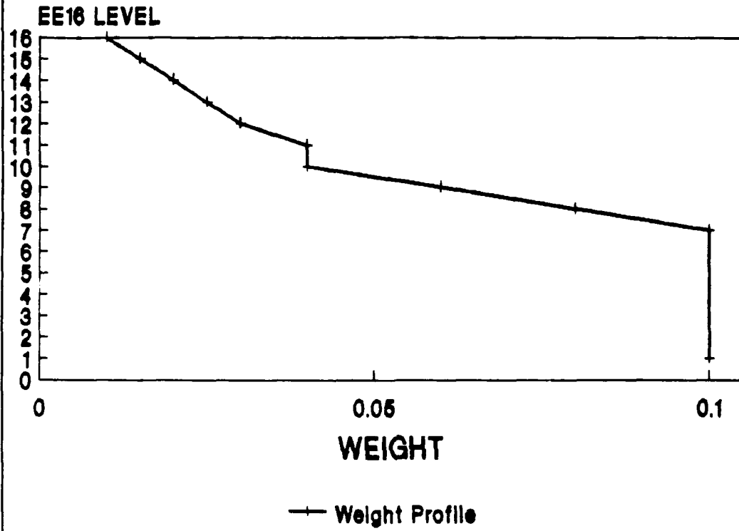
Figure 23. Vertical weighting function for conversion of 16 Layer data to 10 Layers.
