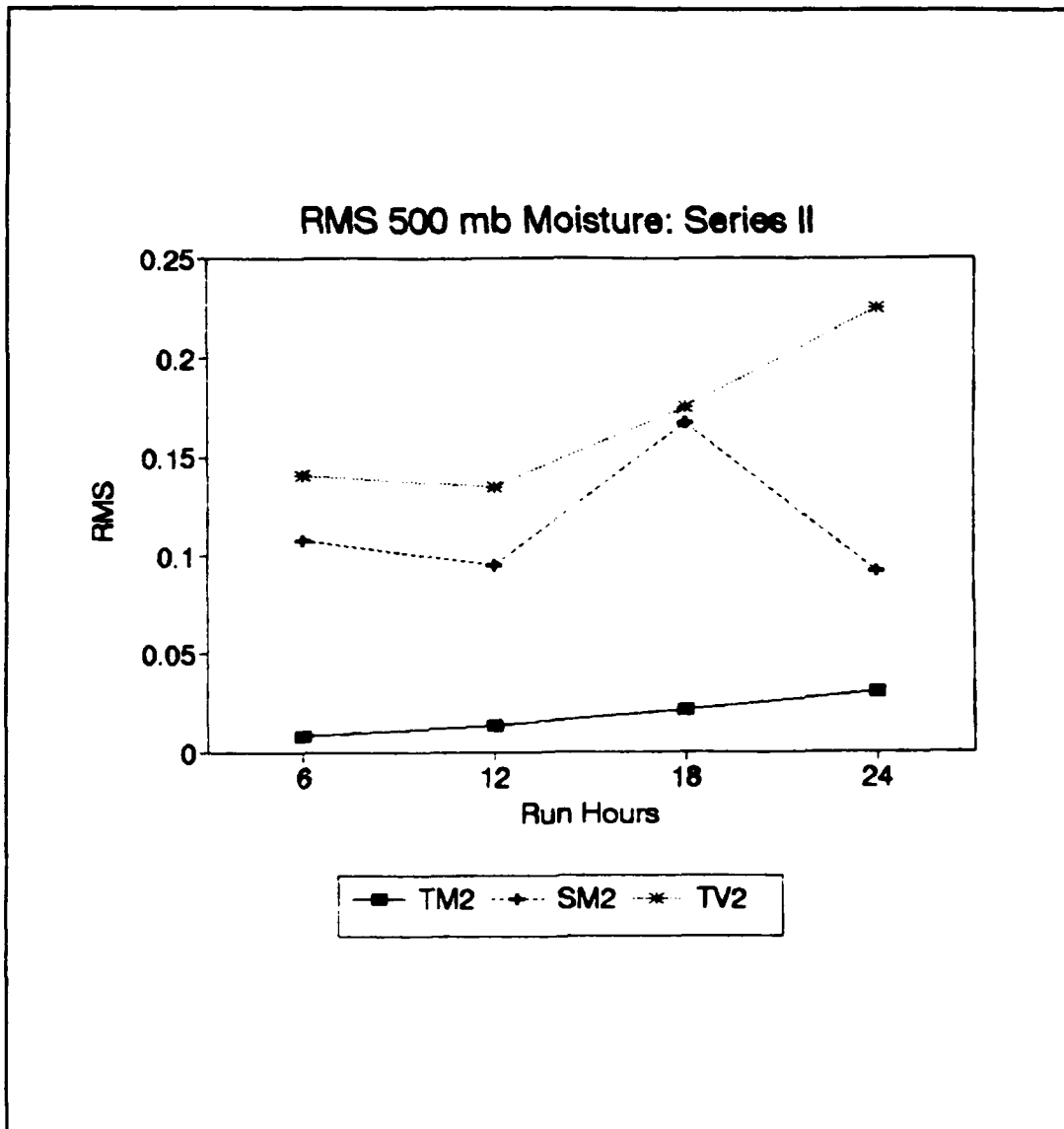
Figure 37. Series II 500 mb moisture RMS error.
