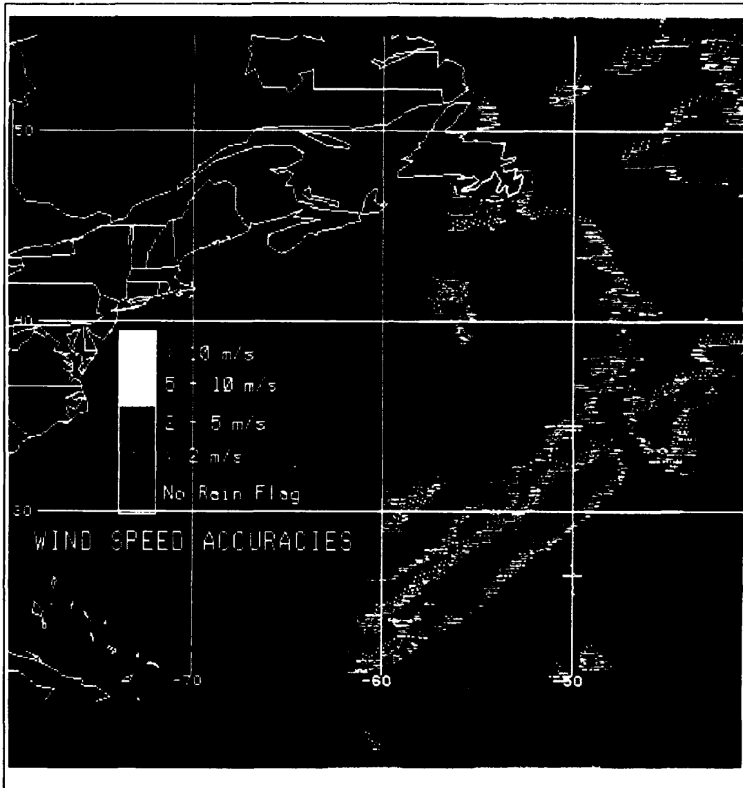
Figure 6. Wind speed accuracies as in Figure 4, but for the 2200 UTC swath.
