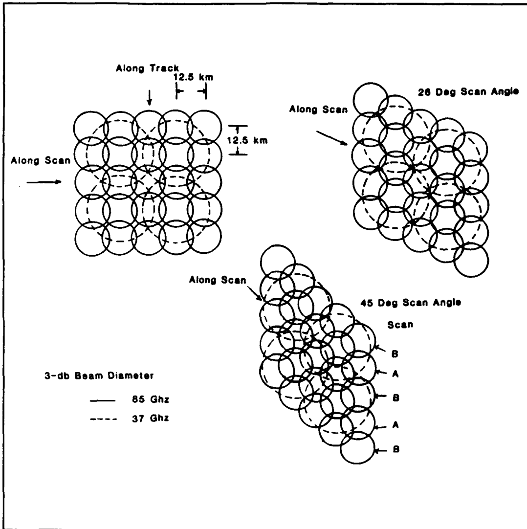
Figure 3. SSM/I 37 Ghz and 85 Ghz channels beam footprints within a swath for various angles from the nadir (Hollinger et al., 1987).
