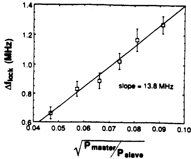
Figure 2: Injection locking range versus the square root of the master oscillator power to the slave oscillator power. The data is fit to a straight line with a slope of 13.8 MHz.
