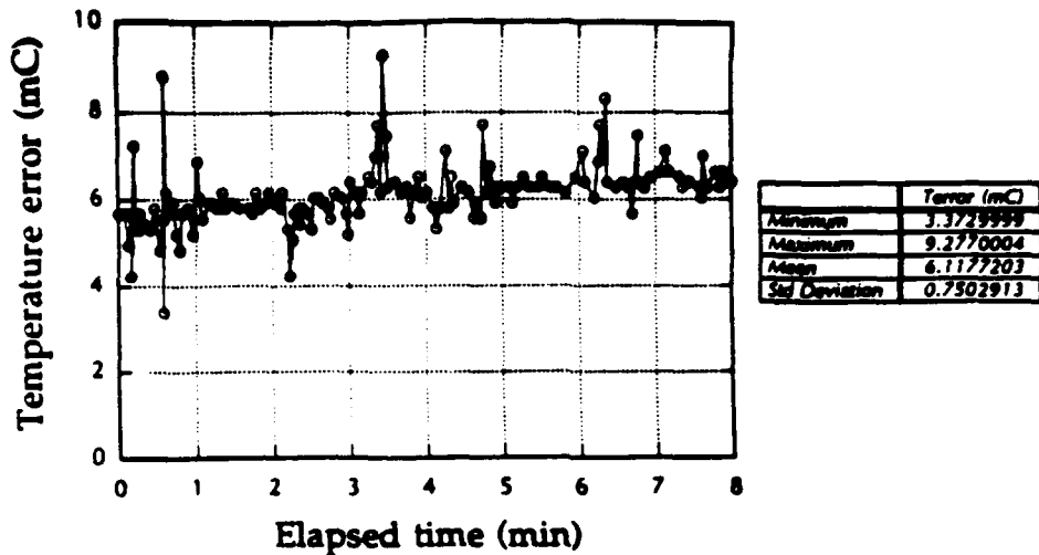
Figure 17: Temperature controller error vs time. The diode temperature is kept within 15mC of the setpoint under actual operating conditions.
