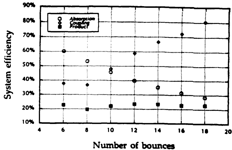
Figure 12: Variations in absorption efficiency and coupling efficiency with number of bounces. Absorption efficiency decreases due to the decreasing thickness of the slab. Coupling efficiency increases as the signal beam spends more of its time in the strongly pumped regions of the slab. The product of these two efficiencies is approximately constant with bounce number.
