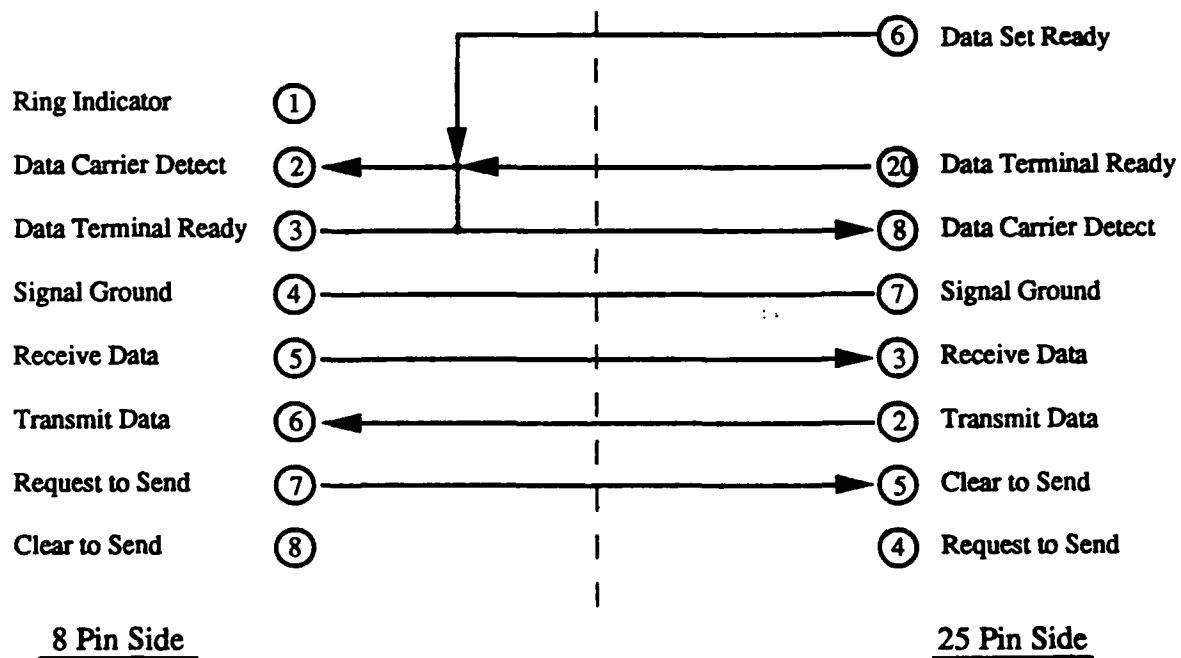
Figure B-3. RS-232-to-8-Wire adaptor wiring diagram.
