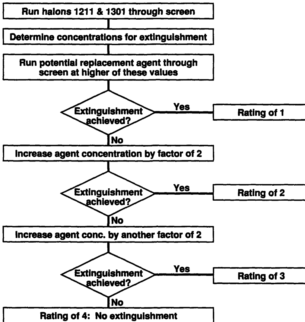
Figure 11. Candidate Agent Test Sequence
