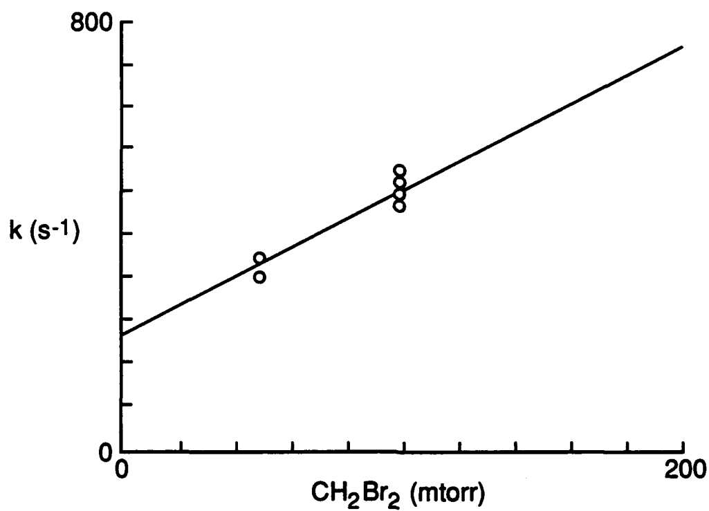
Figure A8. Plot of the First-Order Rate Constant for the Decay of OH Against the Concentration of Dibromomethane.
