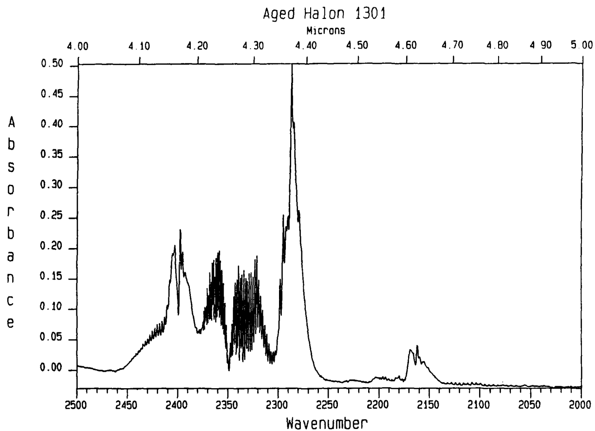
Figure 11. The Presence of CO and CO 2 are Revealed in the Expanded View of the IR Spectrum of a Sample of Halon 1301 Which was Aged at 170°C for Approximately 2 Days.
