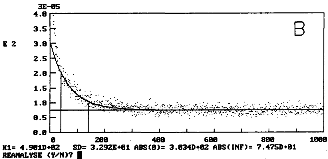
Figure A5. Decay of OH Resonance Fluorescence Signal in the Presence of Dibromomethane (halon 1002). A: 250 mtorr \text{CH}_2\text{Br}_2 . B: 500 mtorr \text{CH}_2\text{Br}_2 .
