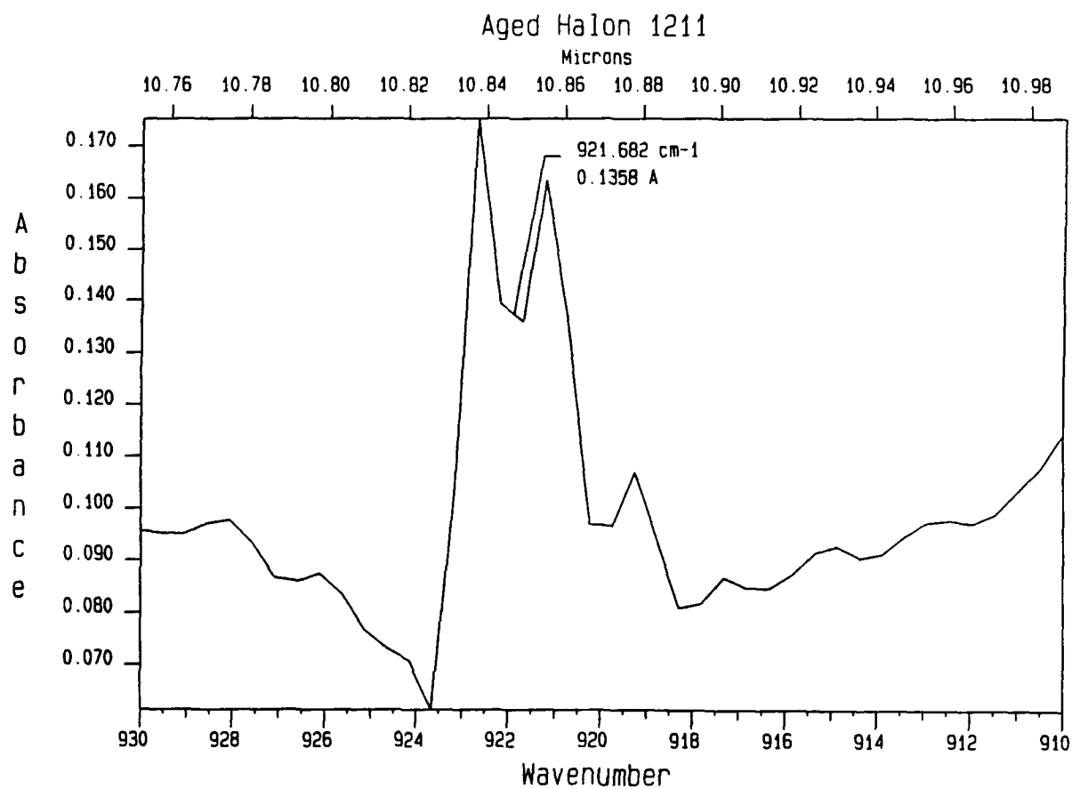
Figure 10. The Unidentified Peak in the Spectrum of Aged Halon 1211.
