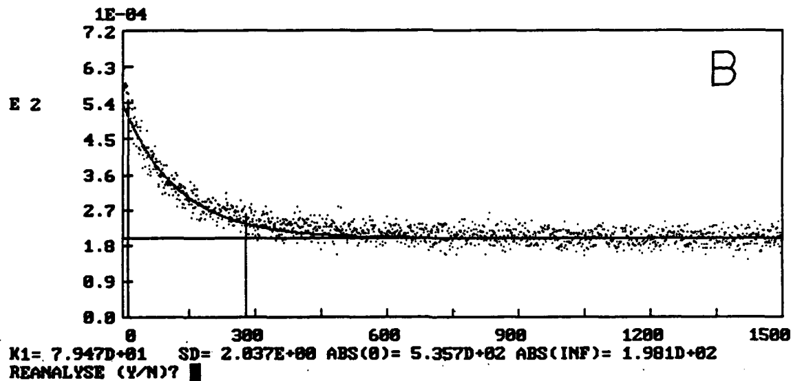
Figure A3. Decay of OH Resonance Fluorescence Signal in the Presence of Trifluorobromomethane (halon 1301). A: 2150 mtorr CF_3Br . B: 500 mtorr CF_3Br .
