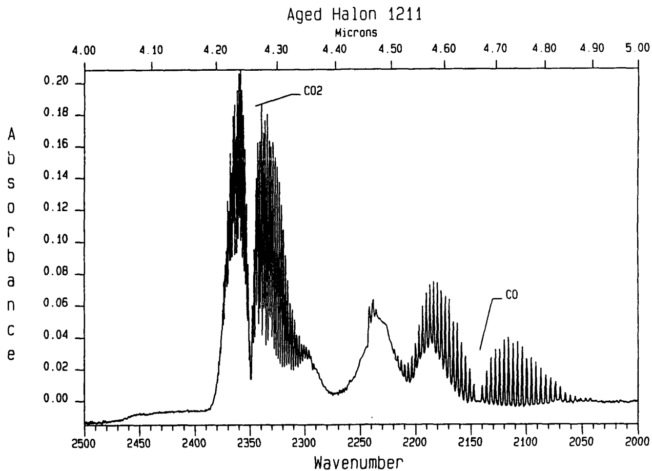
Figure 6. The Presence of CO and CO 2 are Revealed in the Expanded View of the IR Spectrum of a Sample of Halon 1211 Which was Aged at 250°C for Approximately 2 Days.
