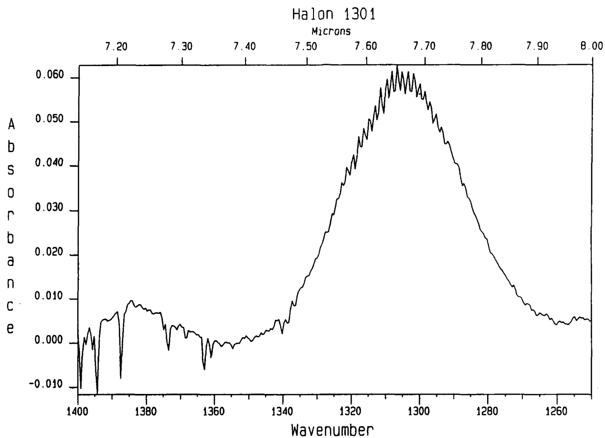
Figure 7. An Expanded View of the IR Spectrum of Halon 1301 Focusing on the Region Extending from 1400 to 1250 cm -1 .
