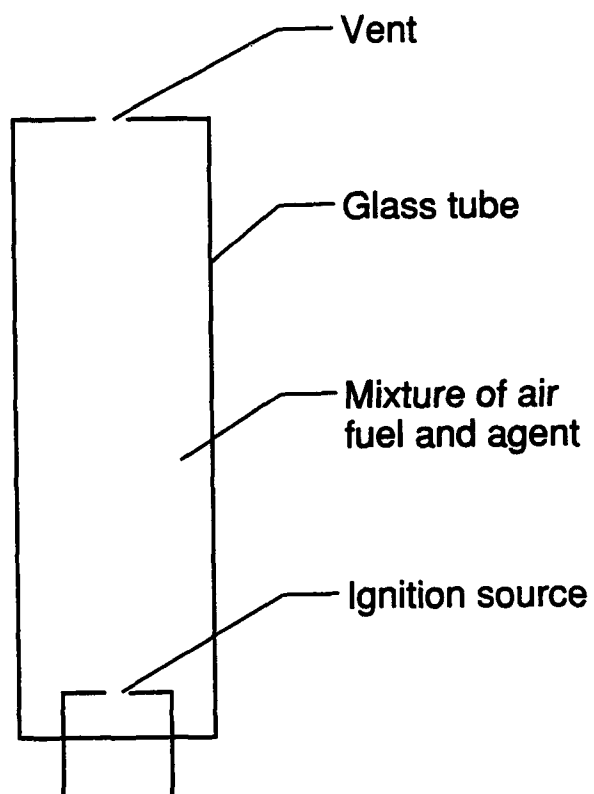
Figure 1. Explosion Burette
