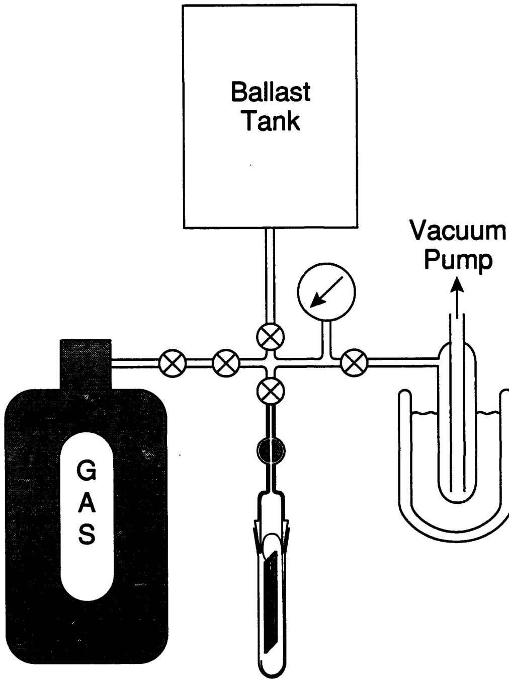
Figure 3. Piping Layout for Gas Transfer
