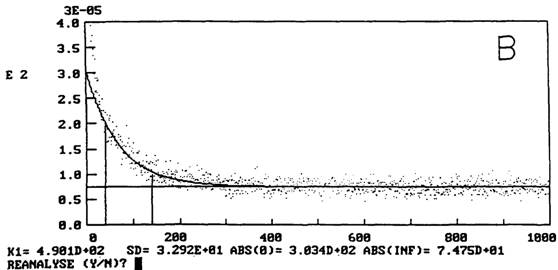
Figure A5. Decay of OH Resonance Fluorescence Signal in the Presence of Dibromomethane. A: \text{CH}_2\text{Br}_2 , 49.7 mtorr. B: \text{CH}_2\text{Br}_2 , 100 mtorr.
