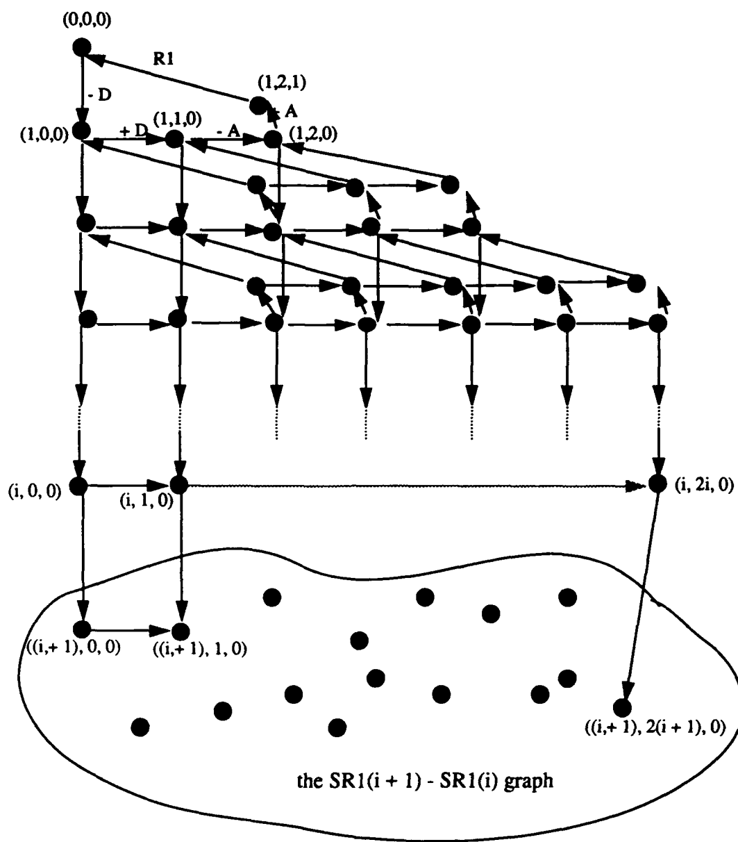
Figure 12: System State Analysis for SR1(i+1) . The lower, encircled part represents the nodes and edges not also in SR1(i) .
