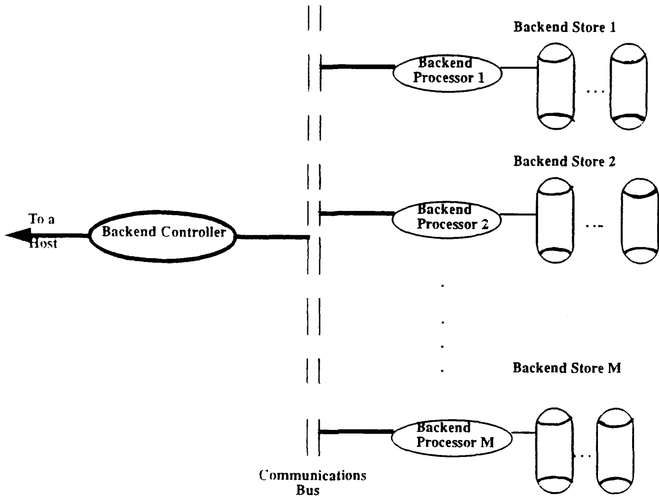
Figure 2. The Multi-Backend Database System.
