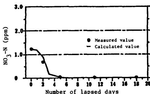
Figure 12. Concentration of \text{NO}_3\text{-N}
