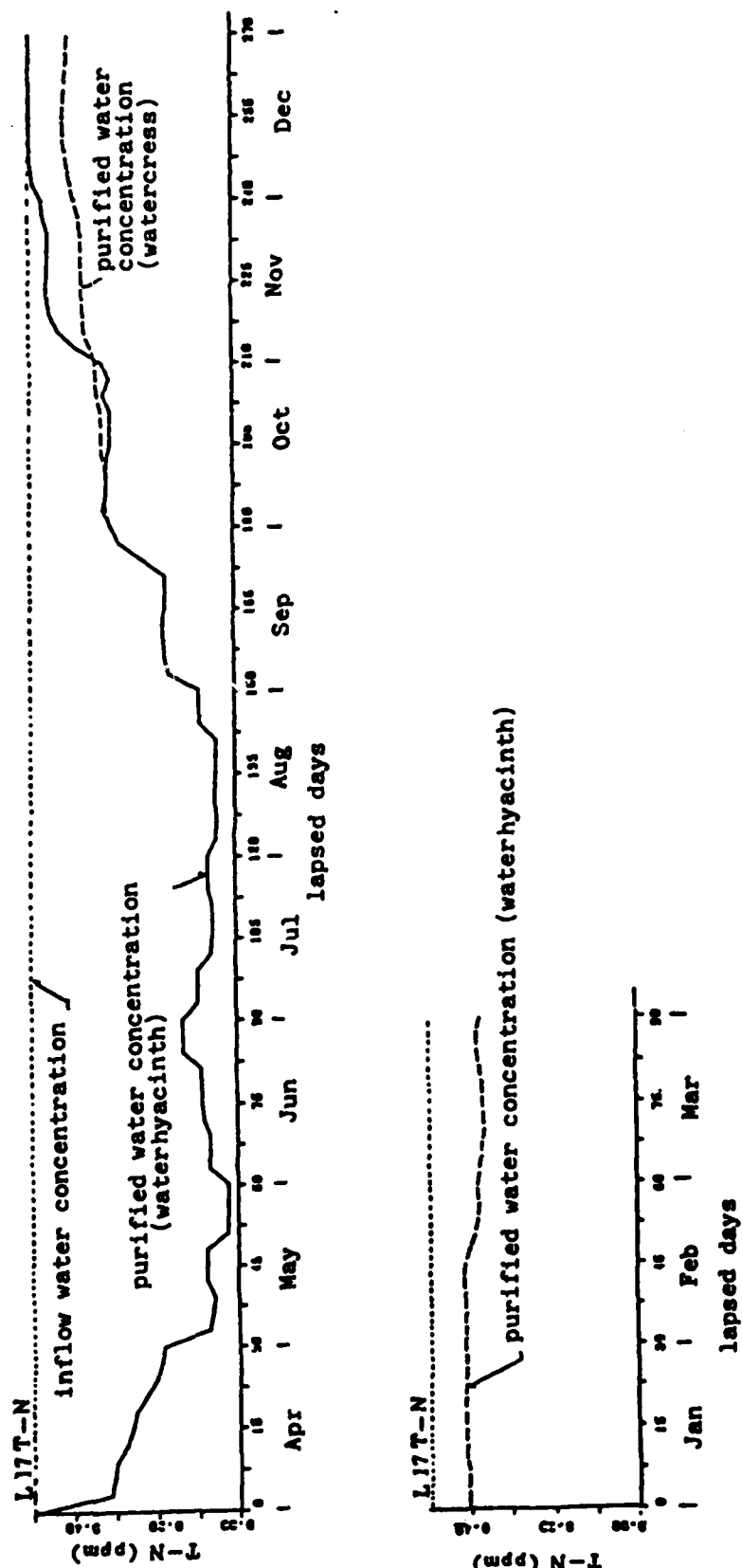
Figure 30. Calculation results for total nitrogen
