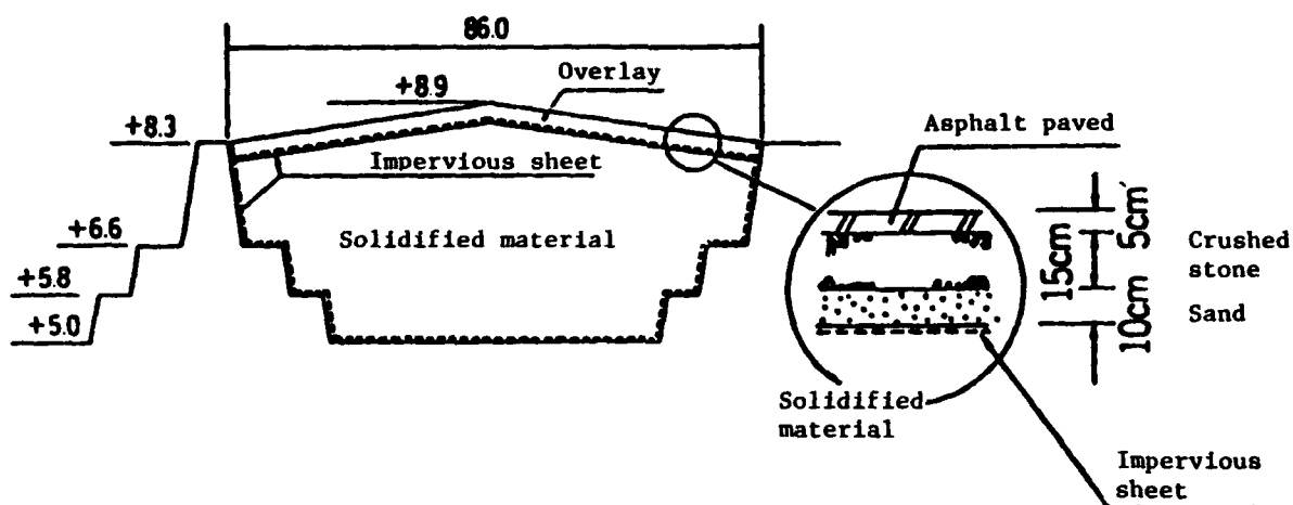
Figure 13. Cross-sectional view of final disposal area
