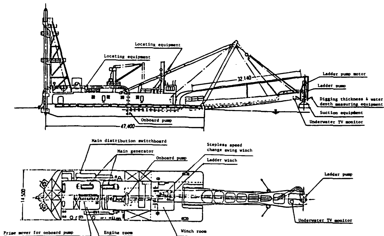
Figure 6. Pump dredge
