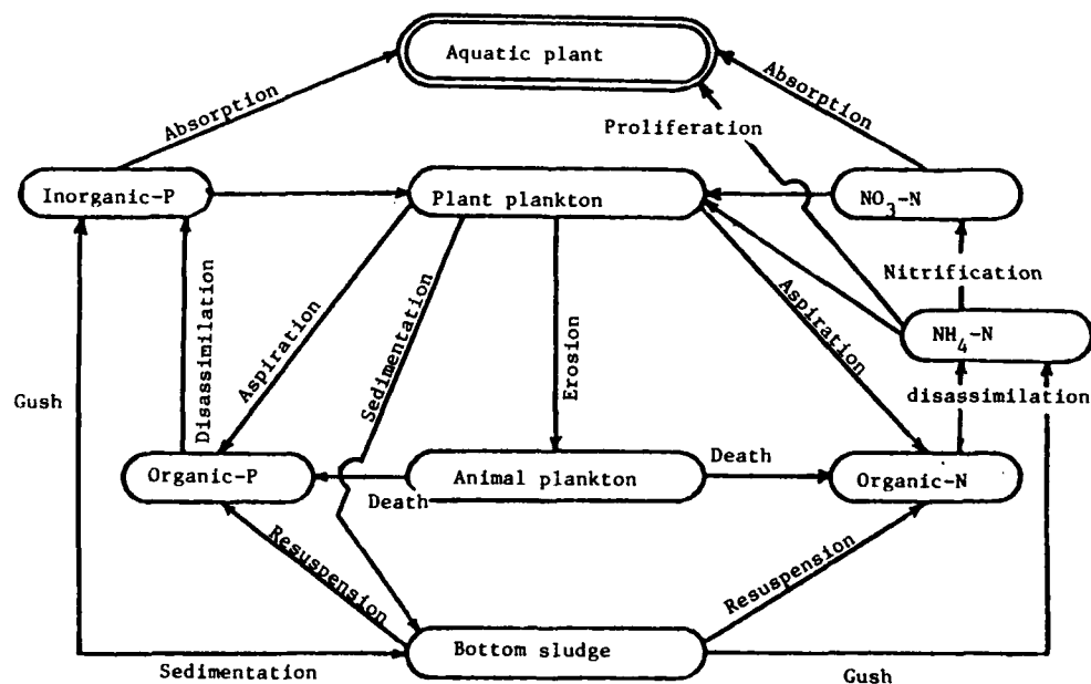
Figure 10. Organism model
