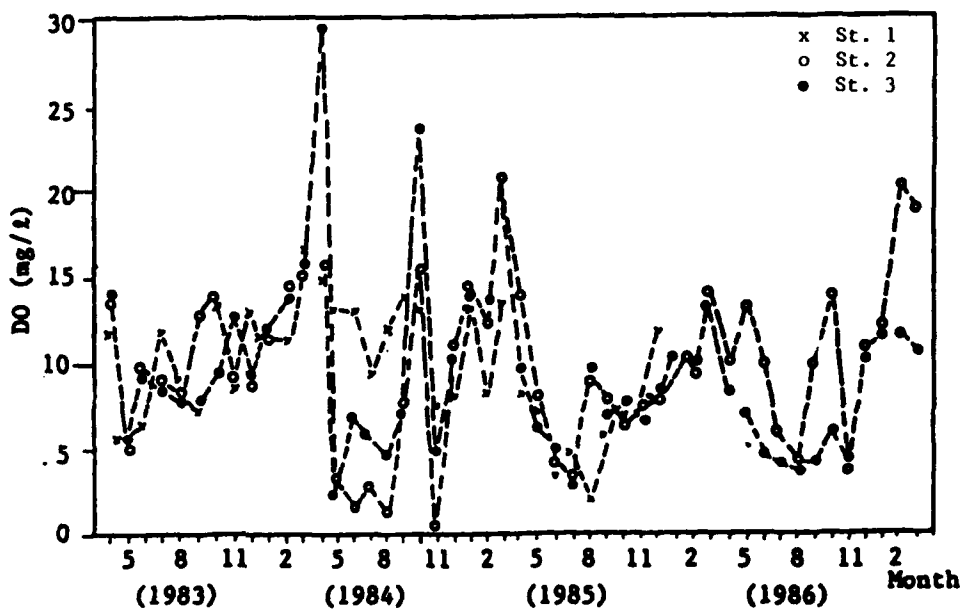
Figure 15. Monthly changes in DO
