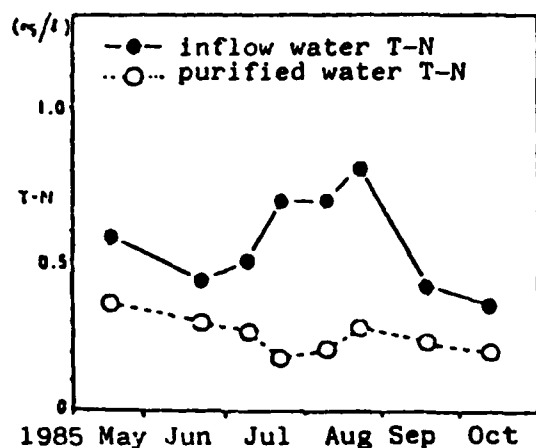
Figure 32. Water quality variation (T-N)
