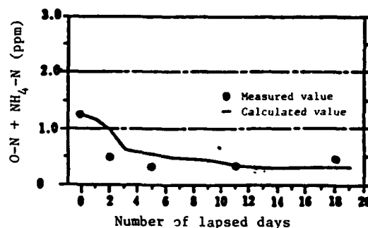
Figure 13. Concentration of organic \text{N+NH}_4\text{-N}
