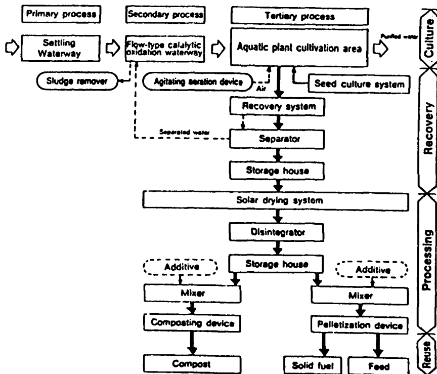
Figure 19. Test plant flowchart
