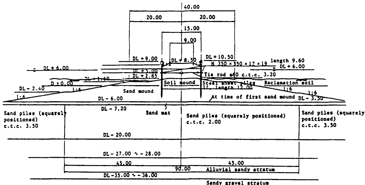
Figure 9. Cross section of partition dike 2
