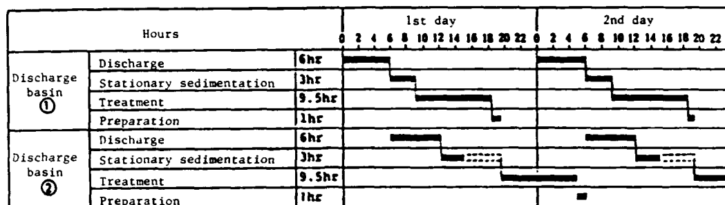
Figure 27. Residual water treatment cycle
