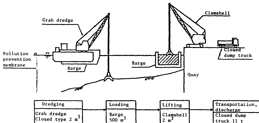
Figure 7. Grab dredging
