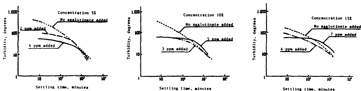
Figure 22. Turbidity of segregated water by coagulated sedimentation (direct method)
