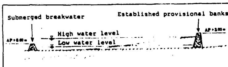
Figure 4. Section profile of the artificial beach
