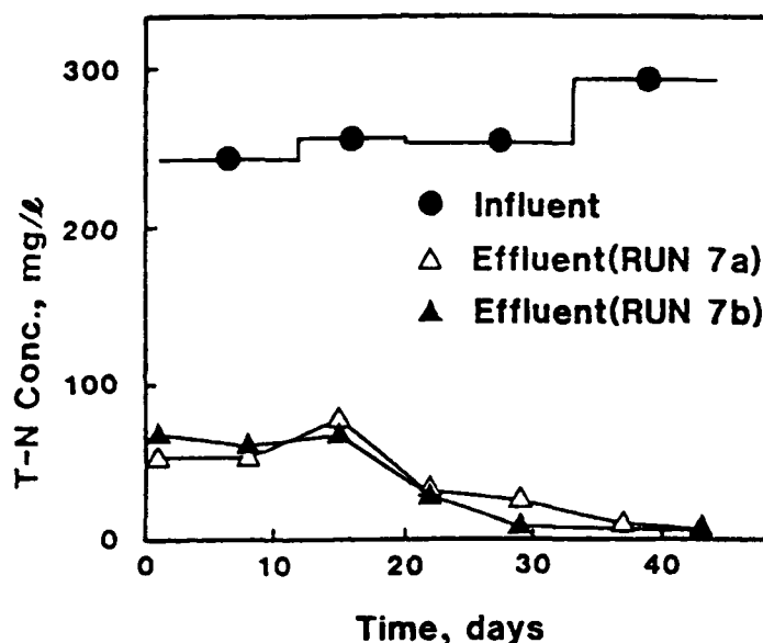
Figure 8. Concentrations of T-N in the influent and effluent in Run 7
