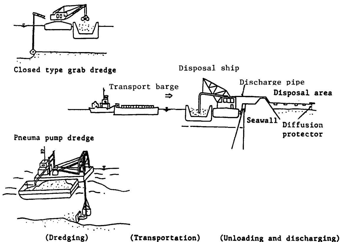
Figure 2. Organic sludge removal flowchart
