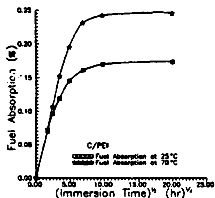
Figure 1. Fuel absorption curves for C/PEI specimens at two different temperatures.
