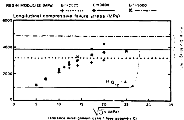
Figure 10 - Resin modulus influence.
