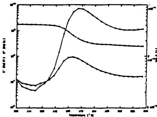
Figure 2. The dynamic mechanical spectrum of PEEK.
