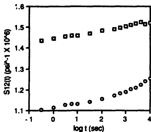
Figure 5. Creep Compliance for APC-2 \pm 45 after exposure JP-4, at room temperature.
