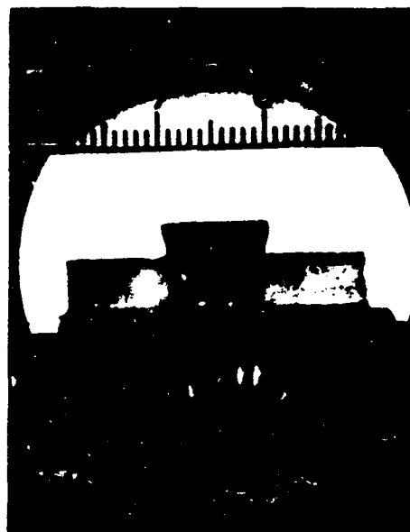
Figure 1. Brooming of Specimen Outside the ASTM D 695 Support Jig
