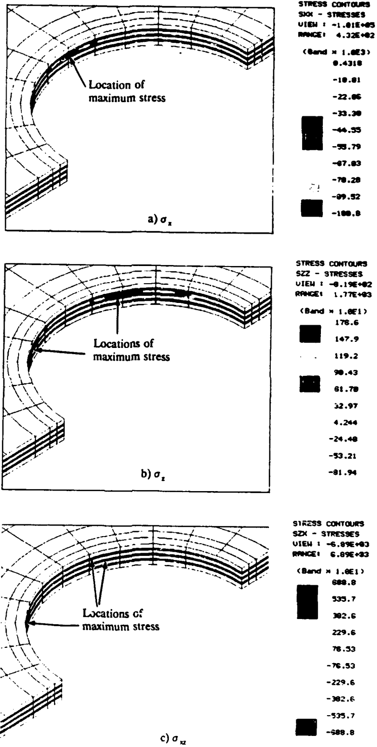
Figure 12: Finite element stress plots of the type C model.
