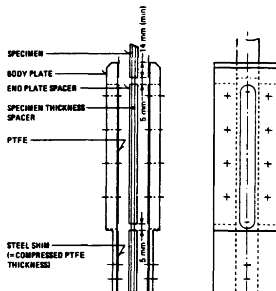
Fig. 3 Anti-buckling guide for multidirectional laminates (CRAG ref. 3)
