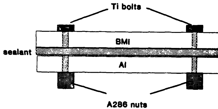
Figure 5 Salt spray exposure specimen
