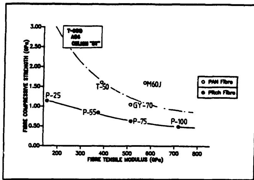
Fig 6. Comparison of fibre properties. (Reproduced from ref. 15).
