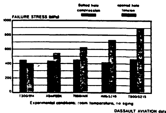
COMPRESSION & TENSION STRENGTH on a 28 plies laminate: 0,45,-45,0,90,0,45,-45,0,90,0,45,-45,0,90
