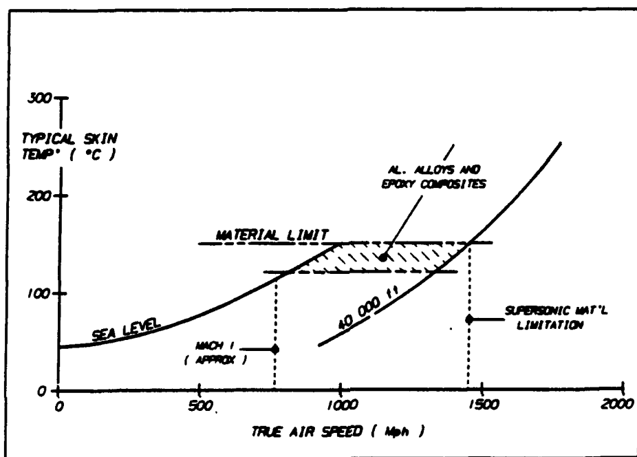
Fig 10. Skin temperature versus true air speed.
