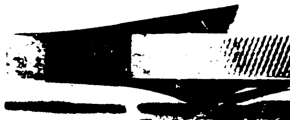
FIGURE 3. Intralaminar fracture (originating under the tab) of a 24-ply unidirectional AS4/3501-6 composite specimen tested in compression. (Specimen width: 6.35 mm)
