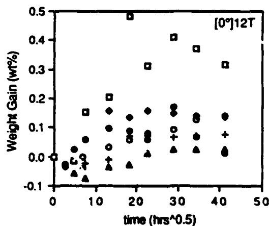
Figure 4. JP-4 weight gain for 0^\circ laminates for materials given in Table 1. Symbol meanings are as follows: open square, IM8/HTA; diamond, IM7/8551-7A; solid circle, APC-2; open circle, AS4/3501-6; cross, IM7/977-2; and triangle, IM7/5250-4.
