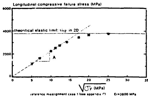
Figure 8 - \Sigma_u^c \sim A\sqrt{\sigma_y}
