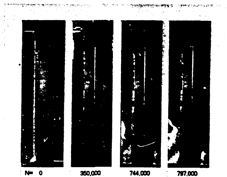
Figure 5. Laminate 2 specimen with photoelastic coating. Center of specimen is obscured by antibuckling guides. Specimen failed after 797,794 cycles so the images represent 0, 0.44, 0.94 and 0.999 life time (LT). The white area in the lower left corner of specimen seen at 0.94 and 0.999 LT indicates damaged zone.
