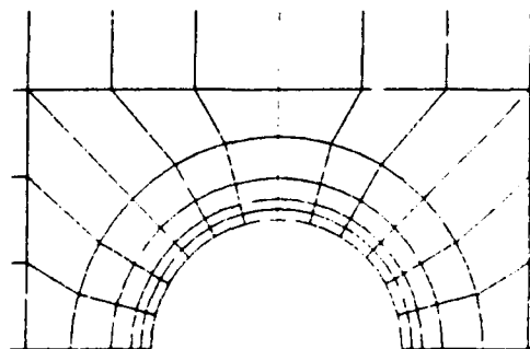
Figure 11: Finite element models
