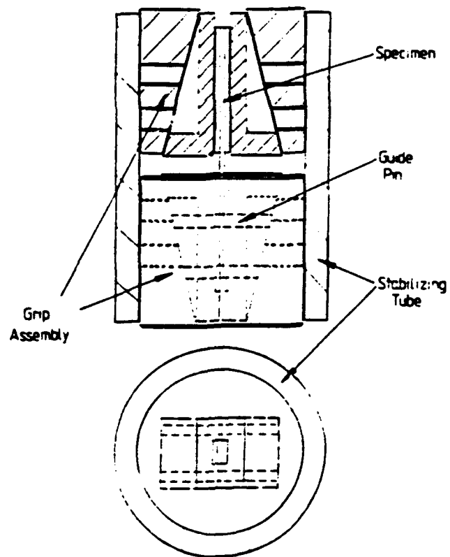
Fig 4. Modified Celanese compression rig.
