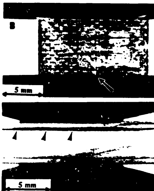
FIGURE 16. Photographs of three [0/±45/90] AS4/3501-6 sandwich specimens loaded in axial compression. (A) Edge view showing initial damage and fracture of outer 0° and 45° plies; (B) Flat view of gage section showing fracture of outer 0° ply; (C) Edge view after final failure showing separation of skin from core.
