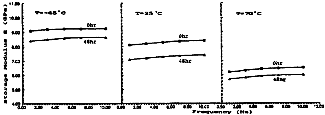
Figure 7. Storage modulus of virgin and 48 hr - immersed SIGRI CE 1007 specimens for 90^\circ fibre orientation, at three different temperatures, against frequency.
