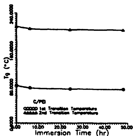
Figure 11. 1 st and 2 nd glass transition temperatures of C/PEI specimens against immersion time.
