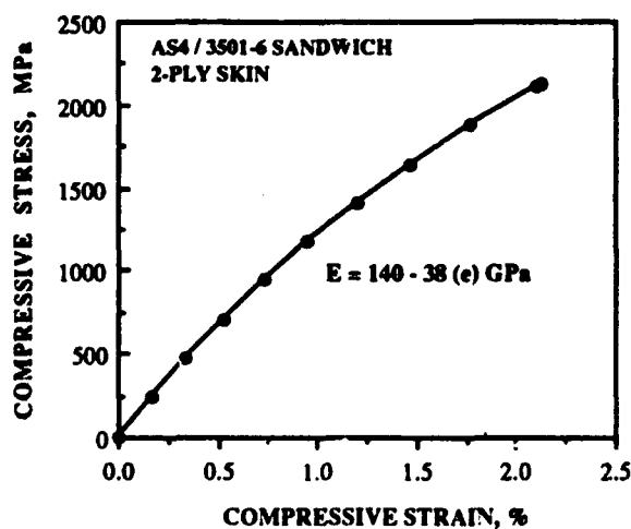
FIGURE 4. Stress-strain curve for the 2-ply composite skin of a unidirectional AS4/3501-6 sandwich specimen tested in axial compression.
