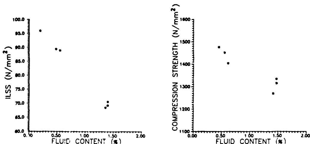
Figure-3: Variation of ILSS and compression strength values of Hercules AS-4/8552 as a function of the fluid content of the specimens.
