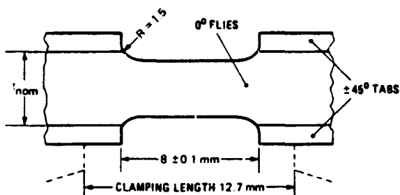
Fig. 2 Detail of DA compression specimen
