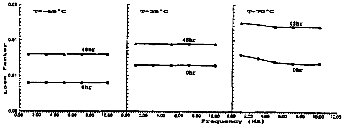
Figure 8. Loss factor of virgin and 48 hr - immersed SIGRI CE 1007 specimens for 90^\circ fibre orientation, at three different temperatures, against frequency.
