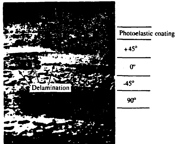
Figure 10: Photomicrograph of hole surface of type C specimen showing initial damage. Note the occurrence of the delamination within the 0° ply group.
