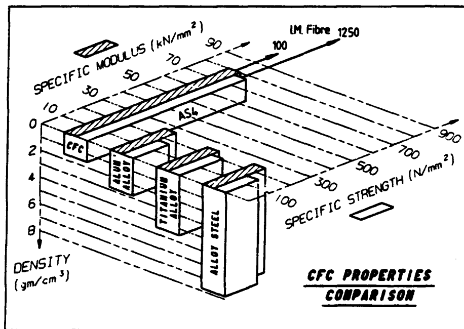
Fig 1. Properties comparison for a number of common aerospace materials. The CFC data relate to a unidirectional laminate.
