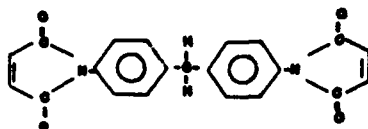
4,4' Bismaleimidediphenylmethane
