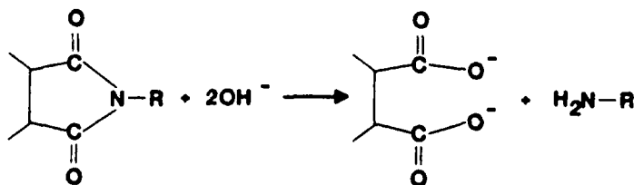
Figure 2 Imide degradation by base.
