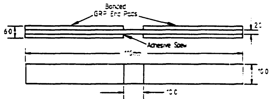
Fig 3. Compression strength test specimen.
