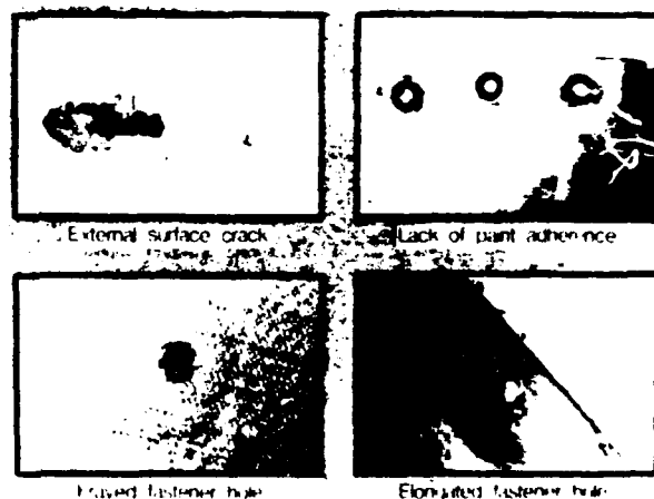
Figure 6. Typical in-service conditions of L-1011 Kevlar/epoxy fairings.
