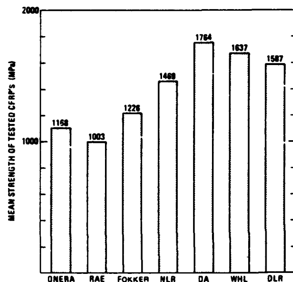
Fig. 4 Compression test performance of participating institutes and industries based on testing the same package of u.d. materials
