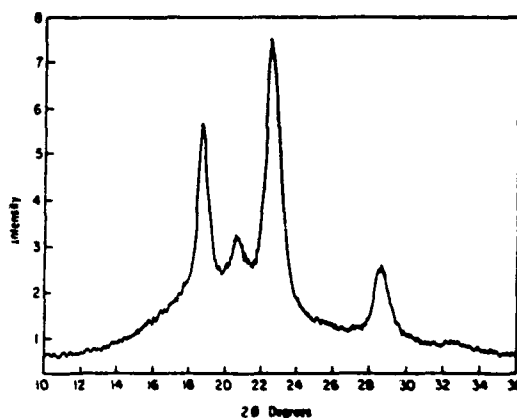
Figure 1. A typical X-ray diffraction scan of PEEK specimens.
