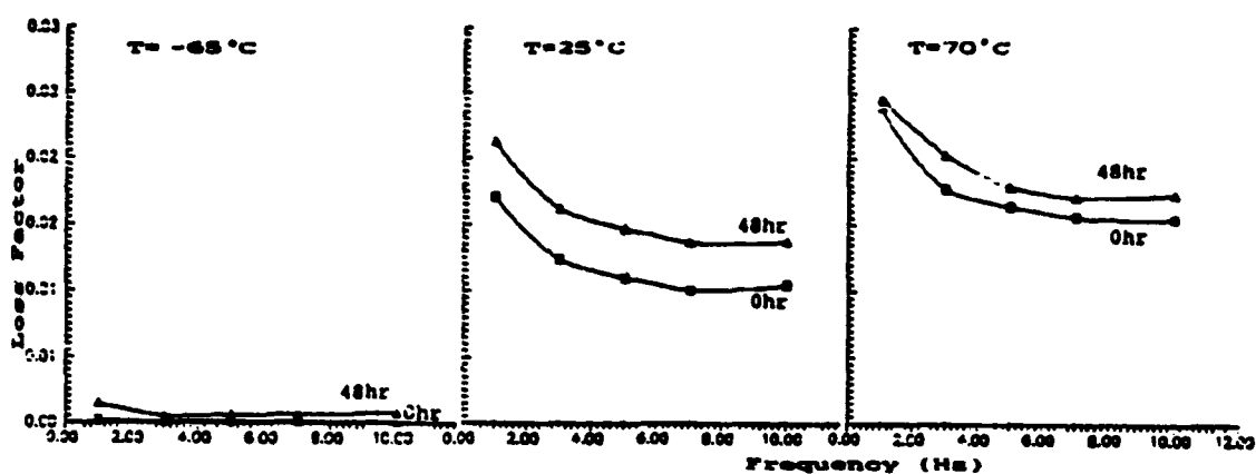
Figure 4. Loss factor of virgin and 48 hr - immersed C/PEI specimens, at three different temperatures, against frequency.
