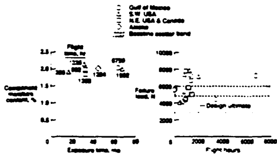
Figure 20. Moisture absorption and strength retention of Kevlar-49/F-185 Bell 206L liner doors.
