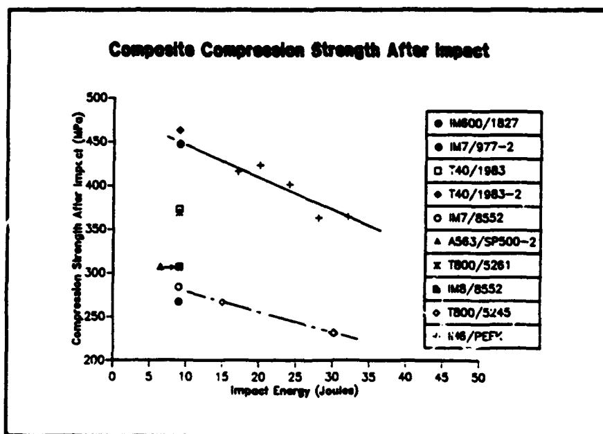
Fig 7. Compression strength after impact results for a range of composite materials. Tests based on the Boeing 7260 CAI test.
