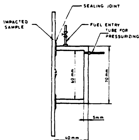
Figure-2: Pressurizing fixture for fuel leakage tests.
