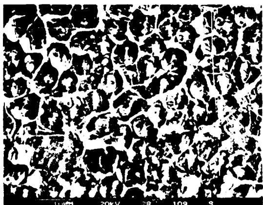
Figure 10. Fracture surface from compression area of APC2-Q(345).
