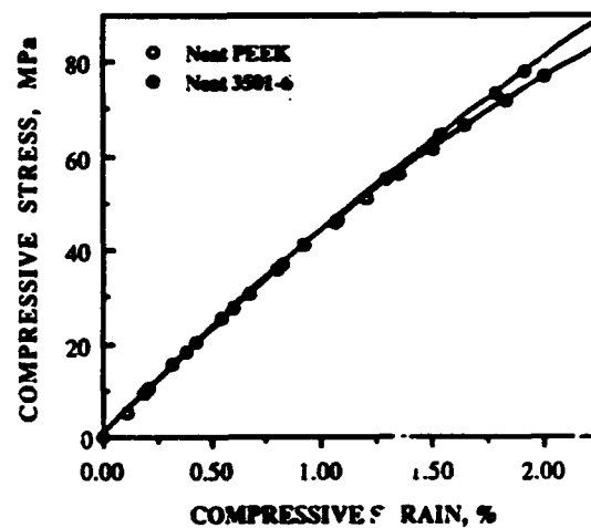
FIGURE 2. Average compressive stress-strain curves for neat PEEK and epoxy (3501-6) resins.
