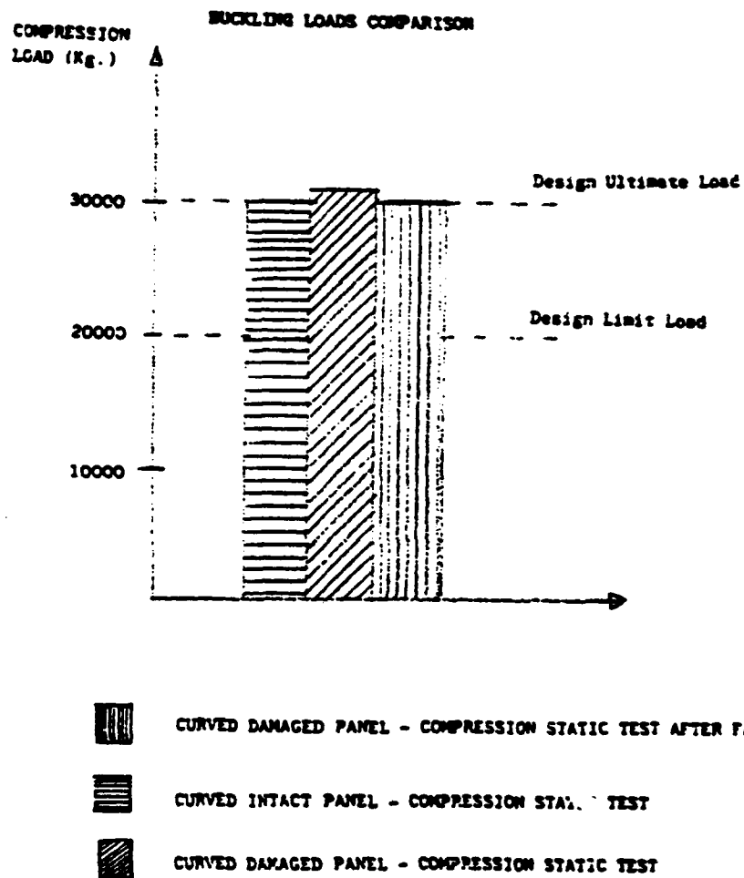
Fig.12 RESIDUAL STRENGTH AFTER FATIGUE TEST
