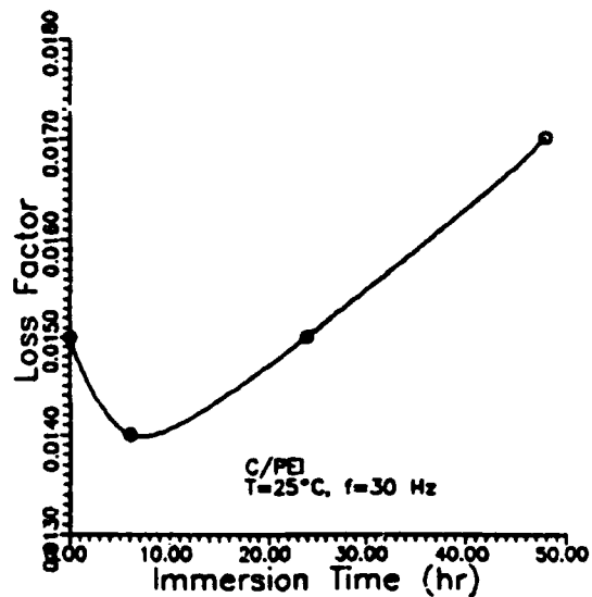
Figure 10. Loss factor of C/PEI specimens against immersion time at T = 25^\circ\text{C} and f = 30\text{ Hz} .
