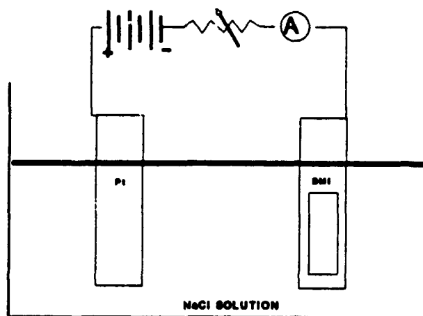
Figure 7 Electrochemical cell
