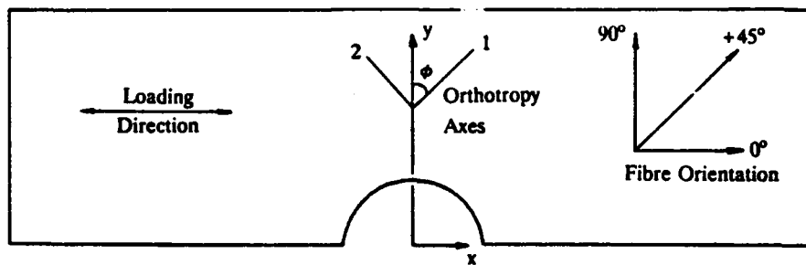
Figure 1: Fibre orientation and laminae orthotropy axes
