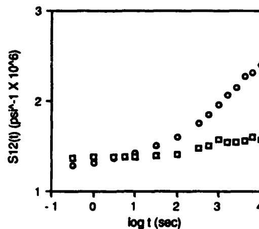
Figure 6. Creep Compliance for APC-2 \pm 45 after exposure JP-4, at 100°C.
