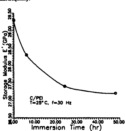
Figure 9. Storage modulus of C/PEI specimens against immersion time at T = 25^\circ\text{C} and f = 30\text{ Hz} .
