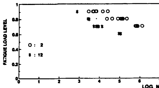
Figure 3. Laminates 2 and 12. Load level versus number of cycles to failure ( R=-3.75 , f=5\text{Hz} ).
