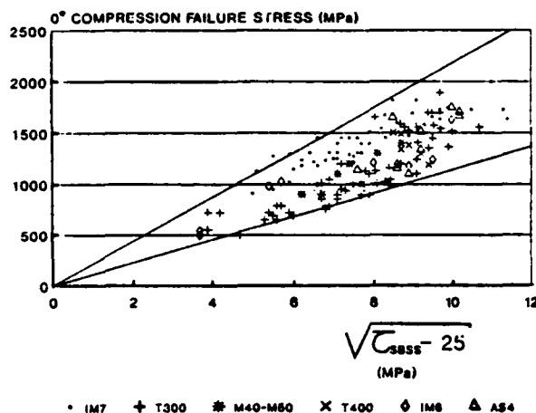
Figure 11 - Litterature experimental data report of E_n^c and \sqrt{\tau_{shear} - 25} value of various carbon/resin systems in different hot/wet conditionings.
