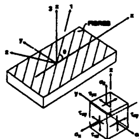
Figure 1. Reference axes and stress representation in a laminate.
