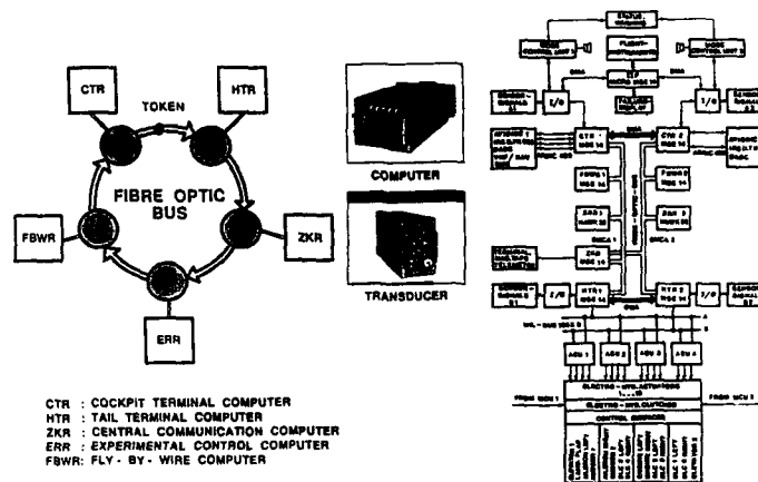
Figure 4 ATTAS Fly-by-Wire/Light Flight Control System
