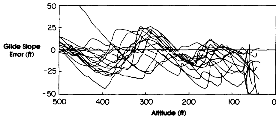
Figure 10 C3 Glide Slope Error vs. Altitude (Reference 9).
