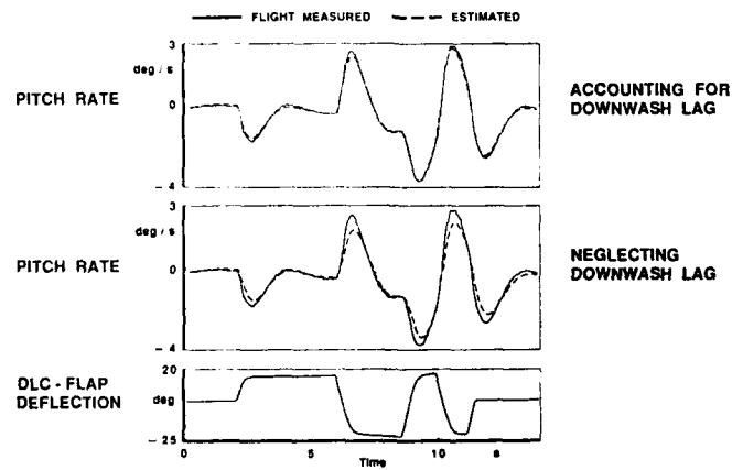
Figure 9 Downwash modelling, [9]
