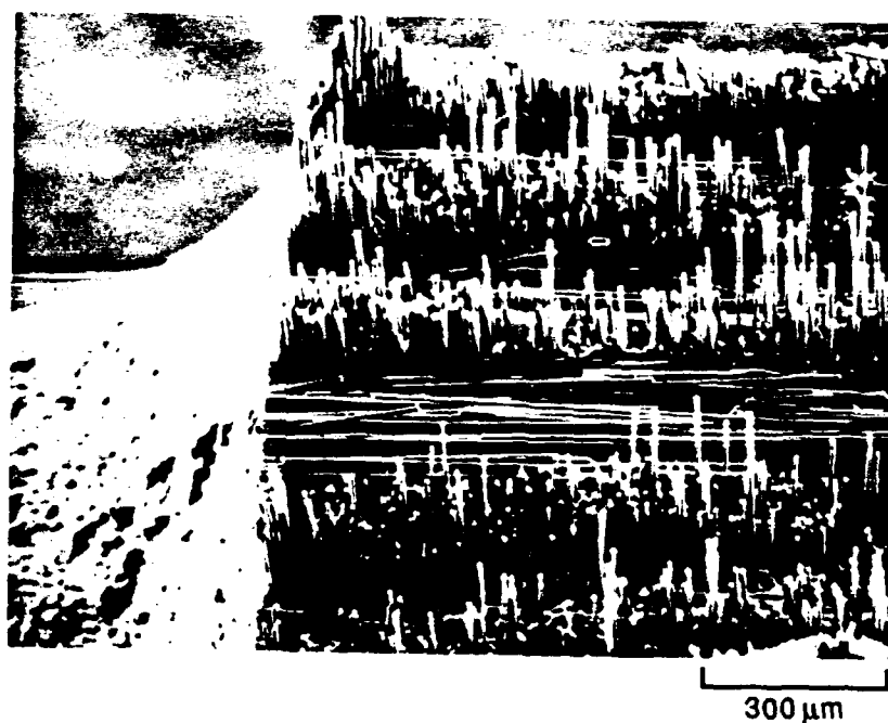
Figure 11-14. (a) Tensile Strength of [0/90] FT700/BSG Composites Containing Circular Holes of Various Diameters. (b) Fracture Surface in the Vicinity of the Notch for a [0/90] FT700/BSG Composite.
