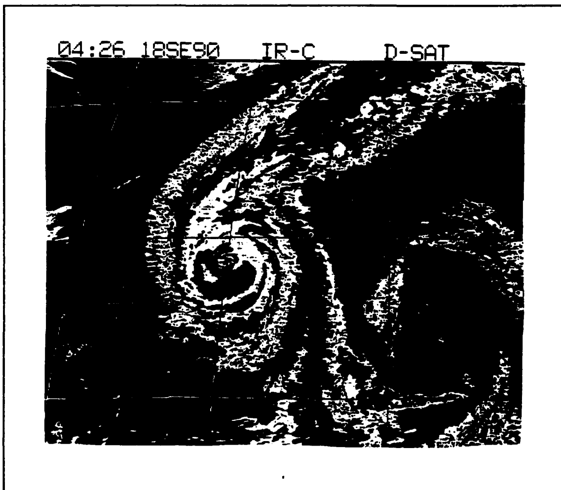
Figure 14. IR satellite imagery of the Supertyphoon Flo on 18 September 1990.
