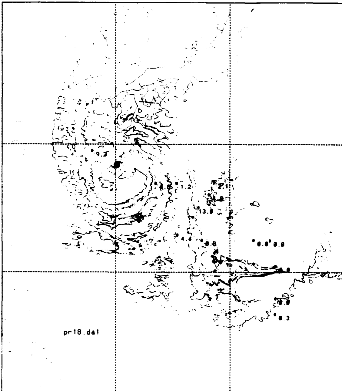
Figure 13. Predicted precipitation rate (mm/day) for the soundings of 18 September 1990.
