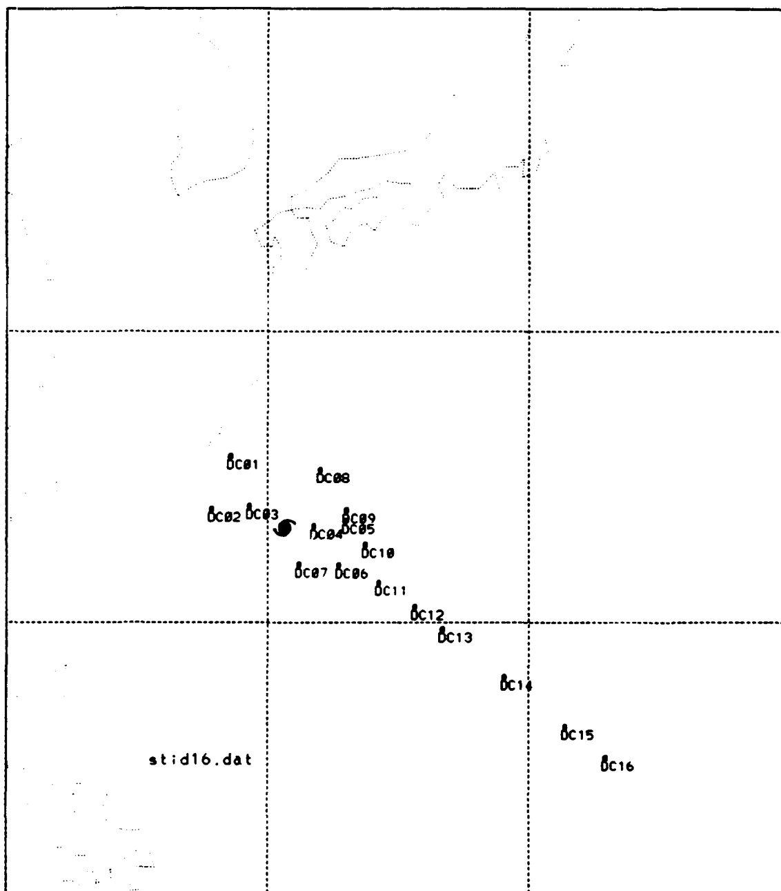
Figure 4a. Positions of dropwindsondes relative to the center of the Supertyphoon Flo on 06 UTC 16 September 1990.
