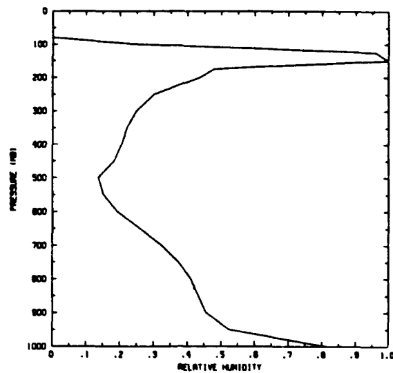
Figure 7a. Relative humidity averaged over the last 100 hours of model run, except for \sigma=10^{-3} value (Emanuel 1991).
