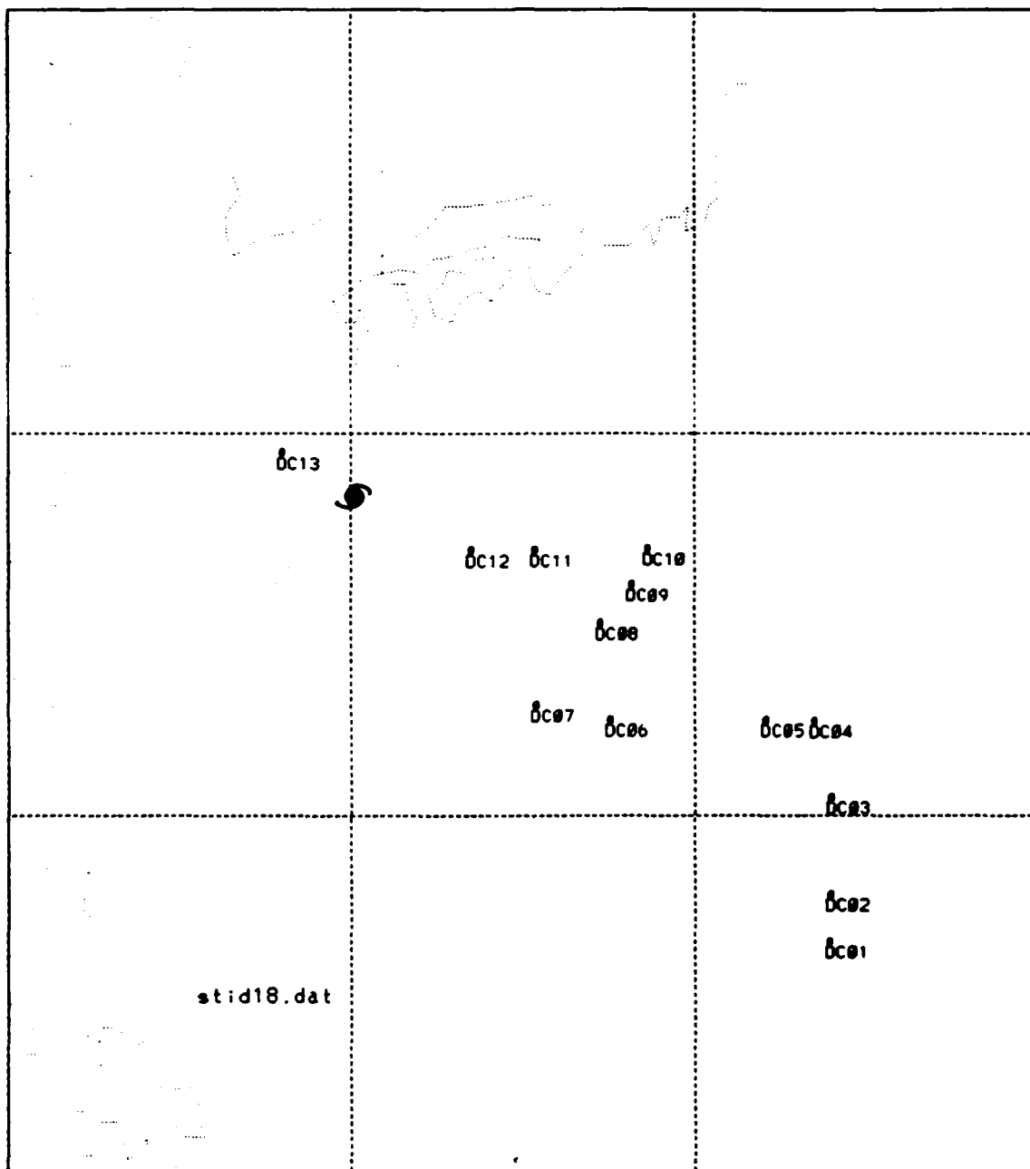
Figure 4c. As in Fig. 4a, except for 06 UTC 18 September 1990.
