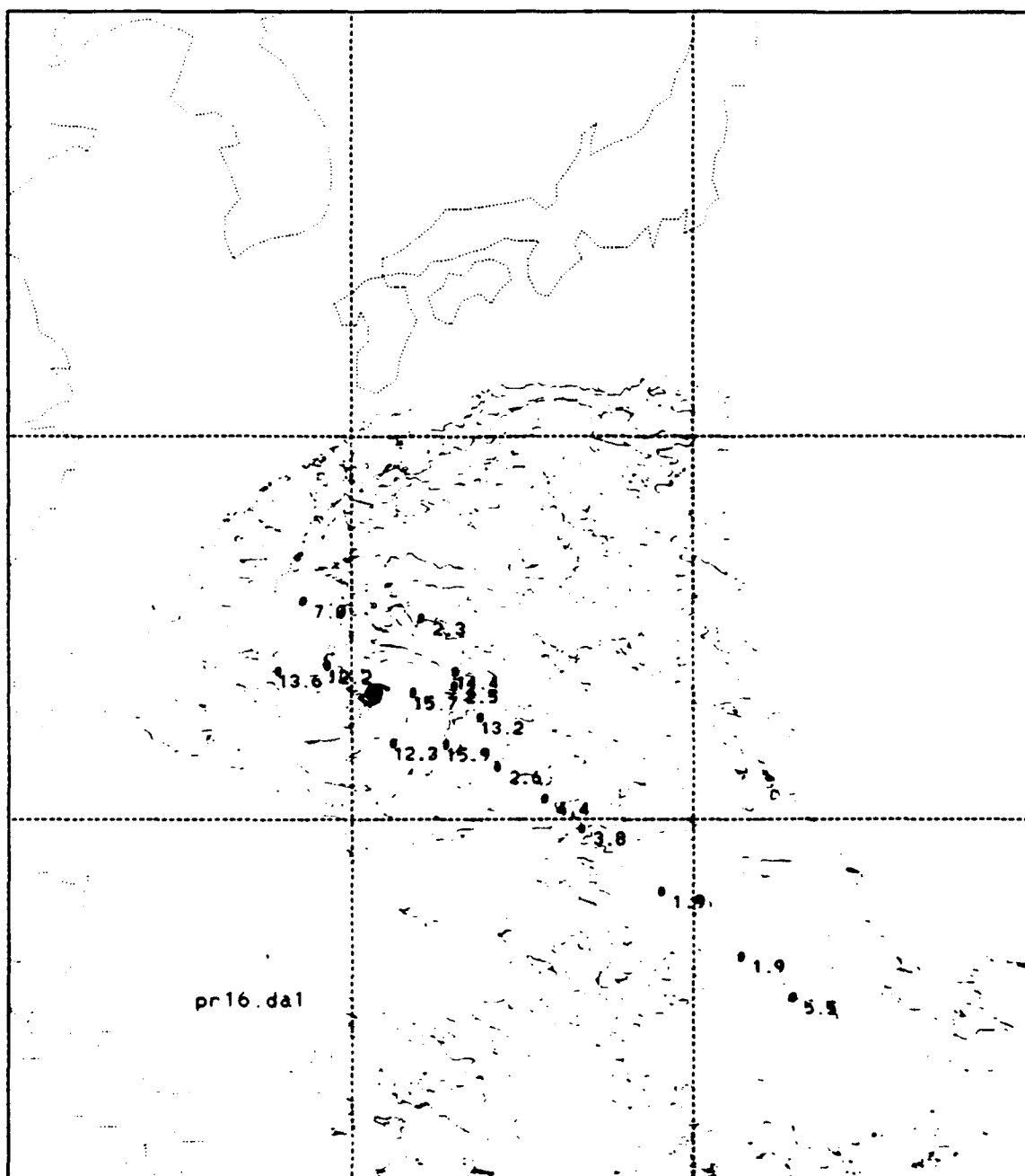
Figure 9. Predicted precipitation rate (mm/day) for the soundings of 16 September 1990.
