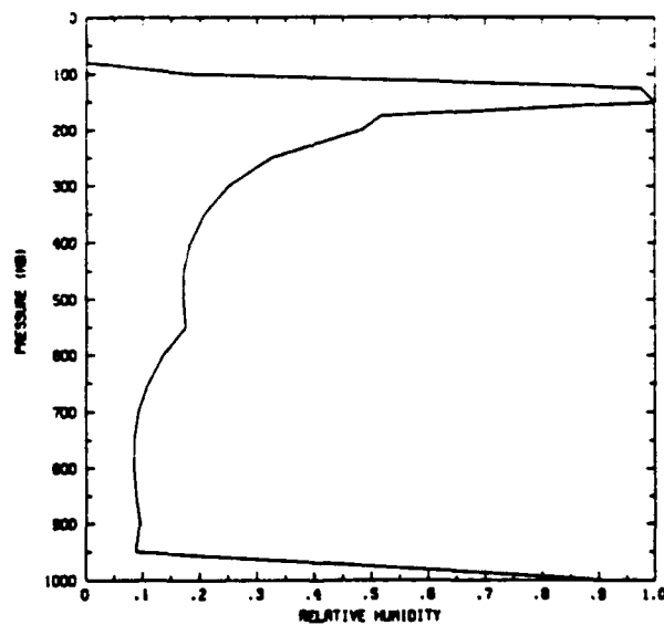
Figure 7b. Relative humidity averaged over the last 100 hours of an equilibrium experiment in which \epsilon^l=1 throughout, with \sigma_z^l=0 except below cloud base (Emanuel 1991).
