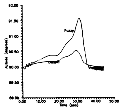
FIGURE 29 - HARDWARE MODEL
