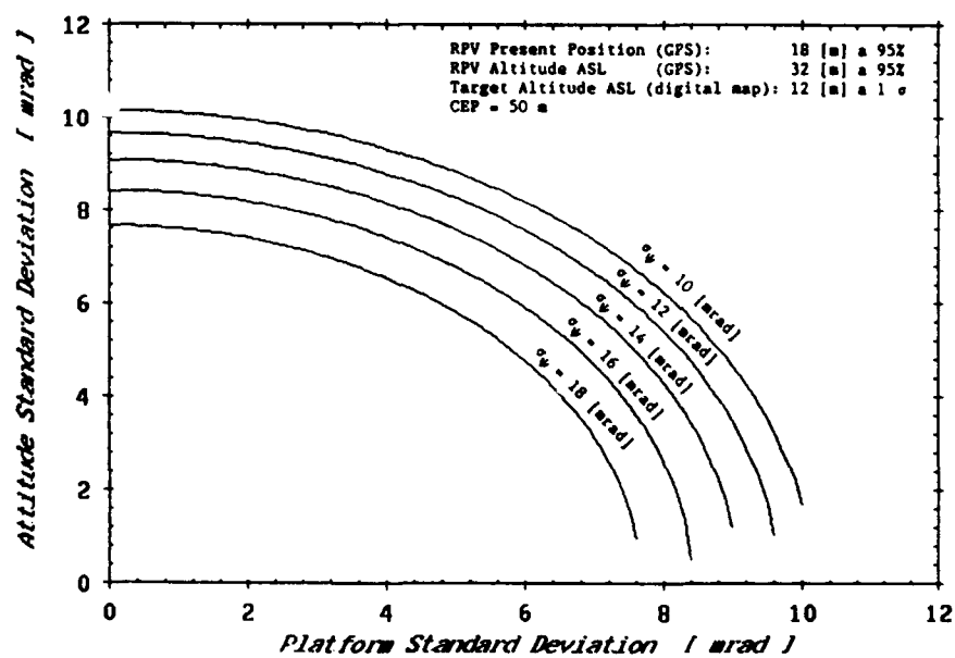
- Figure 9 : \sigma_{ATT} vs \sigma_{PLT} for different \sigma_p -
