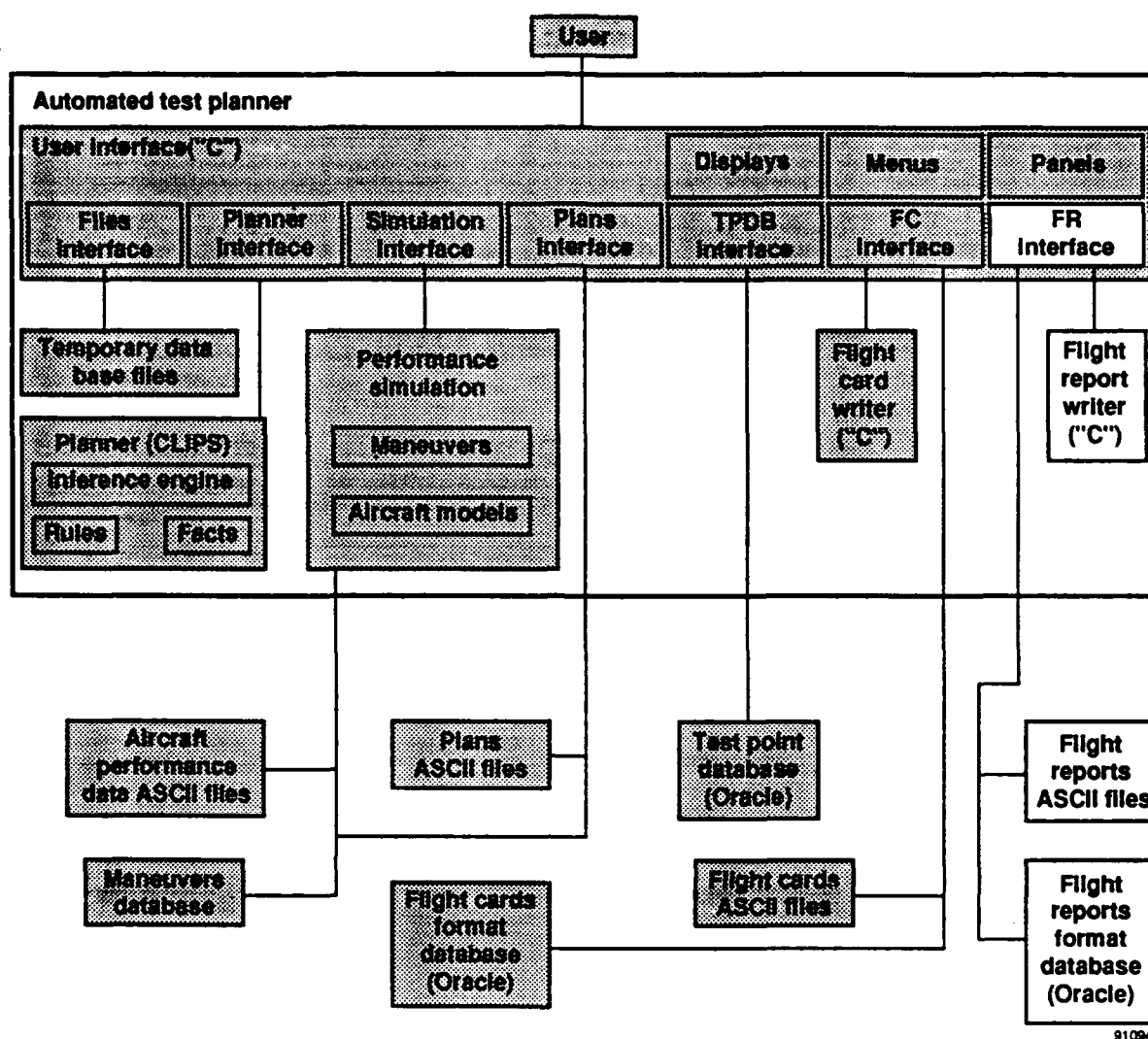
Fig. 8 TEST_PLAN system architecture.
