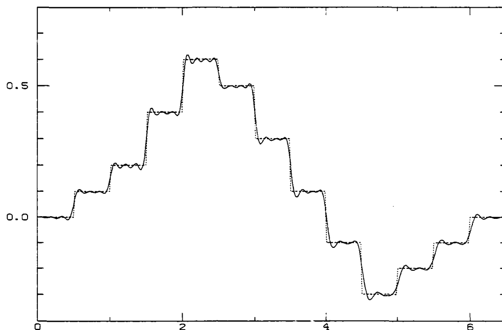
Figure 6.9: Reconstruction of Example 4.2 with a = 20
