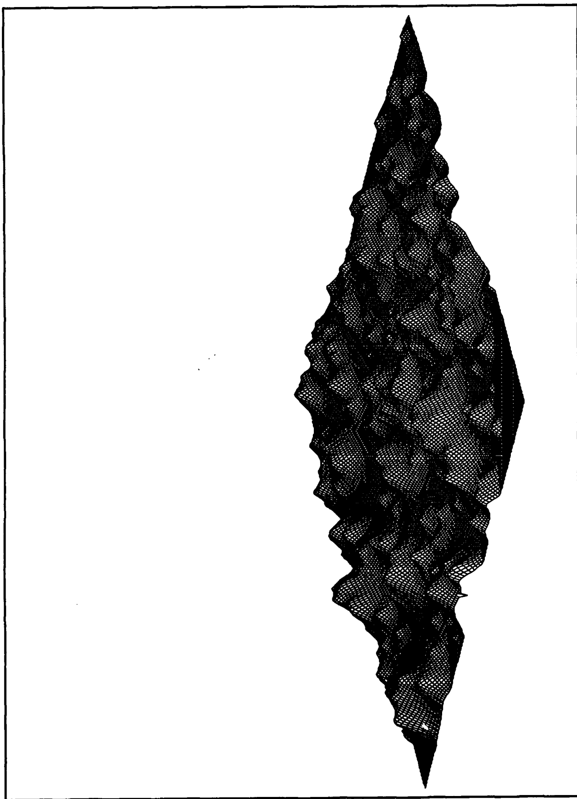
Figure 6. Self-similar Mountains.
