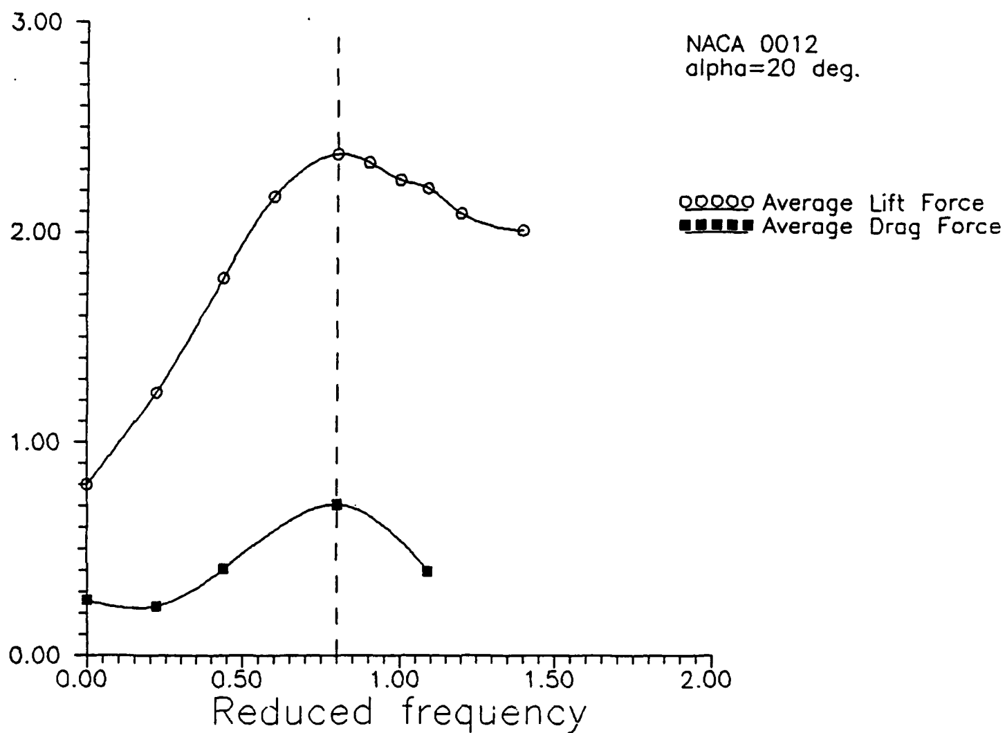
Figure 17: Variation of time-averaged drag force ( \overline{D} / \frac{1}{2} \rho S U_\infty^2 ) and lift force ( \overline{L} / \frac{1}{2} \rho S U_\infty^2 ) as a function of reduced frequency ( \alpha = 20^\circ , R = 0.59 ).
