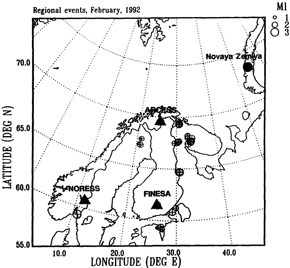
FIG. 3. Epicenters of regional events causing the network threshold to exceed m_s = 2.6 . All events, except one felt earthquake in southern Norway are probable mining explosions. Note the large number of events on the Kola peninsula.
