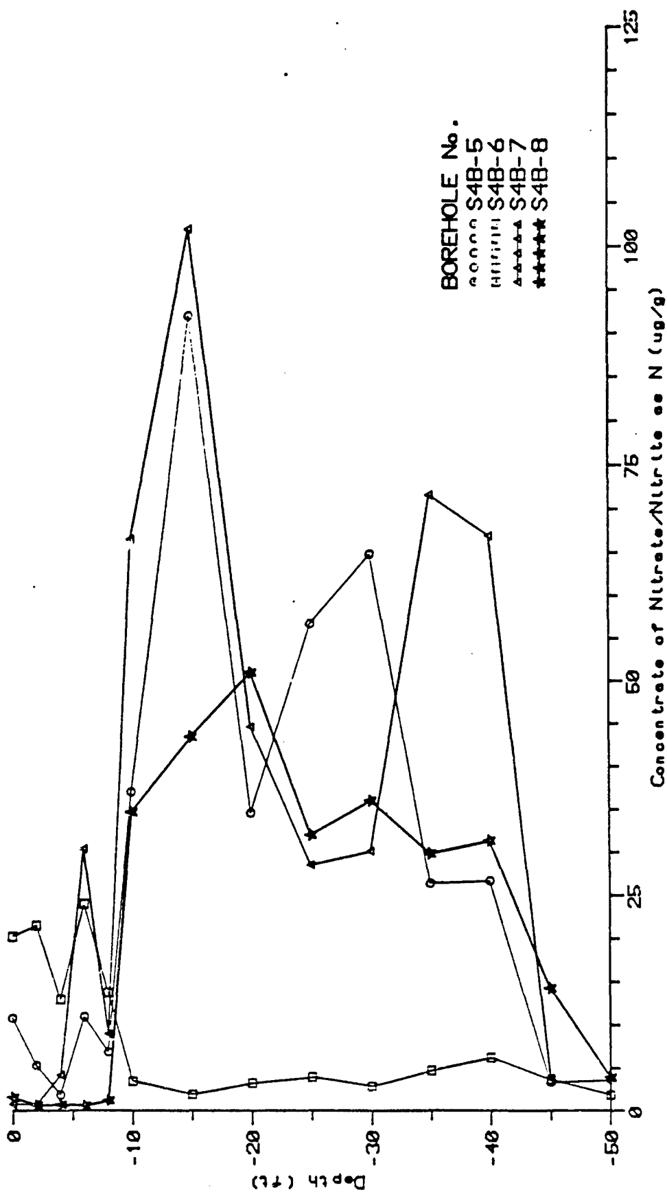
Figure D-8 Depth vs Concentration of Nitrate/Nitrite in Explosive Washout Lagoons
