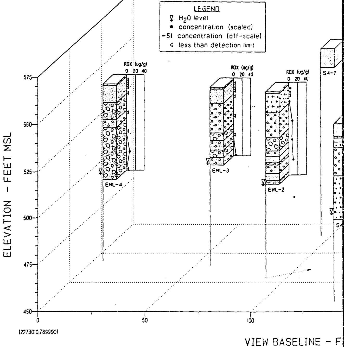
Figure E-5 - Lithologic Profile S
