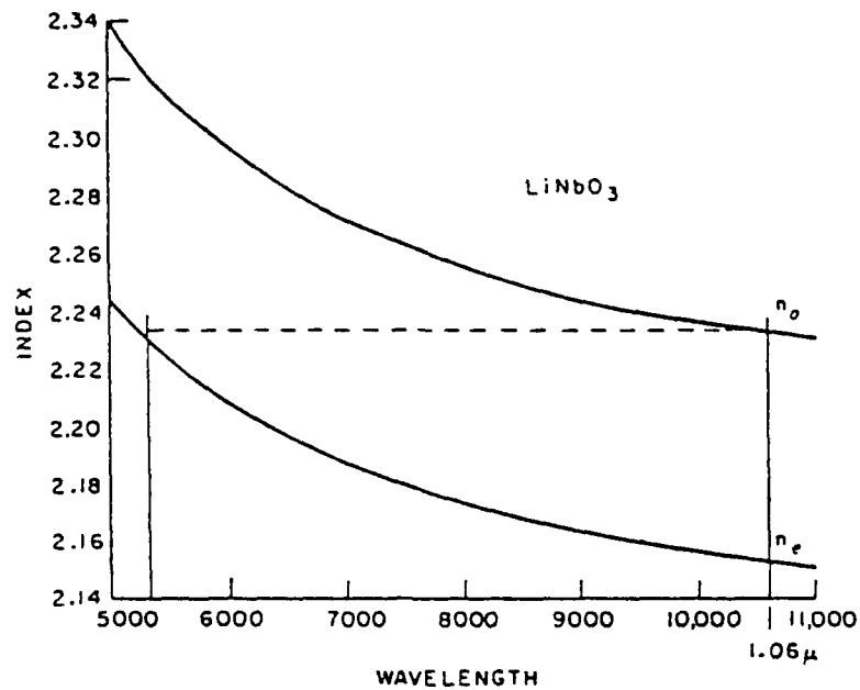
Figure 3. Dispersion curves for LiNbO showing SHG of Nd:YAG laser with noncritical phase matching (ref. 3).
