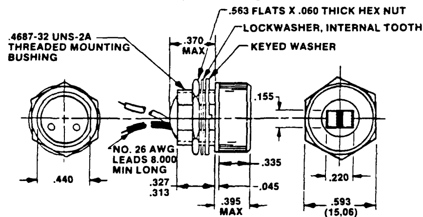
WIRE LEADS
