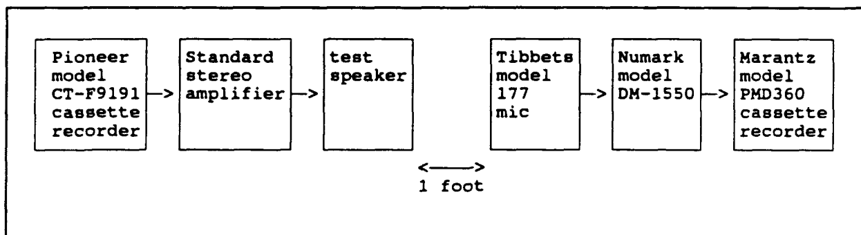
Figure 2. Configuration for the Speaker Evaluation
