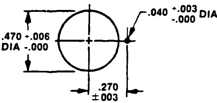
OPTIONAL PANEL LAYOUT USING KEYED WASHER
