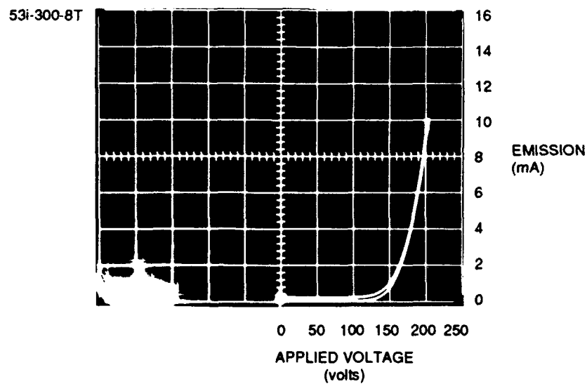
Figure 1. Current/voltage curves for cathodes 53i-300-8Q and 53i-300-8T at the time of shutdown after 1850 hours of operation
