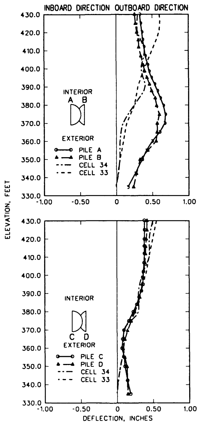
Figure 7.4: Movements of inboard and outboard walls after berm placement.
