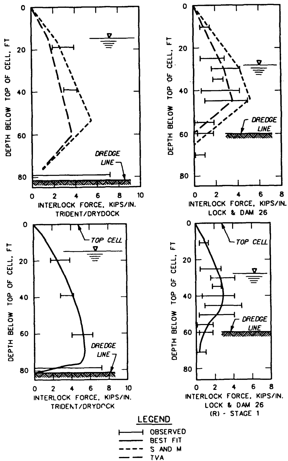
Figure 2.15: Measured interlock forces for Trident and Lock and Dam No. 26 (R) cofferdams.
