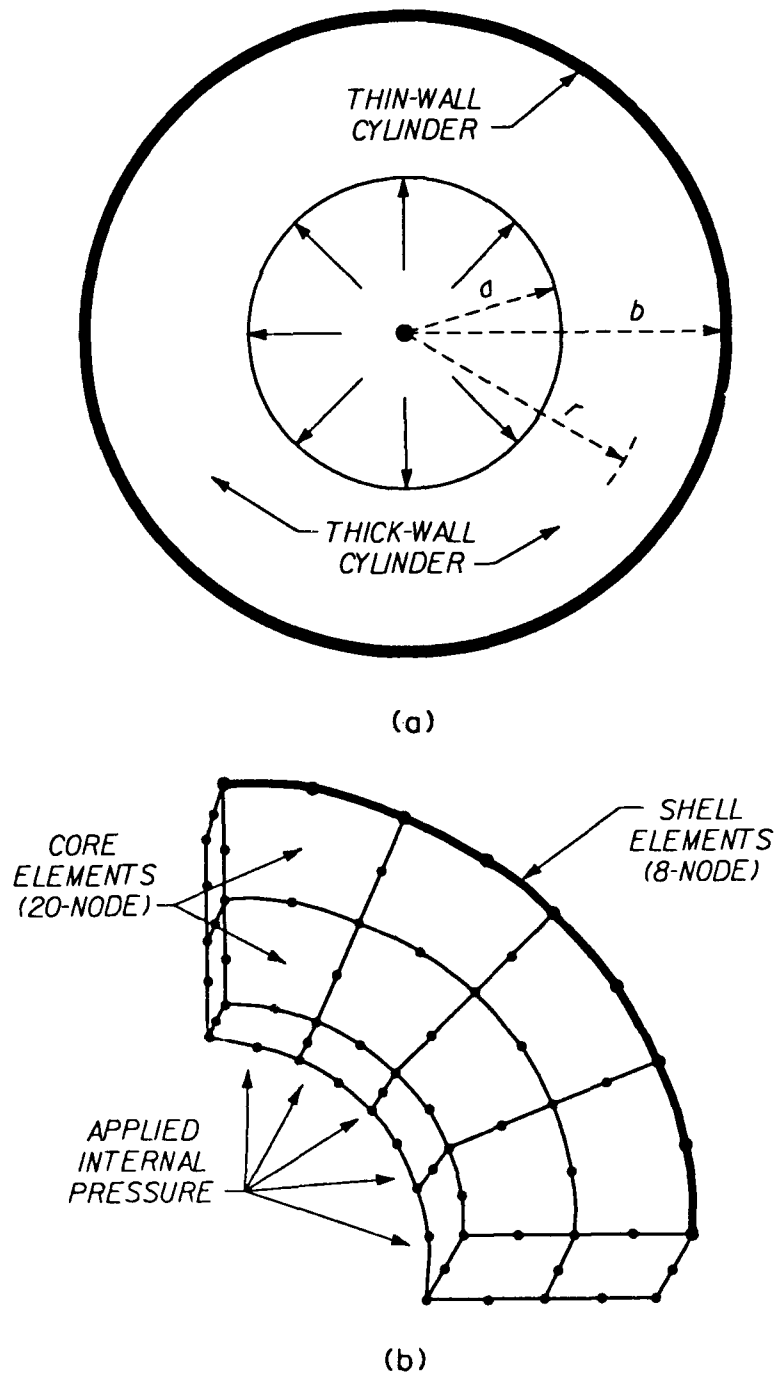
Figure 4.14: Composite, thick-wall cylinder problem: a. composite, thick-wall cylinder with an internal surface pressure; and b. finite element mesh for the composite-wall cylinder.
