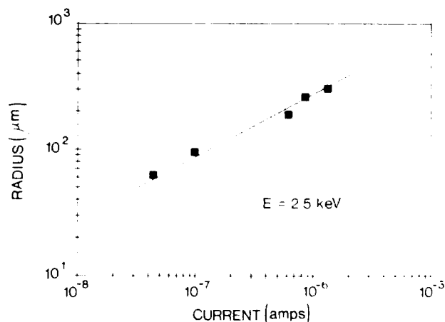
FIG. 5. Beam radius vs beam current for the high-energy cesium ion gun at a beam energy of 2.5 keV. The squares are experimental data, and the line represents Eq. (4) in the text.
