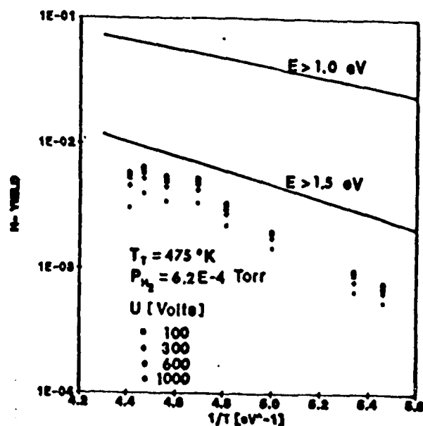
Fig. 5. Negative Hydrogen Ion Yield vs. 1/T(\text{oven}) at several extraction voltages. Chamber pressure = 6.2 \text{ E-}4 torr.
