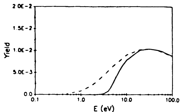
FIG. 2. H^- yield as a function of incident energy on a bare tungsten surface. Solid line: variable velocity; Dotted line: constant velocity.
