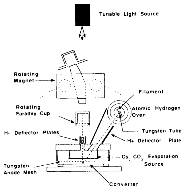
Fig. 1. Experimental apparatus.
